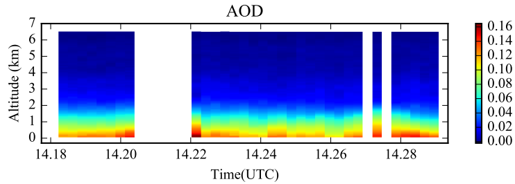
Figure 4. The cumulative aerosol optical depth (AOD) at 532nm from HSRL, which is the AOD of the layer from the aircraft to the altitude as indicated in the plot, for the open water case in 07/27/2014. The white stripes indicate no HSRL retrieval due to the presence of cloud.
