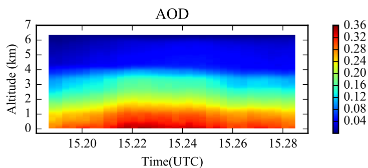
Figure 8. The cumulative aerosol optical depth (AOD) from HSRL. Same as Fig. 4 but for coastal water case in 07/30/2014.
