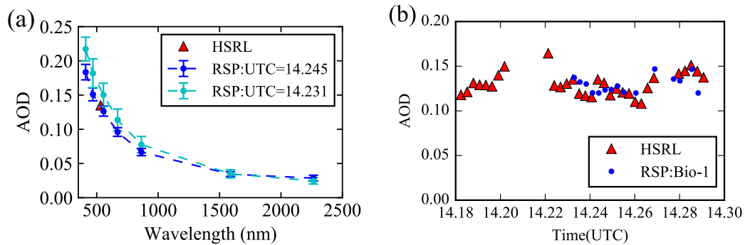
Figure 5. (a) The retrieved aerosol optical depth (AOD) from RSP measurement at UTC=14.231 (SABOR-Open) and 14.245 comparing with HSRL AOD at 532nm similar at both time. The error bars indicate the retrieval uncertainties. The retrieval algorithm is based on the [Chla]-based bio-optical model (Bio-1). (b) The comparison of the RSP retrieved AOD at 550nm with the HSRL AOD product across the flight track.
