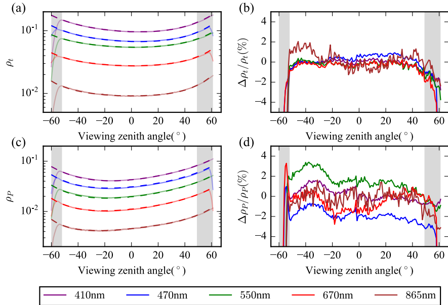
Figure 13. Same as Figure 3 but for NAAMES-Coastal on 11/04/2015. The minimum cost function value is \chi_{min}^2 = 0.16 and the bio-optical model used here is Bio-2.
