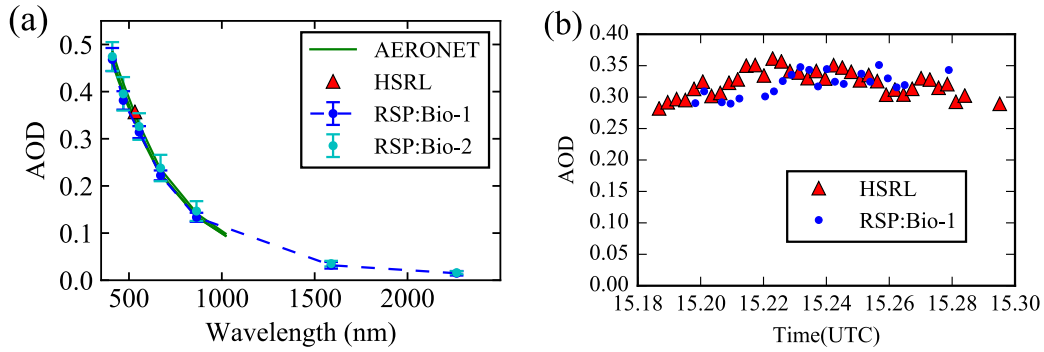
Figure 9. (a) The comparison of the RSP retrieved AOD, the HSRL HSRL AOD at 532nm and the AOD from AERONET site (COVE_SEAPRISM) for SABOR-Coastal. The error bars indicate the retrieval uncertainties. (b) The comparison of the RSP retrieved AOD at 550nm with the HSRL AOD at 532nm across the flight track.
