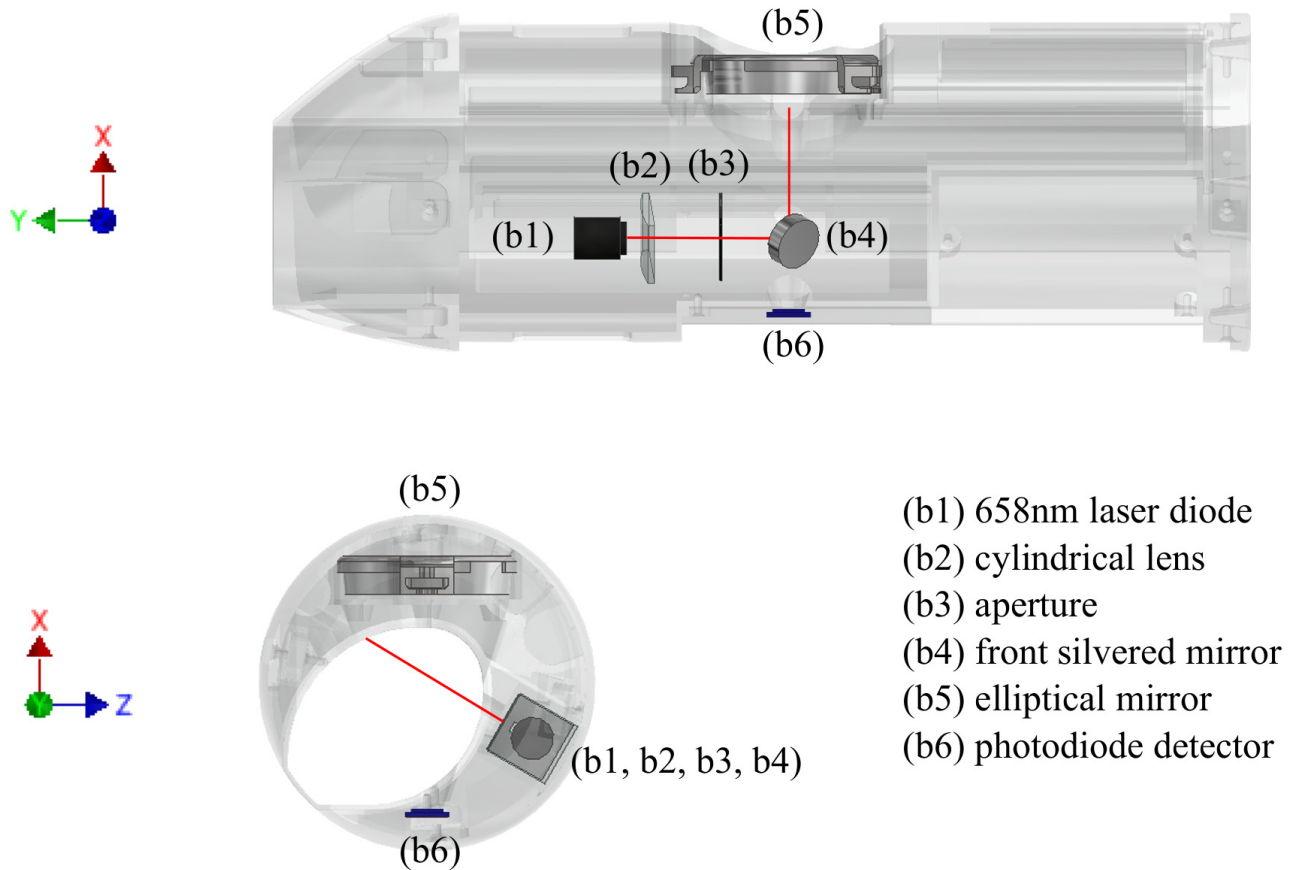
Figure 2. Optical assembly of the UCASS. The top panel shows a view in the xy plane, parallel to the airflow . The bottom panel shows a view in the xz plane, perpendicular to the airflow. The beam forming optics consist of a laser with collimator (b1), a cylindrical lens (b2) and a 2 mm aperture (b3). The beam is directed into the instrument via a front silvered mirror (b4), angled at 45^\circ to the beam. Particles that cross the laser beam will scatter light. The elliptical mirror (b5) collects light scattered between angles 16^\circ and 104^\circ and focuses this onto the detector (b6), where the pulse height and duration is recorded.
