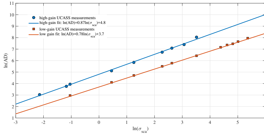
Figure 10. The log of the measured instrument response ( AD ) is plotted against the log of the scattering cross-section ( \sigma_{sca} ) for the calibration standards used. For PSL and Duke Scientific borosilicate glass beads, the mean instrument response is used as this is how the manufacturer defines the particle size. For the Whitehouse Scientific soda-lime glass beads, the sample size is defined by the median and so the median instrument response is plotted.
