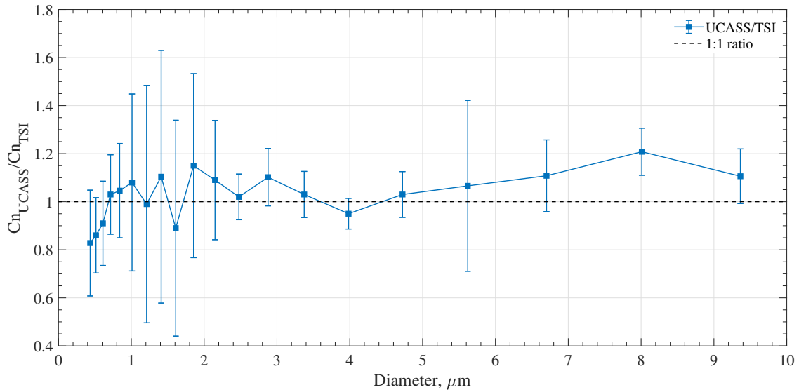
Figure 15. Ratio of UCASS measured number concentrations ( C_{n_{\text{UCASS}}} ) to TSI measured number concentrations ( C_{n_{\text{TSI}}} ) where data points represent means averaged over 100 readings, and error bars represent standard deviations. The 1:1 ratio is shown as a black dashed line.
