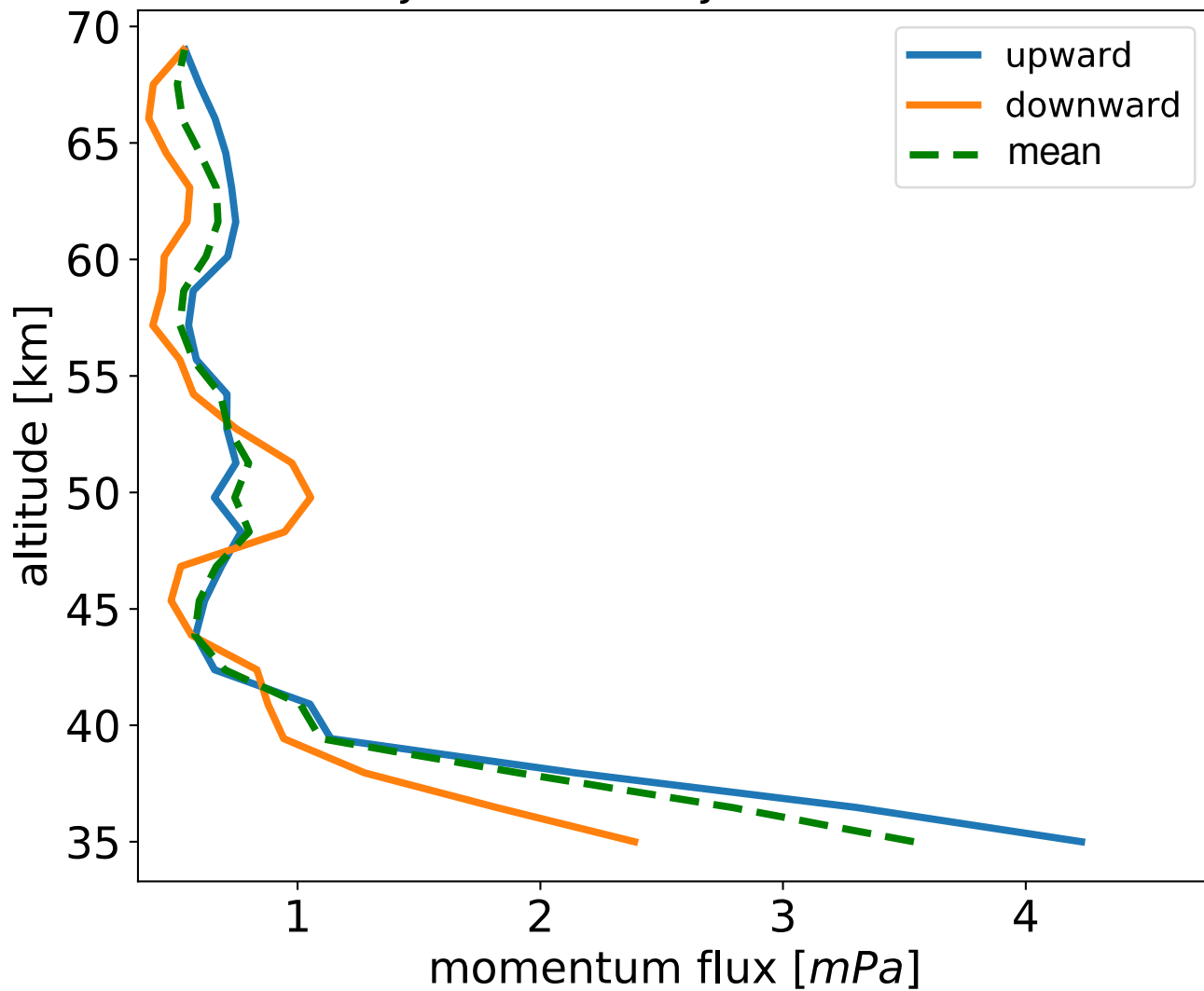
Figure 18. Vertical flux of horizontal momentum averaged through all observed hodographs (dashed), upward (blue), and downward (orange) propagating waves.
