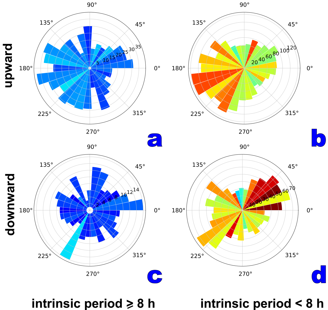
Figure 17. Polar histogram of the upward (upper row) and downward (lower row) propagating GW separated for waves with intrinsic periods \geq 8 hours (left) and < 8 hours (right). The length of the bars represents the number of waves per given horizontal direction. The colors represent the vertical group velocity in km/day.
