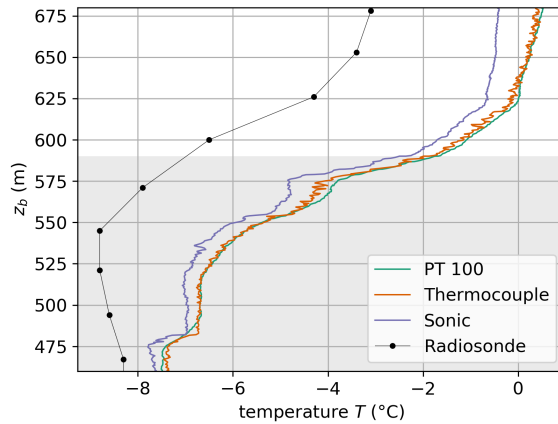
Figure 6. Comparison of balloon-borne temperature measurements measured with the UP descending at 10:00 UTC on 7 June 2017. The plot shows temperature T as a function of barometric altitude z_b around a temperature inversion capping the cloud layer (shaded area, determined from relative humidity and Cloudnet data). The temperature vertical profile includes the time-response corrected PT100, corrected and calibrated thermocouple data and the temperature calculated from the sonic temperature. Plotted data are averaged over 0.5 s intervals. The temperature profile as observed from the radiosonde about 2 hours later is shown for comparison.
