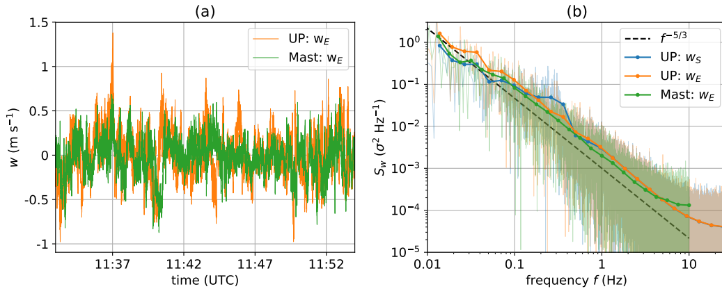
Figure 5. Time series of the vertical wind speed w (a) and power spectral density S_w (b). Wind speeds are shown for the UP measurements with (orange) and without motion correction (blue, only plotted in the right panel). As reference, the sonic data measured on the mast in a height of 10 m are presented (green). The time period is the same as in Fig. 4, the mean horizontal wind speed for this period was 1.7 \text{ m s}^{-1} .
