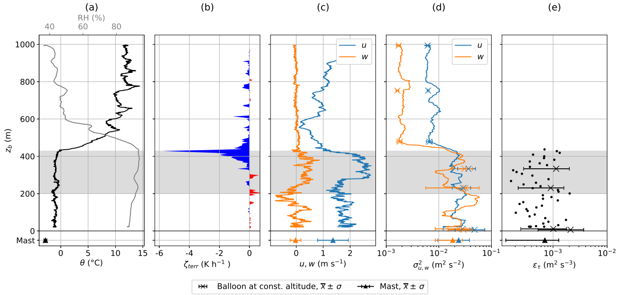
Figure 10. Vertical profiles of potential temperature \theta and relative humidity RH (a), terrestrial heating rate \zeta_{terr} (b), horizontal wind u and vertical wind w (c), local wind speed variance \sigma_{u,w} (d) and the local dissipation rate \varepsilon_\tau (e) observed on 5 June 2017. Solid lines and small dots show slant profile data measured during the ascent (60 s running time window for variances, non-overlapping time segments of 10 s for dissipation rate). Crosses and corresponding horizontal bars in panel d and e show mean and standard deviation of dissipation rate and variances for measurements at constant altitude (segments of typically 10 minutes) obtained during the descent. Averaged ground-based measurements at the meteorological mast are shown as triangles with the standard deviation indicated by horizontal bars. The cloud extend is indicated by the gray shaded area.
