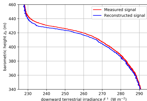
Figure 8. Vertical profile of downward terrestrial irradiance measurement on 5 June 2017 (red) in the cloud top region. The blue line displays the reconstructed signal.
