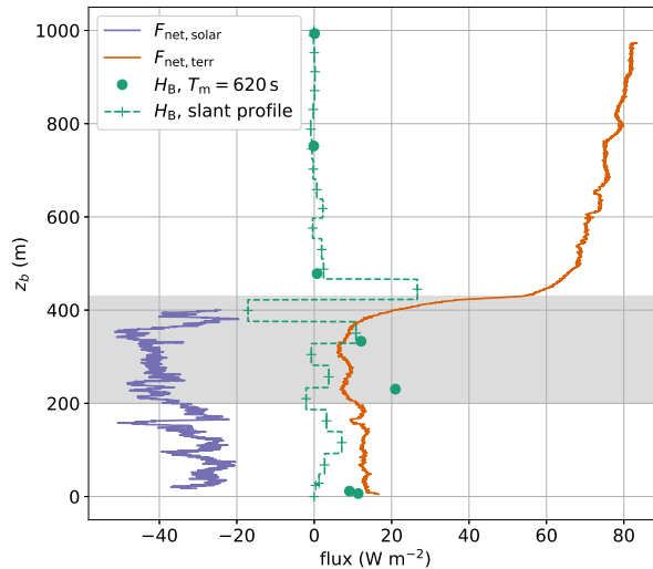
Figure 11. Vertical profile of buoyancy flux H_B and solar and terrestrial net irradiance F_{\text{net}} on 5 June 2017. Balloon-borne buoyancy fluxes are calculated from 620 s time periods at constant altitudes (filled circles) and the slant profile with T_m = 50 s (crosses with dashed line). Positive values indicate upward oriented fluxes.
