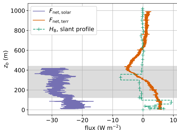
Figure 14. Solar and terrestrial net irradiance F_{\text{net}} and buoyancy flux H_B on 14 June. The buoyancy fluxes are based on the slant profile. The shaded area represents the lower cloud layer.
