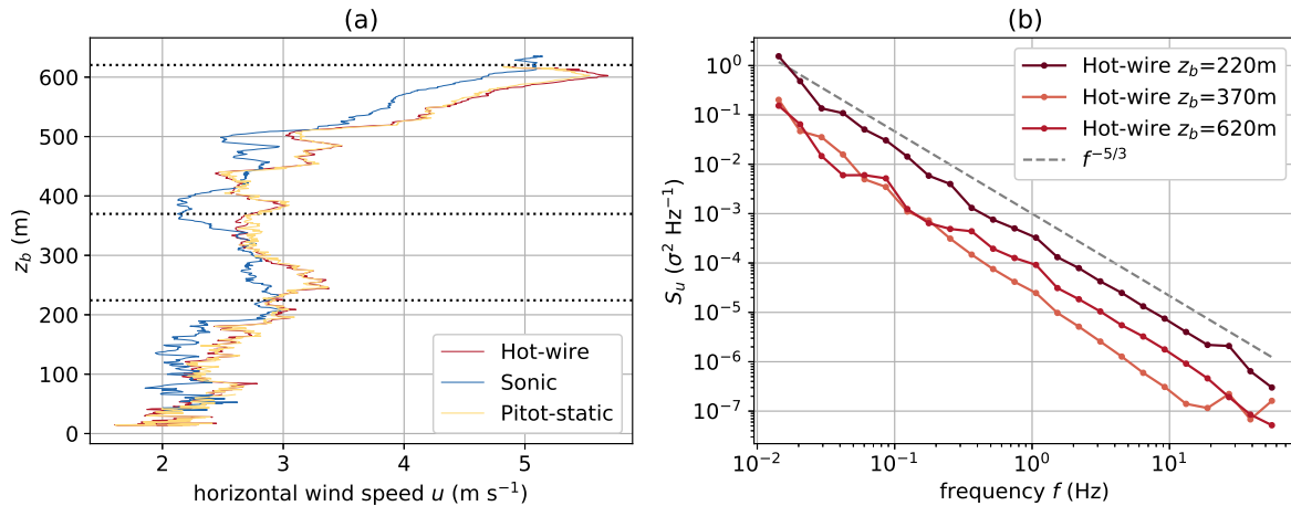
Figure 7. Horizontal wind speed u measured on 8 June 2017 with UP and HP simultaneously. Panel (a) compares the vertical profile of wind speed for measurements with the sonic anemometer, hot-wire anemometer and the Pitot-static probe. The HP was attached 25 m below the UP. Panel (b) contrasts power spectral densities for horizontal wind speed S_u measured with the hot-wire anemometer on three constant altitude segments of \sim 1000 s length (dotted horizontal lines in panel a). The data for the spectra was sampled during an ascent shortly before the descent profile of panel (a).
