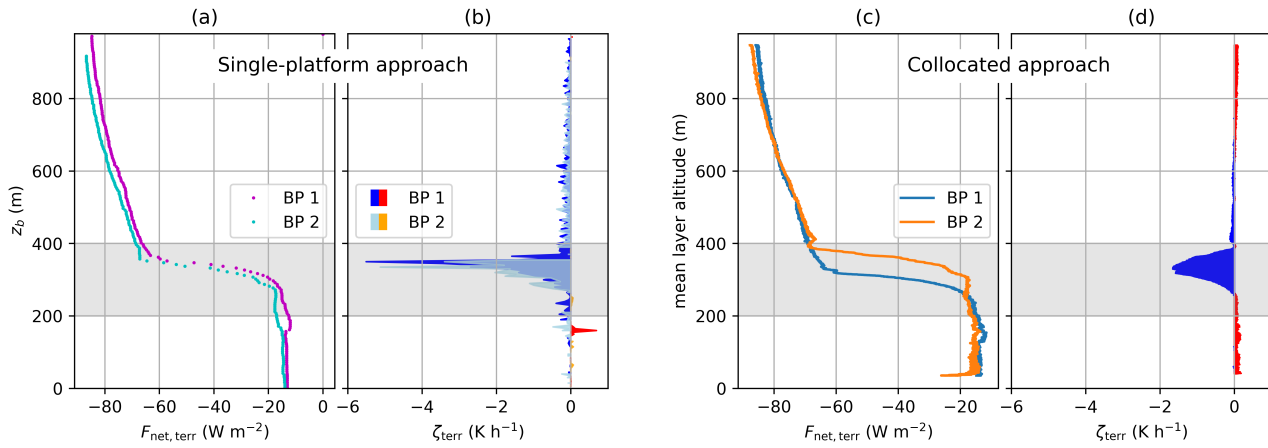
Figure 9. Profiles of net terrestrial irradiance measured on 5 June 2017, 17:00 UTC with respect to the individual sensor altitude (a) and with respect to the mean altitude of the layer between both platforms (c). The calculated heating rates are shown for both individual sensors using the single-platform approach (b) and combining both sensors in the collocated approach (d). Positive values of the heating rate are in red/orange color (indicating a warming), negative values in blue/light blue (indicating a cooling).
