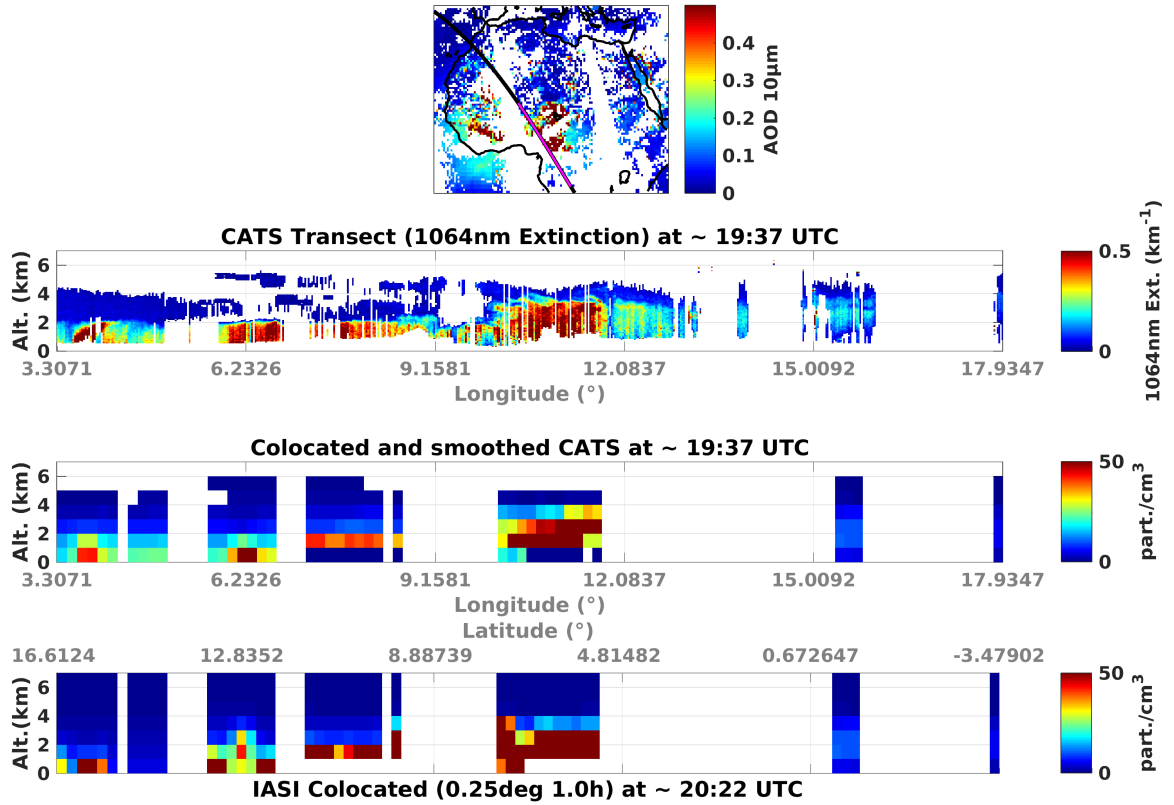
Figure 11. Mineral dust profile comparison along the CATS track on 16 February 2017. The first plot gives the global retrieved AOD by MAPIR together with the pathway of CATS that could be co-located with IASI in time and space. The part which corresponds to the plotted profiles below is given in pink. It covers the Sahel region. The second plot shows the dust extinction profiles along the pink track, as measured by CATS. On the third plot, the CATS data smoothed according to Eq. (7) is presented, on those locations where there is a MAPIR profile. Finally, the fourth plot presents the averaged MAPIR profiles along the track.
