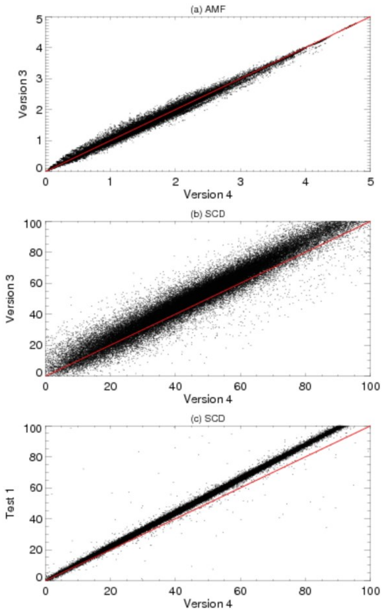
Supplementary Figure 1. (a) Version 4 versus Version 3 AMF comparison; (b) Version 4 versus Version 3 SCD comparison; (c) Version 4 versus Test 1 SCD comparison. Test 1 has the same setting as Version 4 except for the water vapor reference spectrum. Results are for OMI Orbit 10423.
