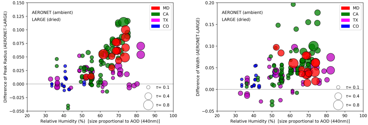
Figure 3. Differences in r_{peak\_conc} [left] and width_{fine\_mode} [right] between AERONET (ambient aerosol) and LARGE (dried aerosol) versus profile relative humidity. Marker is size is proportional to coincident aerosol optical depth (440nm) from AERONET
