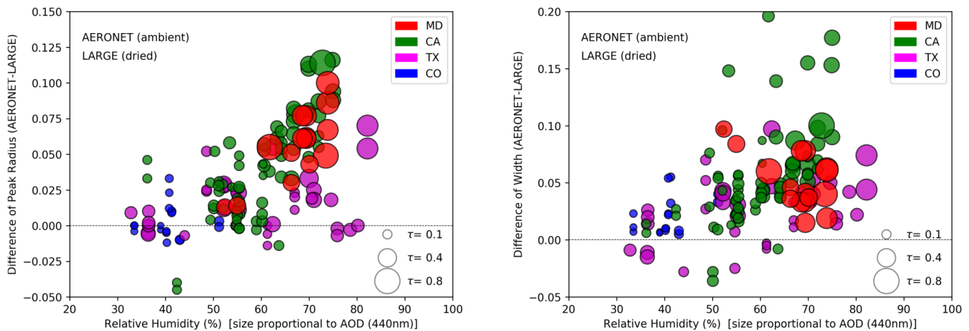
Figure 3. Differences in r_{peak\_conc} [left] and width_{fine\_mode} [right] between AERONET (ambient aerosol) and LARGE (dried aerosol) versus profile relative humidity. Marker size is proportional to coincident aerosol optical depth (440nm) from AERONET
