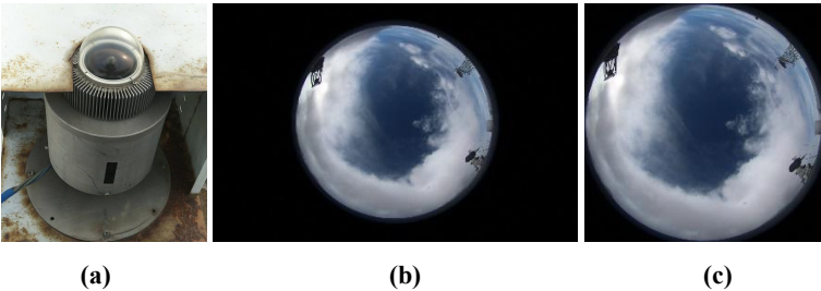
10 Figure 1: Device of ASI and ASI image. (a) device of ASI including a fisheye lens, an industrial camera and a clear glass cover, (b) original RGB color ASI image (2592×1728 pixels), (c) resized RGB color ASI image of (b) (1408×1408 pixels).
