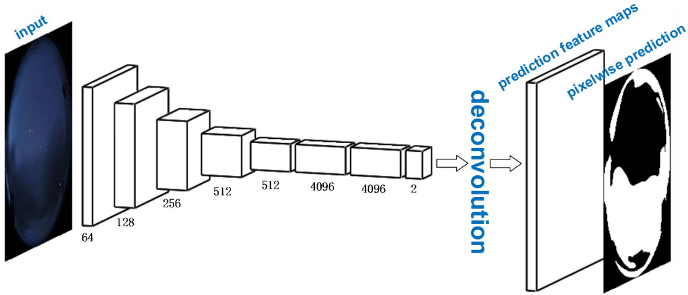
10 Figure 3. Basic components of FCN model including convolutional layers, pooling layers, activation functions and deconvolutional layers.
