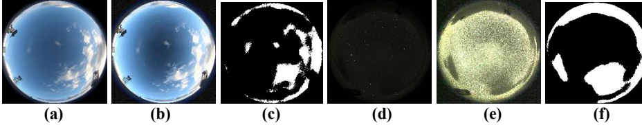
Figure 5. Framework of the complete proposed automatic cloud segmentation based on EFCN-8s. (a) original diurnal ASI image from test set which is the input test image of the EFCN-8s, (b) enhanced diurnal ASI image using the histogram equalization, (c) diurnal cloud segmentation result using the trained EFCN-8s, (d) original nocturnal ASI image from test set which is the input test image of the EFCN-8s, (e) enhanced nocturnal ASI image using the histogram equalization, (f) nocturnal cloud segmentation result using the trained EFCN-8s.
