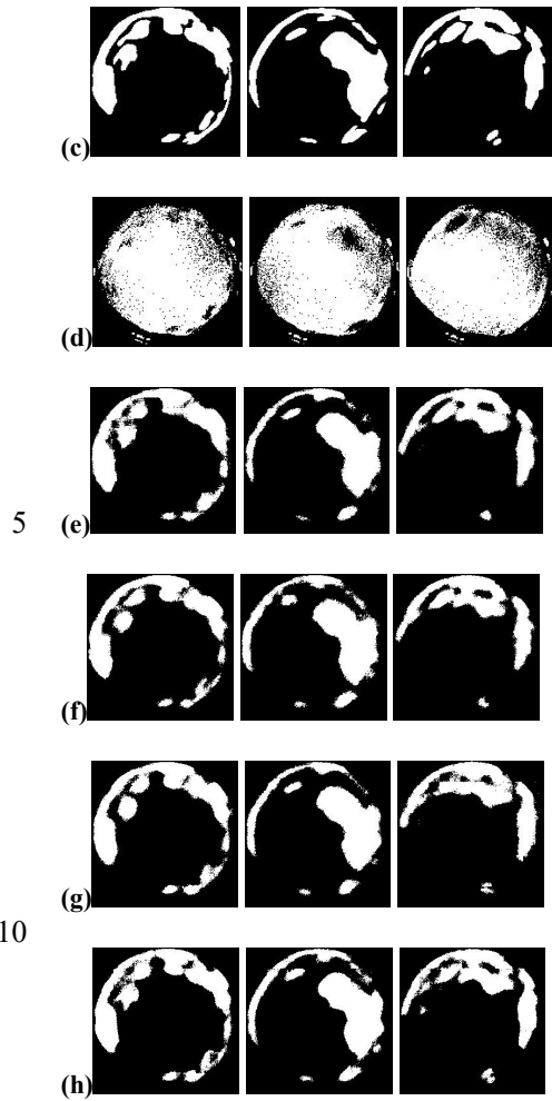
Figure 7. Results of different cloud segmentation algorithms. (a) original nocturnal ASI images, (b) enhanced nocturnal ASI images, (c) ground truth of the corresponding ASI images in (a), (d) results of OTSU, (e) results of EFCN-32s, (f) results of EFCN-16s, (g) results of FCN-8s, (h) results of the proposed EFCN-8s.
