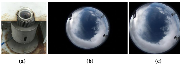
Figure 1: Device of ASI and ASI image. (a) device of ASI including a fisheye lens, an industrial camera and a clear glass cover, (b) original RGB color ASI image (2592×1728 pixels), (c) resized RGB color ASI image of (b) (1408×1408 pixels).
