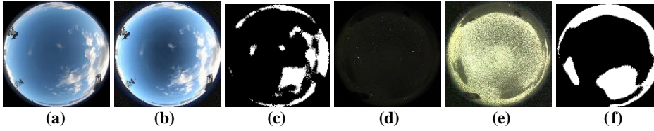
5 Figure 5. Framework of the complete proposed automatic cloud segmentation based on EFCN-8s. (a) original diurnal ASI image from test set which is the input test image of the EFCN-8s, (b) enhanced diurnal ASI image using the histogram equalization, (c) diurnal cloud segmentation result using the trained EFCN-8s, (d) original nocturnal ASI image from test set which is the input test image of the EFCN-8s, (e) enhanced nocturnal ASI image using the histogram equalization, (f) nocturnal cloud segmentation result using the trained EFCN-8s.
