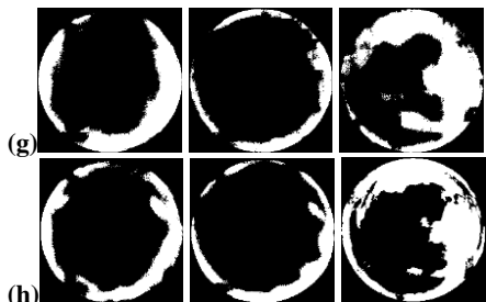
Figure 6. Results of different cloud segmentation algorithms. (a) original diurnal ASI images, (b) enhanced diurnal ASI images, (c) ground truth of the corresponding ASI images in (a), (d) results of OTSU, (e) results of EFCN-32s, (f) results of EFCN-16s, (g) results of FCN-8s, (h) results of the proposed EFCN-8s.
