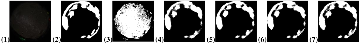
10 (b) Results of different nocturnal cloud segmentation algorithms. (1) Original nocturnal ASI image, (2) ground truth of the corresponding ASI image in (1), (3) result of OTSU, (4) result of EFCN-32s, (5) result of EFCN-16s, (6) result of FCN-8s, (7) result of the proposed EFCN-8s.
