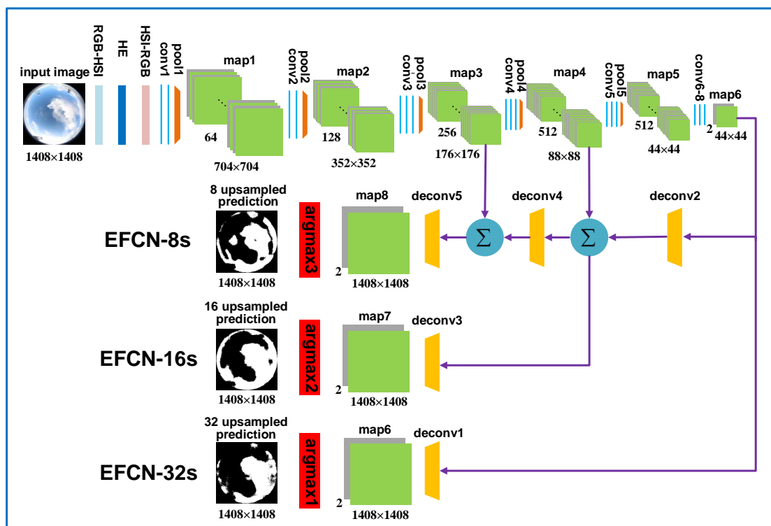
5 Figure 4. Detailed architecture of EFCN model including RGB-HSI layer, histogram equalization layer, HSI-RGB layer, convolutional layers, pooling layers, deconvolutional layers, skip connection, and activation functions.
