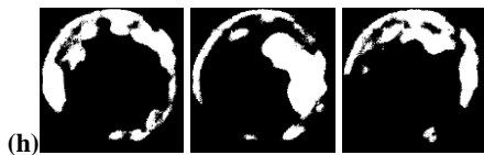
Figure 7. Results of different cloud segmentation algorithms. (a) original nocturnal ASI images, (b) enhanced nocturnal ASI images, (c) ground truth of the corresponding ASI images in (a), (d) results of OTSU, (e) results of EFCN-32s, (f) results of EFCN-16s, (g) results of FCN-8s, (h) results of the proposed EFCN-8s.
