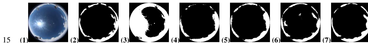
(a) Results of different diurnal cloud segmentation algorithms. (1) Original diurnal ASI image, (2) ground truth of the corresponding ASI image in (1), (3) result of OTSU, (4) result of EFCN-32s, (5) result of EFCN-16s, (6) result of FCN-8s, (7) result of the proposed EFCN-8s.
