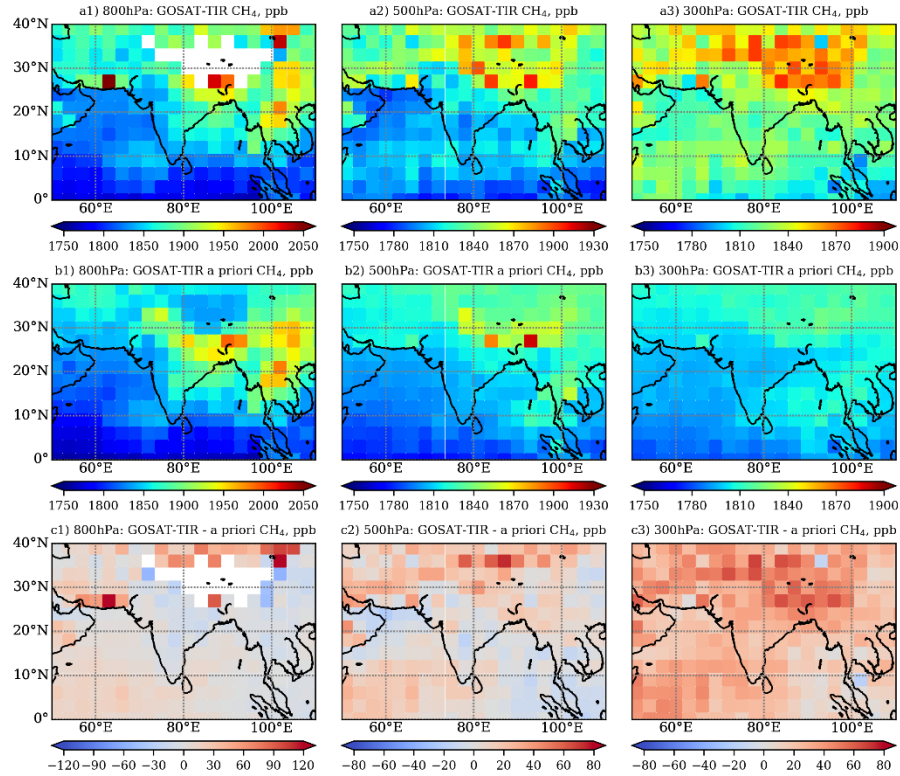
New figure 4: Latitude-longitude distributions of CH 4 at the levels of 800, 500, and 300hPa (the left, middle, and right panels respectively) observed by GOSAT-TIR for the season AMJ 2011. The first upper panels (a1-a3) show GOSAT-TIR CH 4 , the second upper panels (b1-b3) show GOSAT-TIR a priori CH 4 , the third upper panels (c1-c3) show difference between the GOSAT-TIR observed and a priori distributions, respectively.
