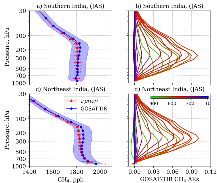
New figure 3: Seasonal mean (July-September 2011) over regions of Southern India (upper panel), and Northeast India (bottom panel). The left columns show the GOSAT-TIR CH 4 a priori with 1- \sigma STD uncertainty of the mean (red line with error bars) and GOSAT-TIR CH 4 profile with the retrieval error (blue line with the shaded area); the right columns depict the averaging kernels of GOSAT-TIR CH 4
