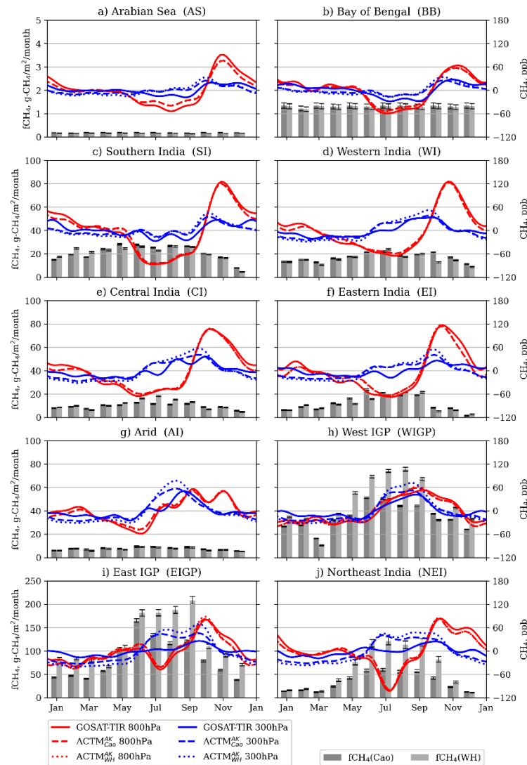
New figure 12: Multi-year (2009-2014) seasonal variation of \text{CH}_4 (right y-axis) derived by the implementation of the Prophet model for levels of 800 (red lines) and 300 hPa (blue lines) over considered regions from GOSAT-TIR (solid line), \text{ACTM}_{\text{Cao}}^{\text{AK}} (dashed line), and \text{ACTM}_{\text{WH}}^{\text{AK}} (dotted line),
