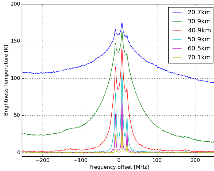
Figure 2: \text{H}^{35}\text{Cl} spectra observed by SMILES.
