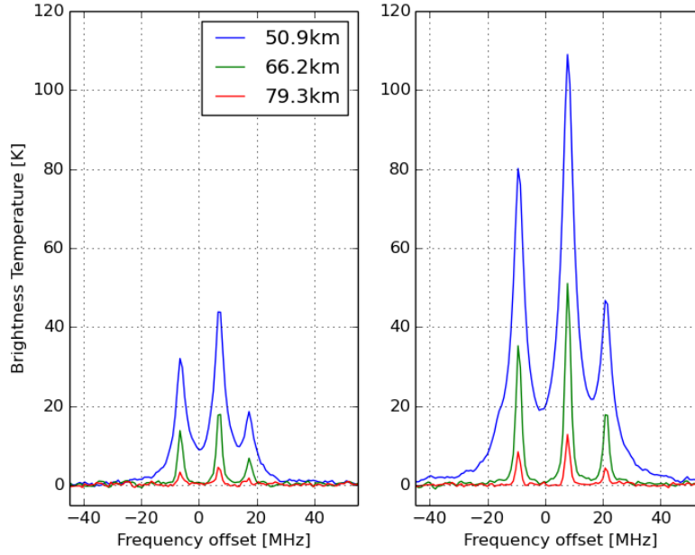
Figure 2. Left: An example of the \text{H}^{37}\text{Cl} spectrum-spectra observed by SMILES from a single scan measurement. Tangent heights are approximately 50, 65, and 80 km. Center frequency is 624.98 GHz. Right: An example of the \text{H}^{35}\text{Cl} spectrum-spectra for the same condition as for the \text{H}^{37}\text{Cl} spectrum-spectra . Center frequency is 625.92 GHz.
