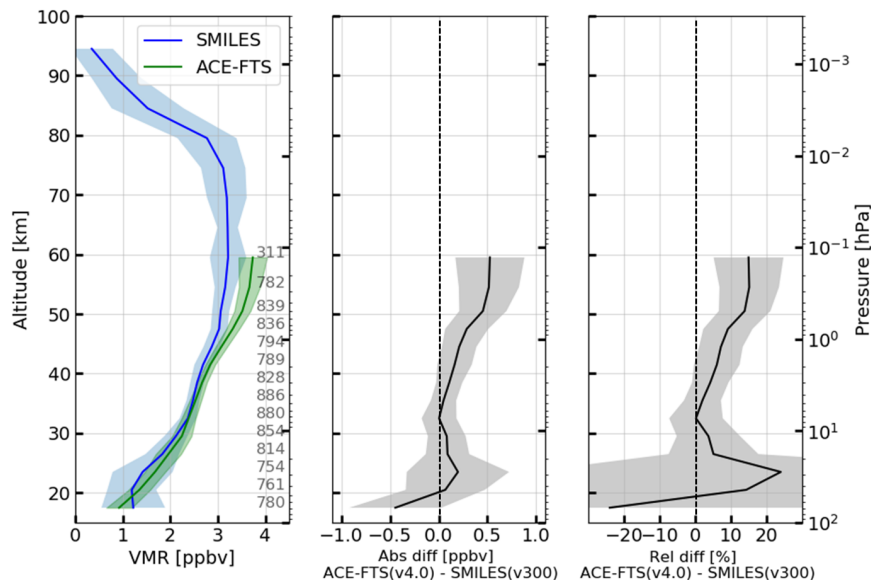
Figure 8. Comparison between SMILES and ACE-FTS profiles from October 16, 2009 to April 17, 2010. Left: The mean HCl VMR values (solid lines) and 1\sigma (shaded areas) for SMILES and ACE-FTS. The blue and green lines are the SMILES and ACE-FTS HCl profiles, respectively. Middle: The absolute difference between the SMILES and ACE-FTS profiles calculated using Eq (3). Right: The relative difference between the SMILES and ACE-FTS profiles calculated using Eq (4).
