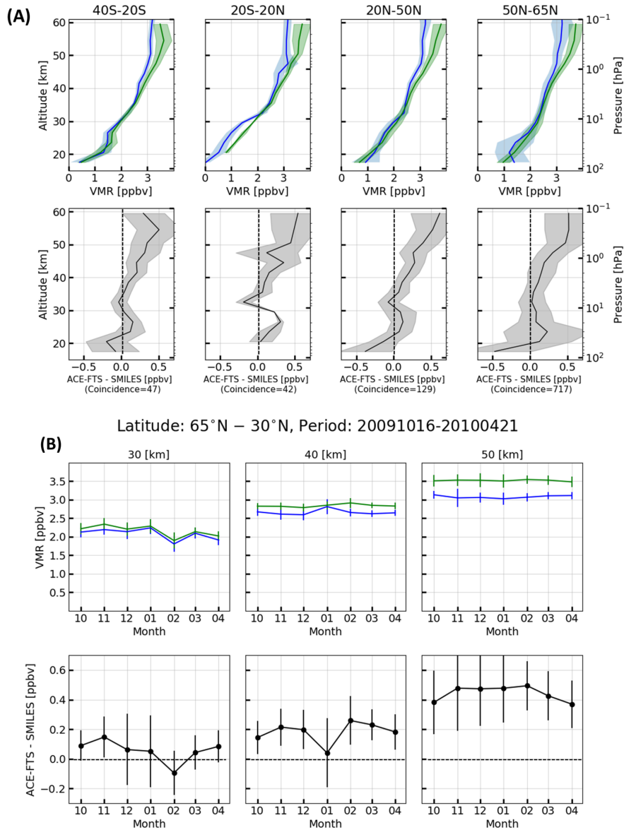
Figure 9. Figure-(A): The mean of HCl values, 1\sigma and the absolute difference for each latitudinal region are shown. Upper row: The blue and green lines indicate the SMILES HCl profiles and ACE-FTS profiles for each latitudinal region, 40^{\circ}\text{S}-20^{\circ}\text{S} , 20^{\circ}\text{S}-20^{\circ}\text{N} , 20^{\circ}\text{N}-50^{\circ}\text{N} , and 50^{\circ}\text{N}-65^{\circ}\text{N} from the left side. Lower row: The absolute difference between the SMILES and ACE-FTS profiles calculated using Eq (3) for each latitudinal region. Figure-(B): Seasonal variation in the SMILES and ACE-FTS HCl profiles at three altitude levels. Latitudinal range is 30^{\circ}\text{N} - 65^{\circ}\text{N} . Upper row: Monthly mean of SMILES (blue) and ACE-FTS (green) HCl profiles for each altitude level. The error bars correspond the 1\sigma . Lower row: The mean and 1\sigma uncertainty of the absolute difference.
