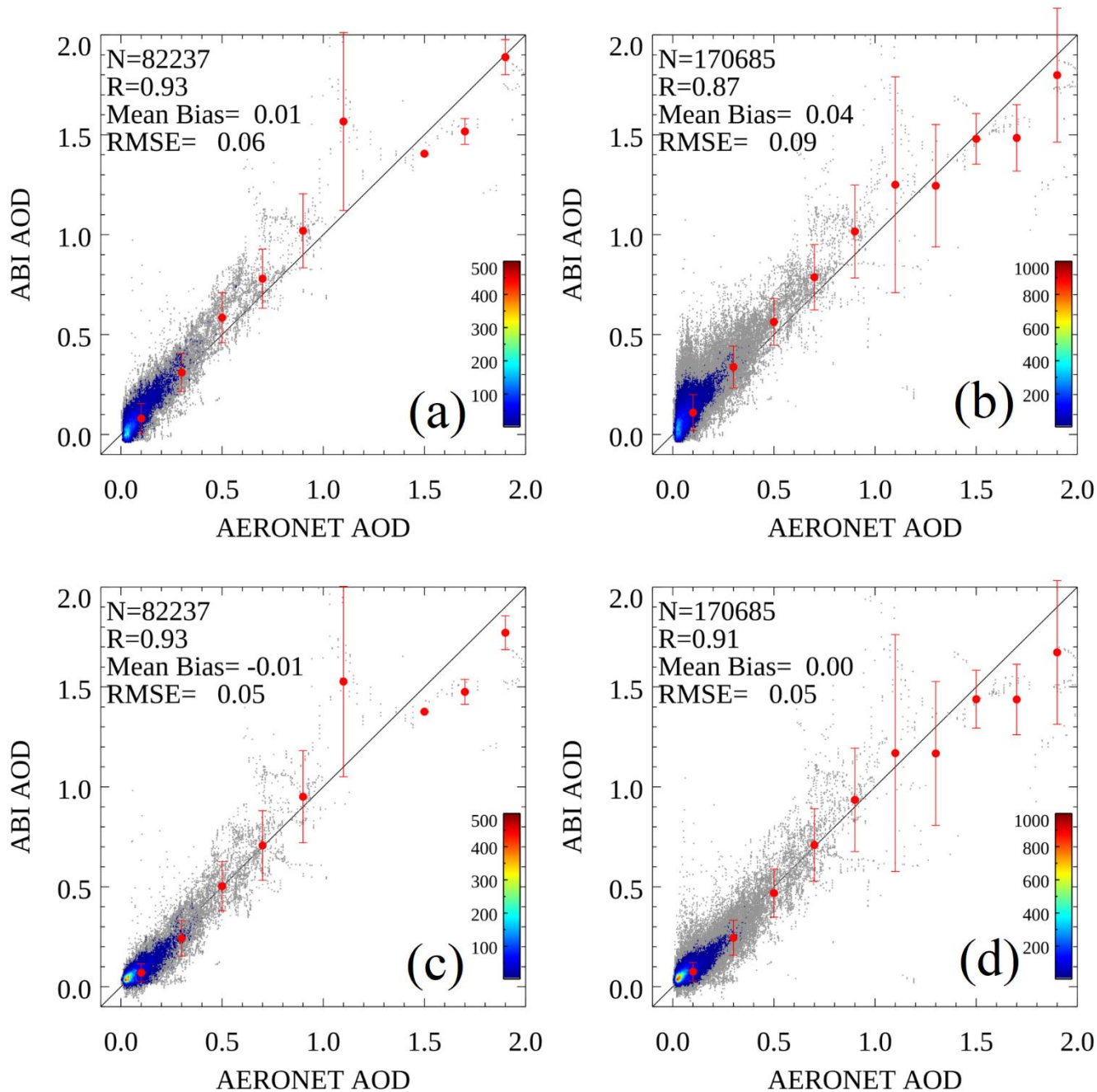
750 Figure 6. Scatter plots of GOES-16 ABI AOD vs AERONET AOD for August 6, 2018 to December 31, 2018 across the CONUS domain: (a) high quality ABI AOD before bias correction, (b) top 2 qualities ABI AOD before bias correction, (c) high quality ABI AOD after bias correction, and (d) top 2 qualities ABI AOD after bias correction. The red circles and vertical bars are the mean ABI AOD and the standard deviation of errors of data points falling in the bins with size of 0.2. In the plots, N is the number of matchups, R is the correlation coefficient, and RMSE is the root mean square error.
