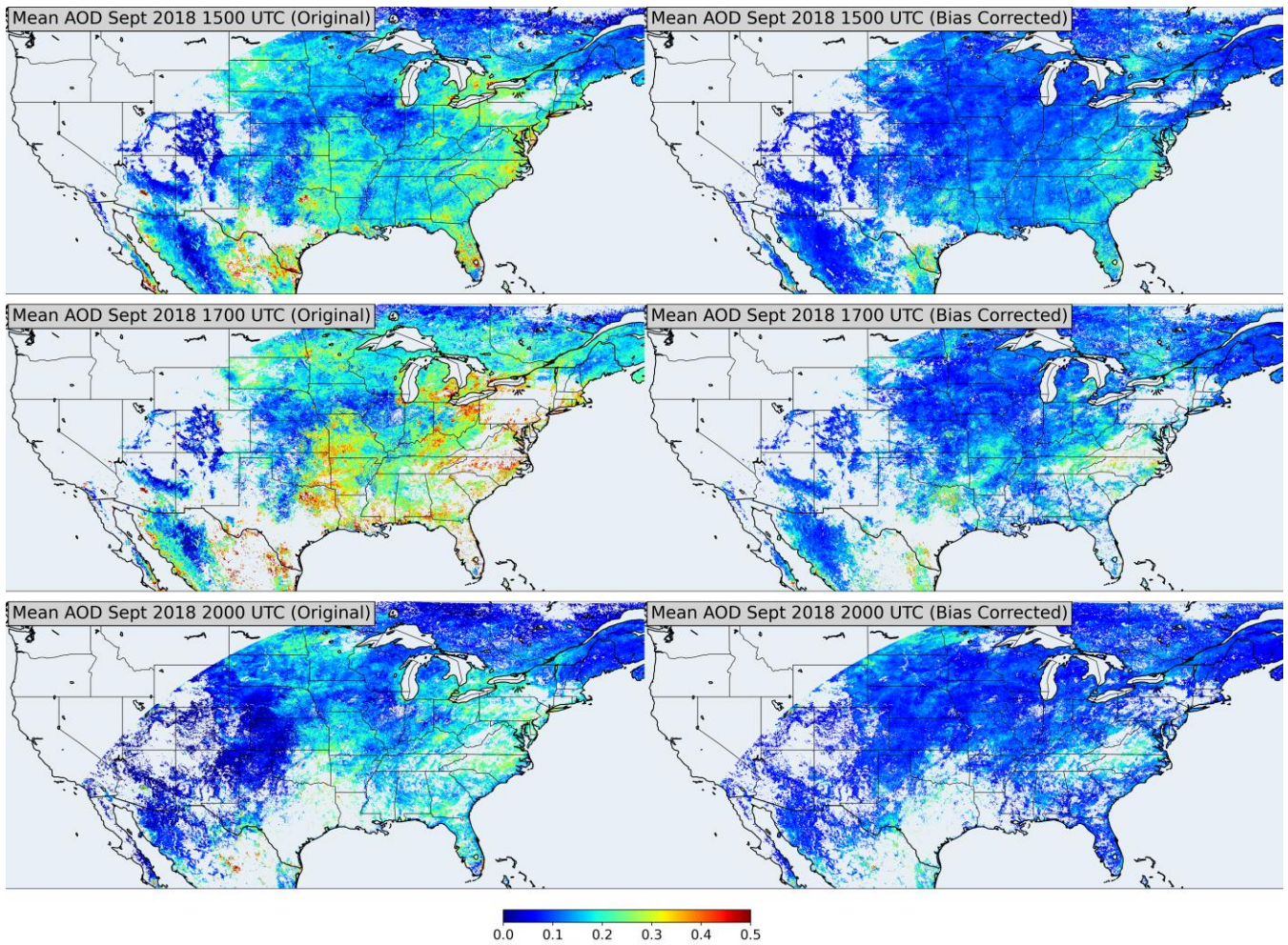
765 Figure 9. Monthly mean AOD (top 2 qualities) for September 2018 at three time steps, i.e. 1500 UTC, 1700 UTC and 2000 UTC, for the original ABI AOD (left column) and bias corrected AOD (right column).
