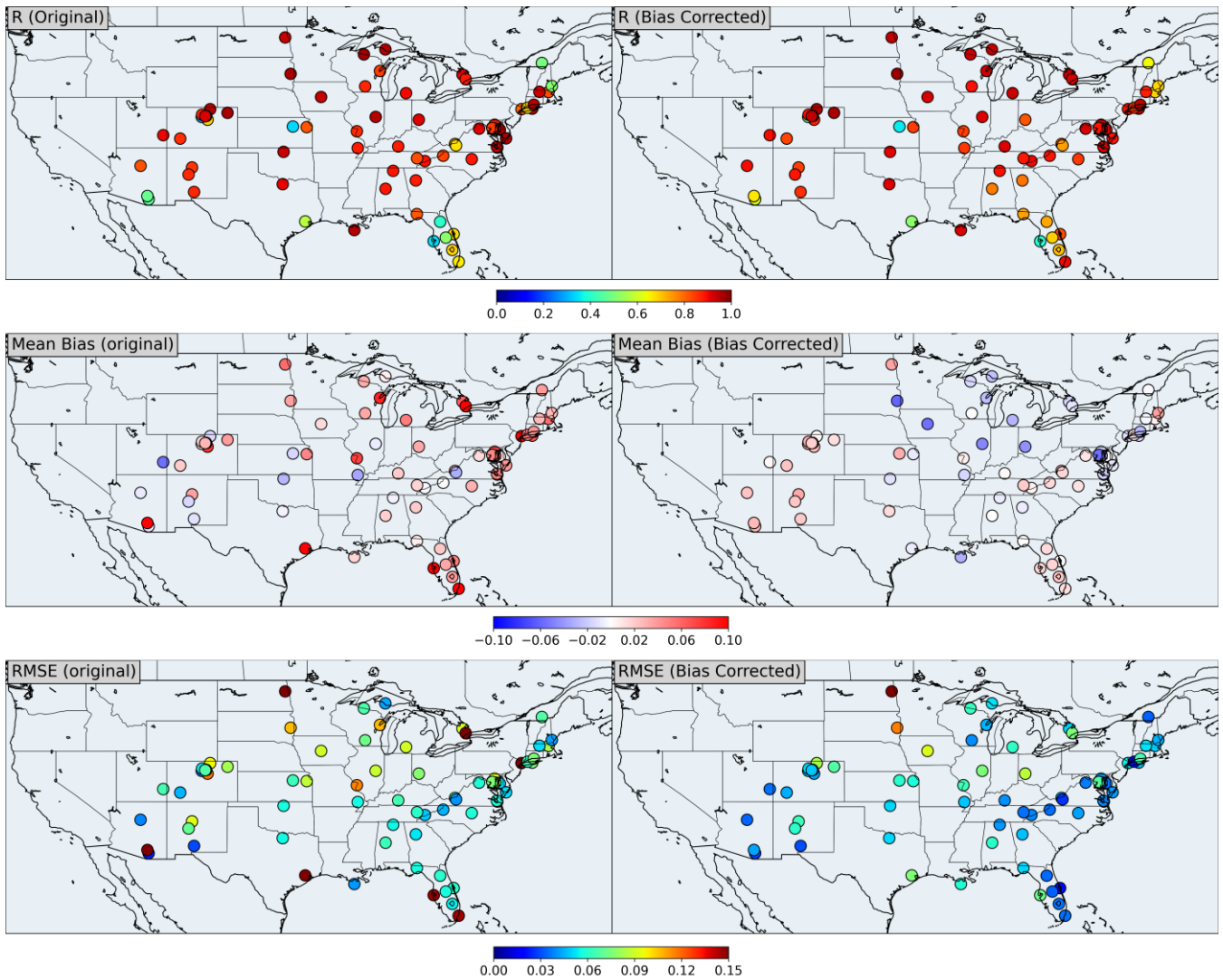
Figure 10. Maps of correlation coefficients, mean biases and RMSEs at AERONET sites with more than 400 matchups for the time period August 6-December 31, 2018 for the original ABI AOD (top 2 qualities) vs AERONET AOD (left column) and for the bias corrected ABI AOD (top 2 qualities) vs AERONET AOD (right column).
