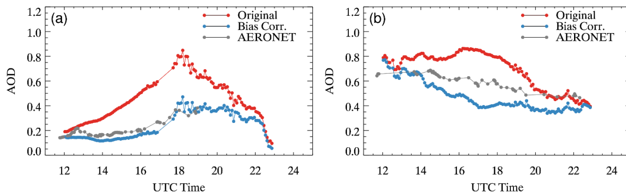
785 Figure 14. Time series of original (uncorrected) GOES-16 ABI AOD, bias corrected ABI AOD, and AERONET AOD at the CCNY AERONET site on (a) August 15, 2018 and (b) August 16, 2018, showing the difference in bias corrected ABI AOD relative to AERONET AOD on two consecutive days with moderate aerosol loading.
