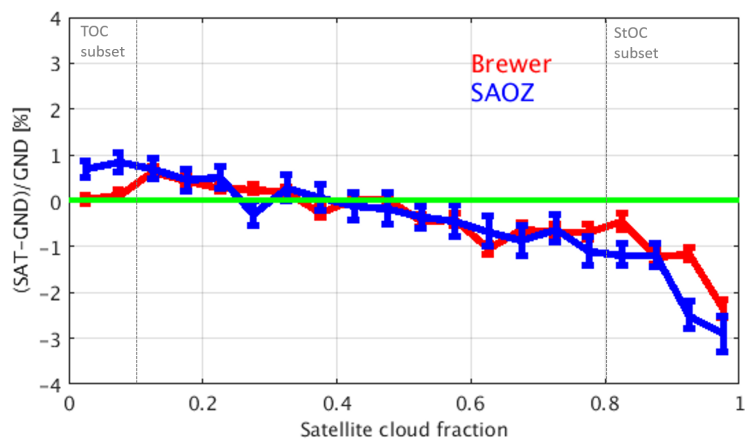
Figure 6. Dependence of TROPOMI total ozone column bias on the cloud fraction over the observed scene (TROPOMI L2_O3 OFFL V01.01.01-01.01.08). Comparisons are done over a two year period with respect to co-located total ozone column data from the Brewer and SAOZ monitoring networks. The two curves are normalised (on a per-station basis) on the mean difference over the 0.2–0.6 CF range, in order to reduce the station-to-station scatter of the mean bias. The two dashed vertical lines identify the cloud-free and cloudy subsets used by the CCD algorithm.
