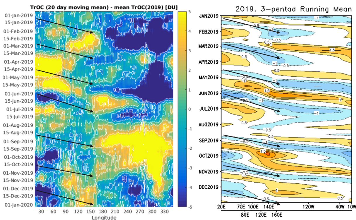
Figure 14. Anomaly of the 20-day moving mean TROPOMI tropospheric ozone column (left) and the NOAA/CPC Madden-Julian Oscillation index (right) during 2019 over the equatorial Indo-Pacific Oceans. Arrows indicate periodical, eastward propagating enhancements in convective activity due to MJO and the corresponding low levels of tropospheric ozone.
