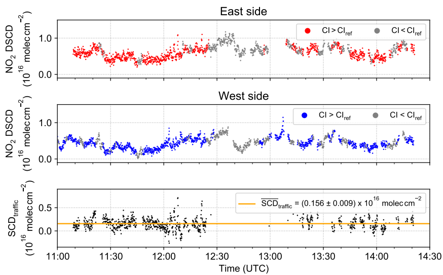
Figure A4. Analysis result of the \text{NO}_2 DSCDs for both sides (blue: west side, upwind; red: east side, downwind) with applied cloud filter based on the colour index (CI, intensity ratio 320 nm/440 nm). The grey data points are filtered out. The resulting difference \text{SCD}_{\text{traffic}} is depicted in the lowermost panel yielding slightly lower \text{NO}_2 SCDs compared to the unfiltered case.
