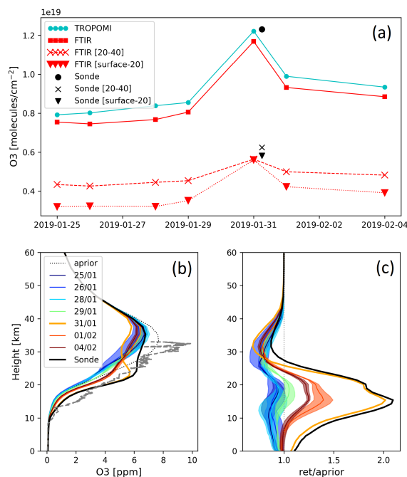
Figure 6. (a): the time series of the total and partial columns daily means from co-located FTIR and TROPOMI measurements between 25 January 2019 and 4 February 2019, and one ozonesonde profile (with smoothing using FTIR averaging kernel), on 31 January 2019 at Xianghe. For visualizing, the ozonesonde measurement is shifted by 6 hours. (b): the FTIR a priori (grey dot line) and retrieved (colored with date) profiles during this period. The shadow is the STD of the retrieved profile for each day. The grey dashed line is the original ozonesonde profile, and the back solid line is the smoothed ozonesonde profile. (c): the ratios of the FTIR retrieved profiles and the smoothed ozonesonde profile to the FTIR a priori profile.
