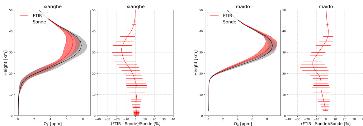
Figure 4. The O_3 profiles from the smoothed ozonesonde and FTIR retrievals (the solid line is the mean and the shadow is the STD), together with their relative differences (the solid line is the mean and the errorbar is the STD) at Xianghe (left) and Maïdo (right).
