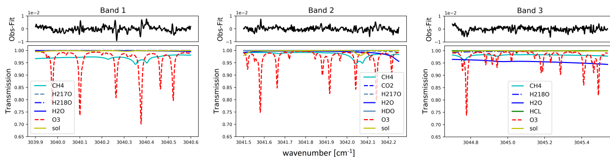
Figure 1. Example of spectral fits in the three microwindows for O 3 retrievals at Xianghe. Lower panels: the normalized transmittance from each atmospheric species and solar lines. Upper panels: the difference between the observed and fitted spectra (Obs-Fit).
