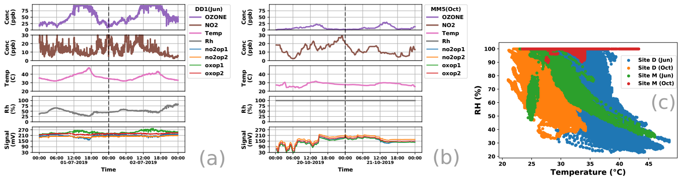
Figure 2. Figures 2(a,b) present time series for raw parameters measured using the reference monitors ( \text{NO}_2 and \text{O}_3 concentrations) as well as those measured using the SATVAM LCAQ sensors (RH, T, no2op1, no2op2, oxop1, oxop2). Figure 2(a) considers a 48 hour period during the Jun deployment (01-02 July 2019) at site D with signal measurements taken from the sensor DD1 whereas Fig. 2(b) considers a 48 hour period during the Oct deployment (20-21 October 2019) at site M with signal measurements taken from the sensor MM5 (see Sec. 2.3 for conventions used in naming sensors e.g. DD1, MM5, etc.). Values for site D are available at 1 minute intervals while those for site M are averaged over 15-min intervals. Thus, the left plot is more granular than the right plot. Site D experiences higher levels of both \text{NO}_2 and \text{O}_3 as compared to site M. Figure 2(c) presents a scatter plot showing variations in RH and T at the two sites across the two deployments. The sites offer substantially diverse weather conditions. Site D exhibits wide variations in RH and T levels during both deployments. Site M exhibits almost uniformly high RH levels during the Oct deployment which coincided with the retreating monsoons.
