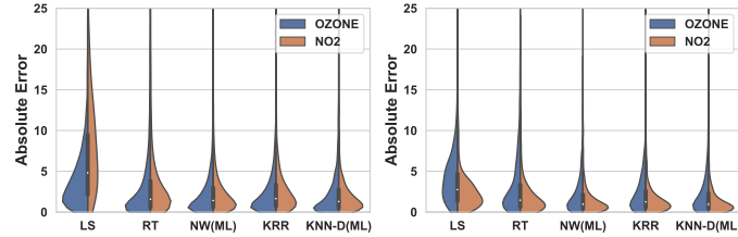
Figure 5. The violin plots on the left and ( resp. rightdepict ) show the distribution of absolute errors incurred by various models on respectively , the DD1(Oct) and ( resp. MM5(Jun) ) datasets. KNN-D(ML) offers visibly superior performance than several as compared to other algorithms such as LS and RT.
