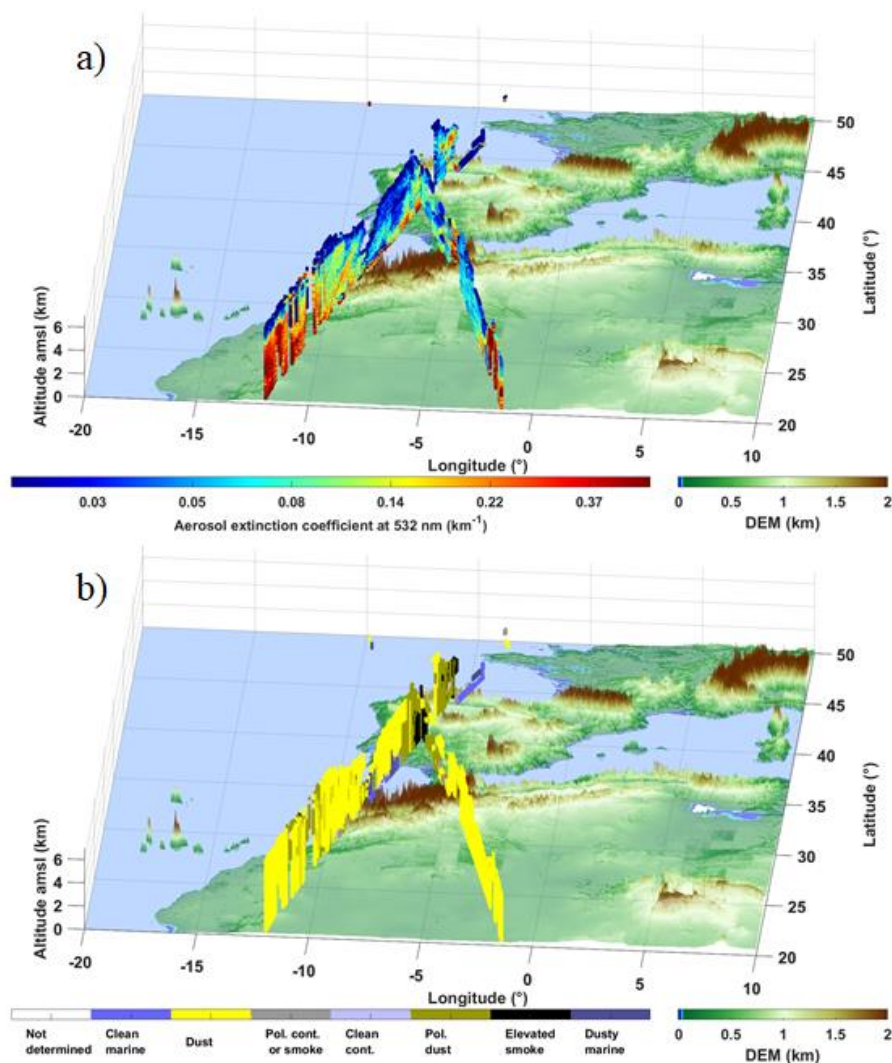
5 Figure 12: CALIOP-derived a) aerosol extinction coefficient at 532 nm and b) aerosol typing. Two orbits are plotted on 13 August 2011, the first one during night time at ~0240 UTC (westernmost over North Africa) and the second one during day time at ~1340 UTC (easternmost over North Africa).
