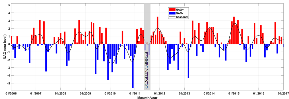
Figure 9: Temporal evolution of the monthly average North Atlantic Oscillation (NAO) index. The data are those of the site https://climatedataguide.ucar.edu/climate-data/hurrell-north-atlantic-oscillation-nao-index-station-based . The grey area highlights the summer 2011 where the NITENDO field campaign took place.
