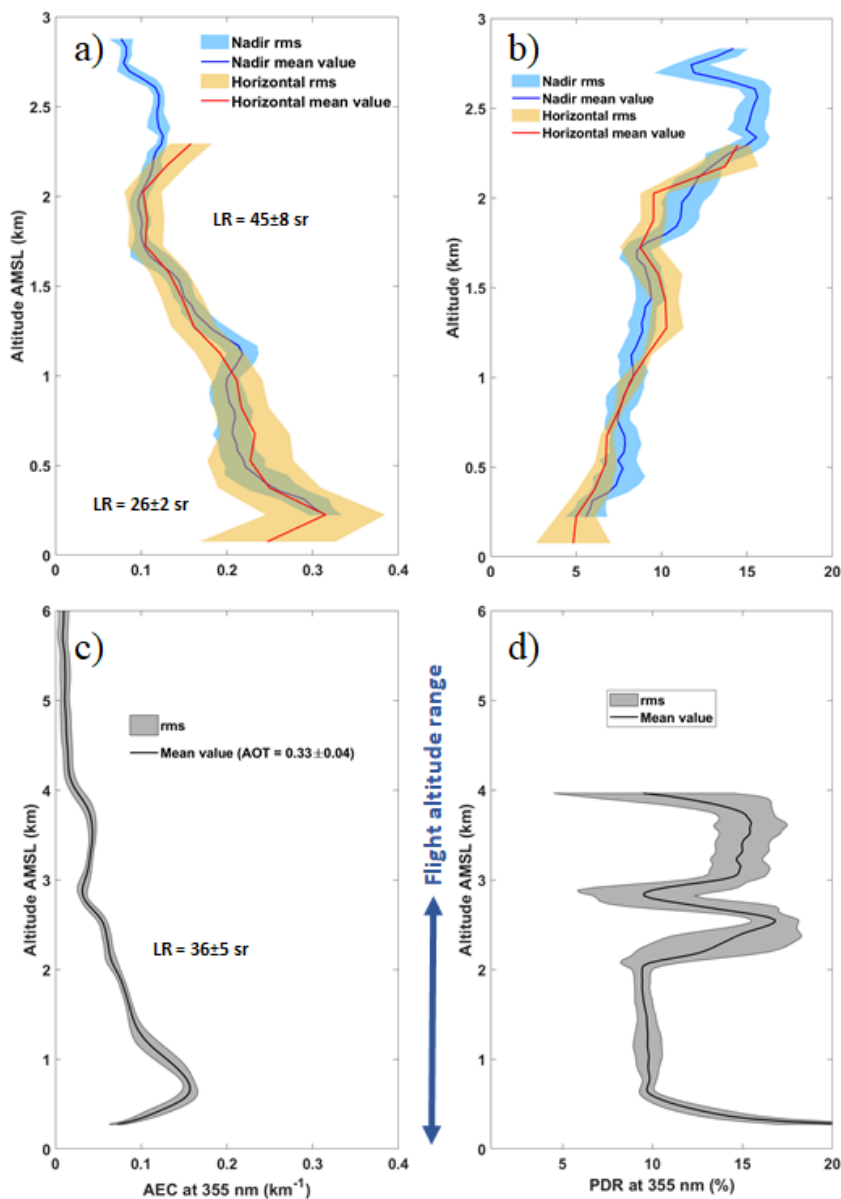
5 Figure 6: Vertical profiles of a) the aerosol extinction coefficient (AEC) derived from the airborne lidar for horizontal and nadir sightings, b) the particle depolarization ratio (PDR) derived from the airborne lidar for horizontal and nadir sightings, c) the AEC derived from the ground-based lidar and d) the PDR derived from the ground-based lidar. The ground-based profiles correspond to an average between 1900 and 2200 local time on 13 August 2011. The aerosol optical thickness (AOT) is also given in Figure 6c.
