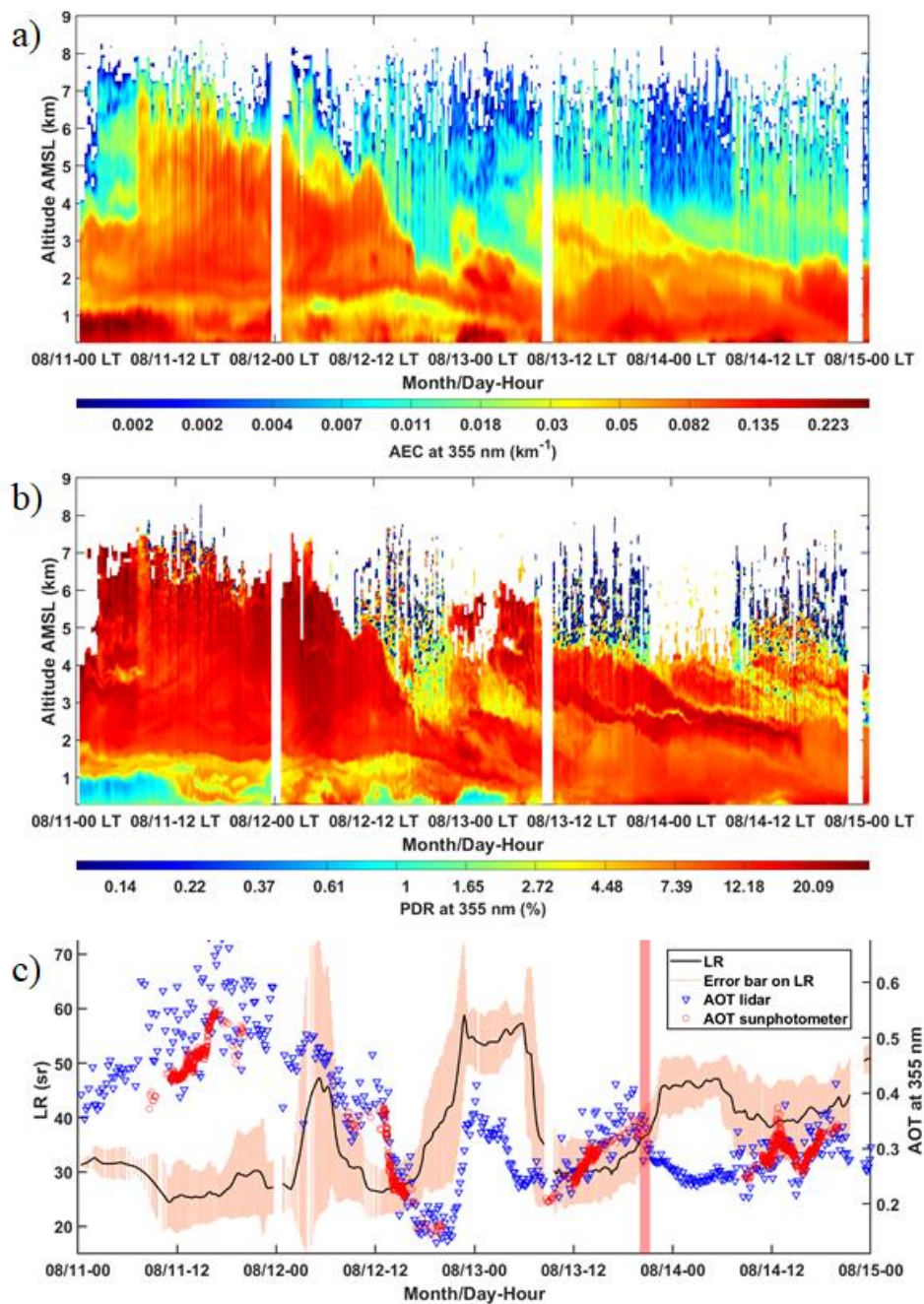
5 Figure 7: Ground-based lidar-derived temporal evolution of the vertical profiles of a) the aerosol extinction coefficient (AEC), the particle depolarization ratio (PDR) and c) the lidar ratio (LR). In Figure 7c, the aerosol optical thickness (AOT) as derived from both the ground-based lidar and sun photometer, are also shown. The time location of the ULA flight over the Strait of Gibraltar is highlighted by the light-red area, around 2030 LT on 13 August 2011.
