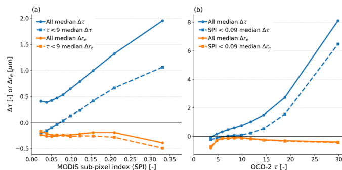
630 Figure 6. Binned median bias in OCO-2 minus MODIS \tau (blue) or r_e (orange) when (a) binned by MODIS sub-pixel index (SPI) derived from the 250 m sampling at \lambda = 0.66 \mu\text{m} or (b) binned by the OCO-2 LUT retrieved \tau . Solid lines are for the full samples, and dashed lines are for the subset (a) below the median OCO-2 \tau or (b) below the median MODIS SPI.
