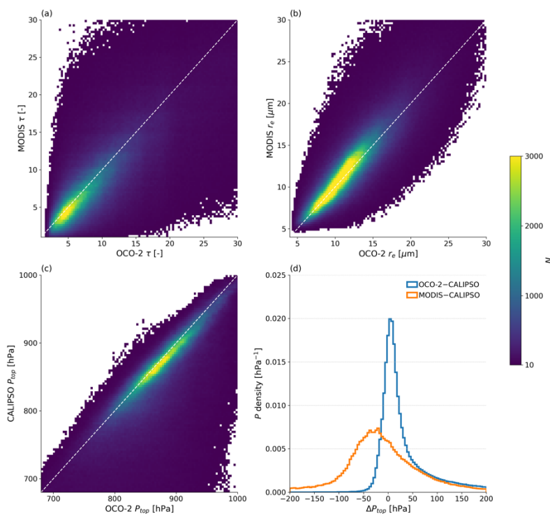
625 Figure 5. Inter-satellite comparison of retrieved cloud properties, (a) MODIS vs. OCO-2 \tau , (b) MODIS vs. OCO-2 r_e , (c) CALIPSO vs. OCO-2 P_{top} and (d) OCO-2 or MODIS P_{top} minus CALIPSO P_{top} . The colour bar on the right applies to (a)–(c).
