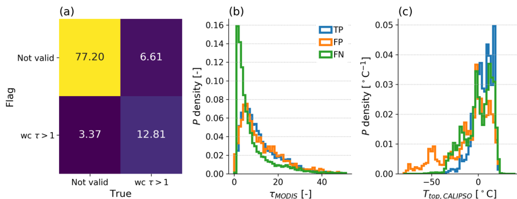
615 Figure 3. (a) confusion matrix with values in %, comparing trained classifier (“flag”) with collocated MODIS-CALIPSO definitions (“truth”) and entries being classified as single-layer water cloud (wc) with \tau > 1 , or “not valid”, (b) normalised histograms of collocated MODIS \tau where retrieved, for true positives (TP), false positives (FP) and false negatives (FN), (c) normalised histograms of collocated CALIPSO T_{top} where retrieved, colours as in (b).
