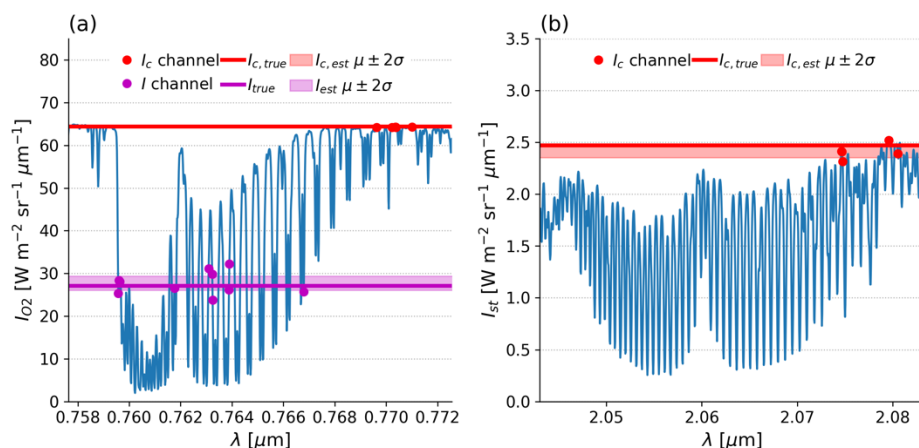
605 Figure 2. Mean cloudy scene spectra in (a) the O 2 A-band and (b) the strong CO 2 band. The channels used in the lookup tables are shown as points, red for the continuum radiance I_c and magenta for the O 2 absorption band radiance I . Thick horizontal lines represent the “truth”, either the L1bSc file’s continuum radiance for I_c or the mean of the 600–609 th brightest undamaged channels (i.e. the 60 th super-channel) for I . The shaded bands of the same colour are the mean \pm 2 standard errors based on the selected channel sample sizes (5 for I_c , 10 for I ).
