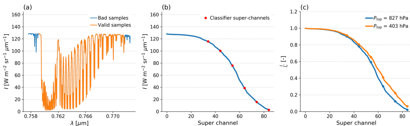
Figure 1.(a) OCO-2 A-band spectrum for a cloud with CALIPSO P_{top} = 827 hPa, with the used channels in orange and non-used (e.g. due to FPA pixel damage) in blue, (b) the smoothed super-channel spectrum, where the channels are ranked in brightness and then non-overlapping 10-channel means are taken. The super channels used in the classifier are shown in red. (c) Comparison of the ranked ratio I/I_c between this cloud, and a higher altitude ( P_{top} = 403 hPa). The SZA is within 0.01^\circ and the continuum radiance within 1 % between each spectrum, the differences are largely due to the shorter path length resulting in less absorption for the higher altitude cloud.
