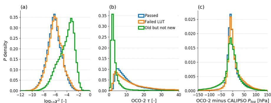
635 Figure 7. Normalised histograms of OCO2CLD-LIDAR-AUX outputs where SZA < 45^\circ separated into whether the soundings pass the new pre-processor flag and retrieval or not. The “passed” set are those that returned valid cloud properties from the LUT along with T_{top} > 0 \text{ }^\circ\text{C} , the “failed LUT” case gave invalid cloud values or had T_{top} < 0 \text{ }^\circ\text{C} , and the “old but not new” set are those that were attempted in OCO2CLD-LIDAR-AUX but are not passed by the new classifier. (a) Logarithm of \chi^2 , (b) retrieved \tau , (c) P_{top} minus the closest CALIPSO retrieved P_{top} .
