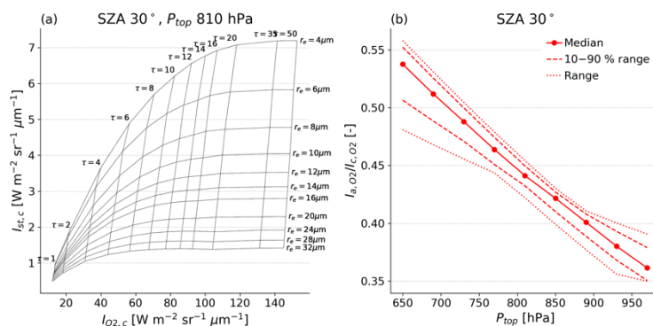
620 Figure 4. Example lookup table (LUT) properties. (a) radiance in the strong CO 2 continuum as a function of A-band continuum radiance at SZA = 30° for clouds with P_{top} = 810 hPa and \tau , r_e as labelled, (b) A-band absorption ratio within the SZA = 30° table as a function of P_{top} . The solid line is the median value within each LUT at a fixed P_{top} , the dashed lines span the 10–90 % range and the dotted lines span the minimum to maximum values.
