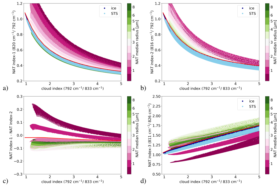
Figure 3. Scatter plots for different NAT indices versus cloud index. Correlations between different NAT indices and cloud index for the simulated PSC scenarios. a) NAT index-1 ( 819 - 821 \text{ cm}^{-1} )/( 791 - 793 \text{ cm}^{-1} ); b) NAT index-2 ( 815 - 817 \text{ cm}^{-1} )/( 791 - 793 \text{ cm}^{-1} ); c) NAT index-1 – NAT index-2; d) NAT index-3 ( 810 - 812 \text{ cm}^{-1} )/( 825 - 827 \text{ cm}^{-1} ). The red lines show the separation lines, which mark the upper envelope of the regions of STS and ice (in a), b), and d) or the region of medium and large NAT (in c)). Simulation results for ice and STS are in shown in dark and light blue, respectively.
