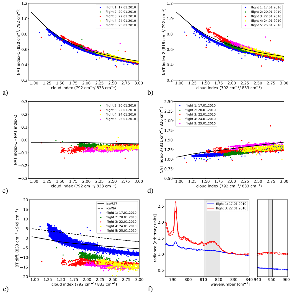
Figure 9. Scatter-plots for Correlations between the different NAT indices versus and cloud index for the CRISTA-NF observations during RECONCILE flights 1 – 5. a) NAT index-1 (819 – 821 cm -1 )/(791 – 793 cm -1 ) (MW3/MW1); b) NAT index-2 (815 – 817 cm -1 )/(791 – 793 cm -1 ) (MW4/MW1); c) NAT index-1 – NAT index-2; d) NAT index-3 (810 – 812 cm -1 )/(825 – 827 cm -1 ) (MW5/MW6). The black lines show the separation lines, which mark the upper envelope of the regions of STS and ice (in a), b), and d) or the region of medium and large NAT (in c). Simulation results for ice and STS are in shown in dark and light blue, respectively. e) Scatter-plot for Correlation between the BT difference (832 – 834 cm -1 ) – (947.5 – 950.5 cm -1 ) versus and cloud index for the CRISTA-NF observations during RECONCILE flights 1 – 5. The black solid line shows the separation line between ice and STS and the dashed line marks the separation between ice and NAT. f) Example spectra from flight 1 and flight 3 for ice and NAT PSC, respectively. The spectra have been scaled such that the radiance for all spectra equals 1 in the spectral window 832.0 – 834.0 cm -1 . The gray bars mark the region of the shifted NAT feature and the region used for the BTD around 949 cm -1 .
