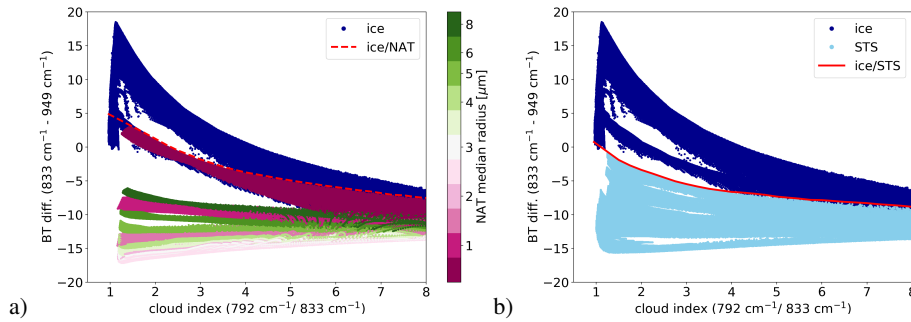
Figure 6. Correlation between the BT difference (832 – 834 cm -1 ) – (947.5 – 950.5 cm -1 ) and cloud index. The red solid line shows the separation line between ice and STS and the dashed line marks the separation between ice and NAT.
