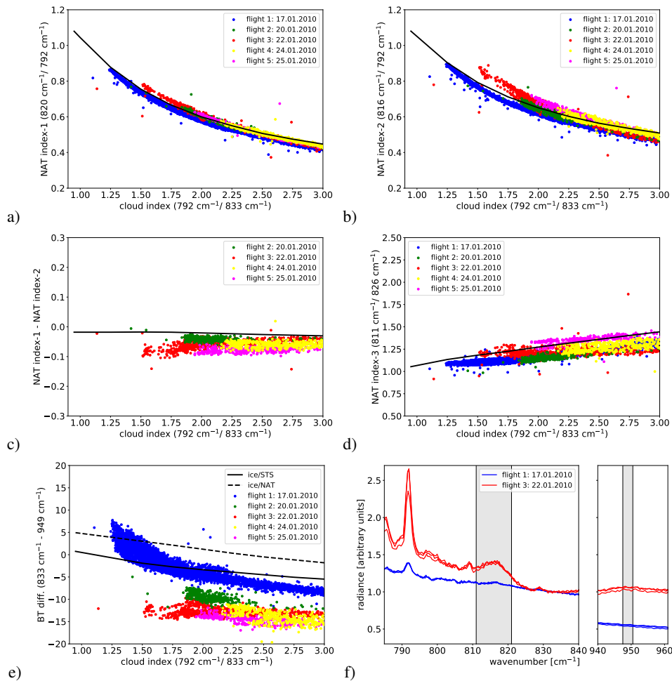
Figure 9. Correlations between the different NAT indices and cloud index for the CRISTA-NF observations during RECONCILE flights 1 – 5. a) NAT index-1 (819 – 821 cm -1 )/(791 – 793 cm -1 ) (MW3/MW1); b) NAT index-2 (815 – 817 cm -1 )/(791 – 793 cm -1 ) (MW4/MW1); c) NAT index-1 – NAT index-2; d) NAT index-3 (810 – 812 cm -1 )/(825 – 827 cm -1 ) (MW5/MW6). The black lines show the separation lines, which mark the upper envelope of the regions of STS and ice (in a), b), and d)) or the region of medium and large NAT (in c)). Simulation results for ice and STS are in shown in dark and light blue, respectively. e) Correlation between the BT difference (832 – 834 cm -1 ) – (947.5 – 950.5 cm -1 ) and cloud index for the CRISTA-NF observations during RECONCILE flights 1 – 5. The black solid line shows the separation line between ice and STS and the dashed line marks the separation between ice and NAT. f) Example spectra from flight 1 and flight 3 for ice and NAT PSC, respectively. The spectra have been scaled such that the radiance for all spectra equals 1 in the spectral window 832.0 – 834.0 cm -1 . The gray bars mark the region of the shifted NAT feature and the region used for the BTD around 949 cm -1 .
