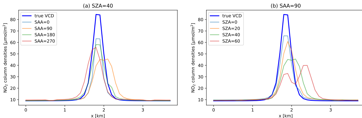
Figure 12. Plume VCD cross section at y=1.6 km (0.3 km downstream of the plume) for (a) the sun at SZA=40^\circ with different SAAs and (b) for the sun in the west with different SZAs
