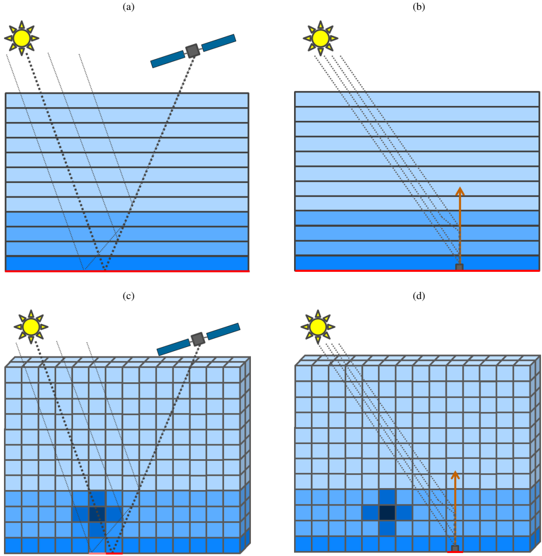
Figure 1. Illustration of the difference between 1D-layer (upper panels a,b) and 3D-box AMFs (lower panels c,d) for two scenarios with downward-looking spaceborne (left a,c) and upward-looking ground-based (right b,d) observations. Selected photon paths are shown as dashed lines. 1D-layer AMFs implicitly assume horizontally uniform atmospheric and surface properties, whereas 3D-box AMFs fully account for both vertical and horizontal variability.
