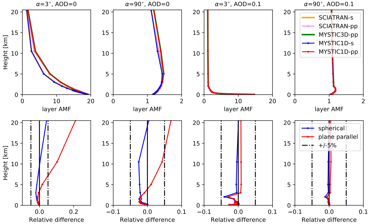
Figure 3. Upper row: MAX-DOAS AMF profiles for MYSTIC 1D spherical geometry (blues), 1D plane parallel geometry (redpp) and 3D plane parallel geometry (greenpp) for two selected elevation angles of 3^\circ and 90^\circ , a SZA of 20^\circ , with and without aerosol for radiation at 577 nm. Corresponding profiles computed with the SCIATRAN RTM are shown for comparison. Lower row: Profile of relative differences of MYSTIC and SCIATRAN results in spherical (blues) and plane parallel geometry (redpp) (Wagner et al., 2007).
