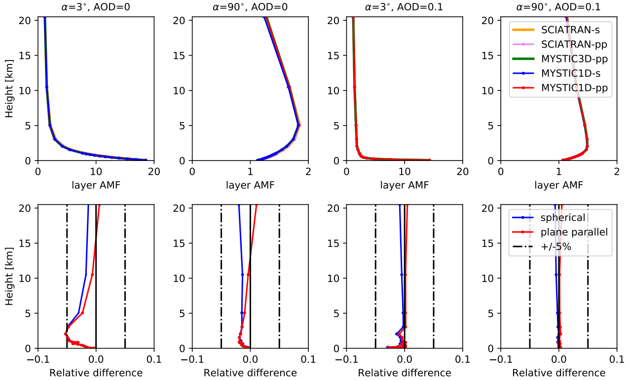
Figure 4. Upper row: MAX-DOAS AMF profiles for MYSTIC 1D spherical geometry (blue), 1D plane parallel geometry (red) and 3D plane parallel geometry (green) for two selected elevation angles of 3° and 90°, a SZA of 20°, with and without aerosol for radiation at 360 nm. Corresponding profiles computed with the SCIATRAN RTM are shown for comparison. Lower row: Profile of relative differences of MYSTIC and SCIATRAN results in spherical (blue) and plane parallel geometry (red) (Wagner et al., 2007).
