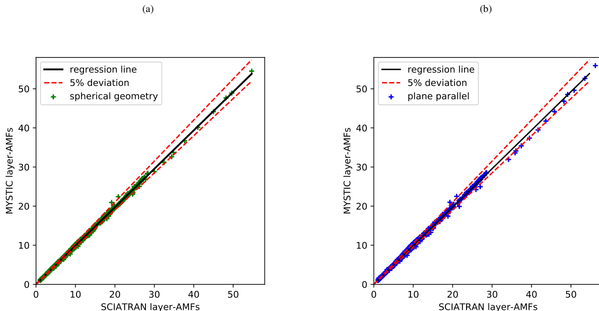
Figure 2. Scatter plots of MYSTIC 1D-layer AMFs computed with spherical (a) and plane parallel geometries (b) against 1D-layer AMFs computed with SCIATRAN spherical (a) and plane parallel (b) for 67 MAX-DOAS scenarios with 17 layers (1139 points). The solid black lines are the respective regression fits to the points.
