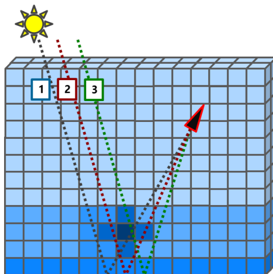
Figure 9. Schematic of the across-track measurement by the aircraft measuring a NO 2 plume (dark blue corresponding to high NO 2 concentrations) with 3 main photon paths for 3 measurement geometries (1, 2, 3).
