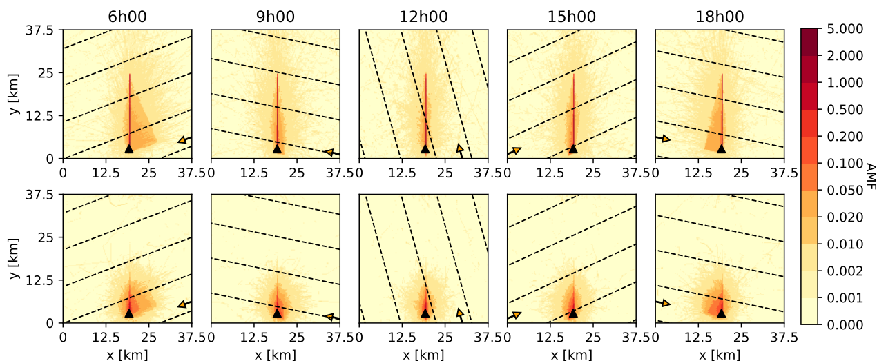
Figure 6. Top: Vertically integrated 3D-box AMFs in the boundary layer ( z < 2.0 km) for an instrument at the ground pointing northwards with an instrument zenith angle of 5^\circ for different times of the day on a 21st of June in Zurich. Solar zenith angles are 77.4^\circ , 47.5^\circ , 24.6^\circ , 38.6^\circ and 68.5^\circ and solar azimuth angles are 249.0^\circ , 281.5^\circ , 344.7^\circ , 65.2^\circ and 101.7^\circ . The arrows point away from the sun and the dashed lines show the direction of photons coming from the sun. AMFs were simulated with a rural type aerosol representative of spring-summer conditions in the aerosol layer (0-2 km) with a visibility of 50 km and a background aerosol above 2 km. Bottom: Same as above but for a scenario with increased aerosol (visibility of 10 km).
