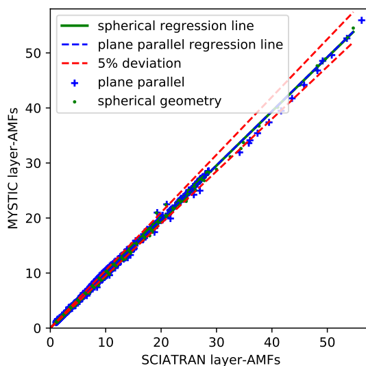
Figure 2. Scatter plot of MYSTIC 1D-layer AMFs computed with spherical (green dots) and plane parallel geometries (blue cross) against 1D-layer AMFs computed with SCIATRAN plane parallel and spherical for 67 scenarios with 17 layers (1139 points). The solid green line is the regression fit to the spherical geometry points and the dashed blue line is the regression to fit the plane parallel geometry points.
