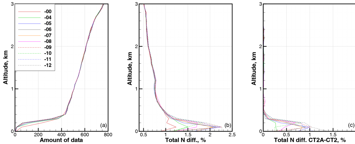
Figure 11. Statistics for latitude band 80–90°. (a) Amount of data. (b) RMS relative difference in refractivity COSMIC–ECMWF \Delta N_{CE} . (c) RMS relative difference in refractivity CT2A–CT2. All are functions of the parameter \beta .
