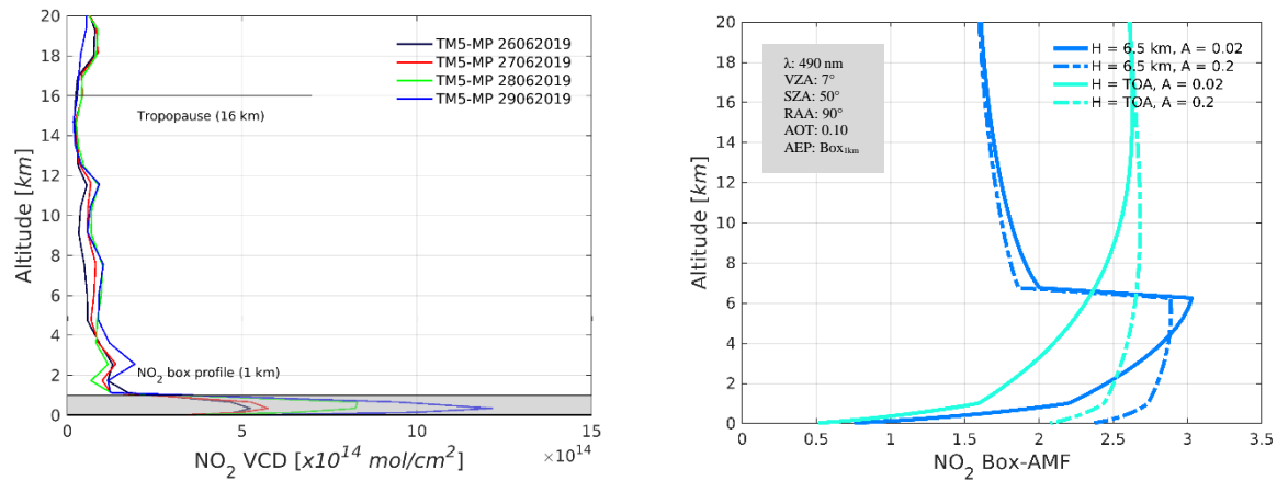
Figure 3. (a) Representation of a well-mixed NO 2 box profile of 1 km thickness and TM5-MP NO 2 profiles interpolated over the campaign sites for Flight #1 to #4, and (b) height-dependent box AMFs representing the vertical sensitivity to NO 2 , illustrated for APEX, operating at 6.5 km a.g.l., and TROPOMI, for both a low and high surface reflectance scenario.
