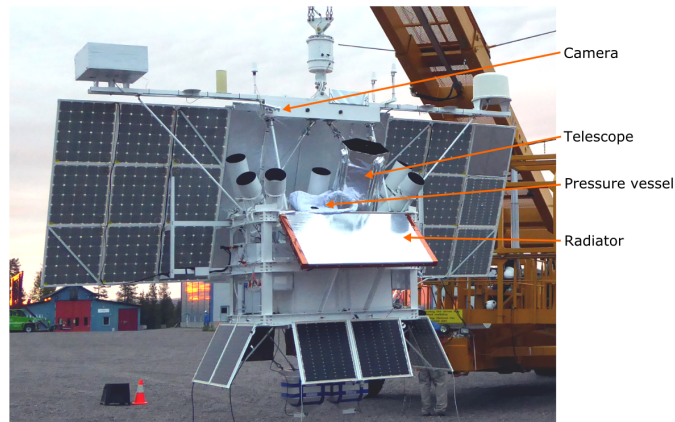
Figure 4. The PMC Turbo gondola during launch preparations on 6 July 2018.
