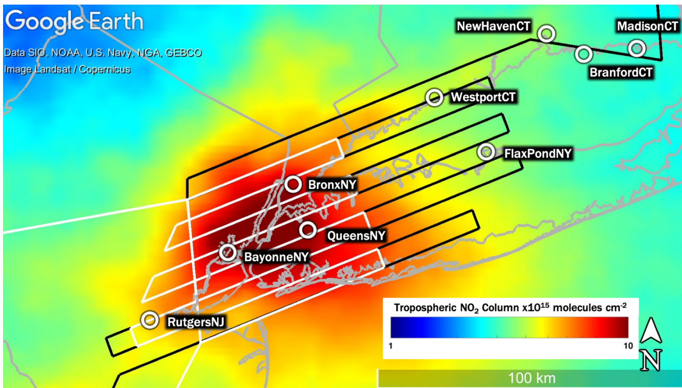
Figure 1: Map showing the annual average TROPOMI tropospheric NO 2 columns between April 2018-March 2019. Overlaid circles show the locations of the nine Pandora spectrometers considered in this analysis. Table 4 shows when each of these instruments operated. The black and white lines represent the two types of flight plans flown by the airborne spectrometers (large in black and small in white). This map was created in © Google Earth Pro.
