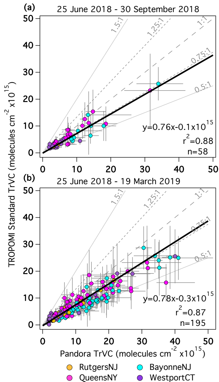
1305 Figure 12: TROPOMI Standard vs Pandora TrVCs colored by site during (a) the LISTOS intensive period for the four locations with extended measurements in time (RutgersNJ, BayonneNJ, QueensNY, WestportCT) followed by (b) coincidences extending from 25 June 2018 – 19 March 2019 at the same four sites. The horizontal bars represent the 10 th -90 th percentile of Pandora data within the \pm 30 min temporal window. The vertical bars represent the reported precision of TROPOMI. Each point is colored by Pandora location.
