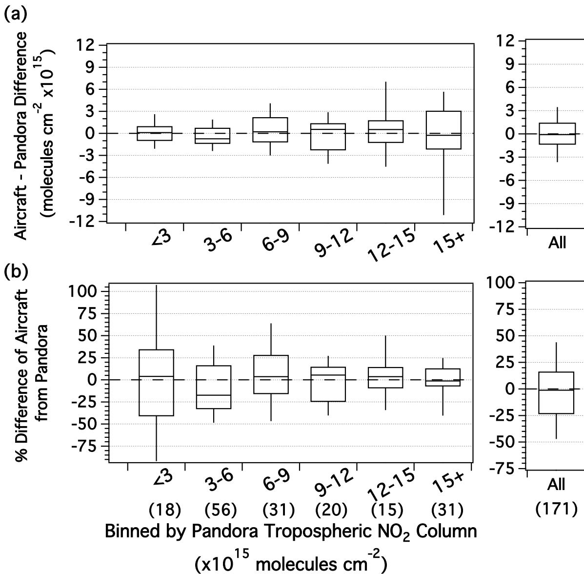
255 Figure 4: Box plots (95-75-50-25-5) showing the airborne column (a) column difference and (b) percent difference from Pandora binned at the labeled thresholds ( \times 10^{15} ) as well as all data points (right). The number of points in each bin are indicated by the numbers in parentheses above the x-axis label.
