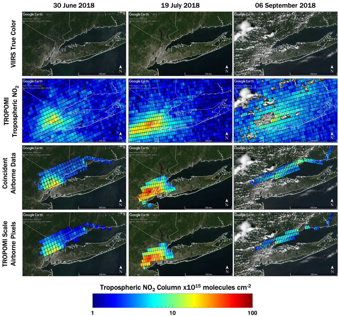
1260 Figure 5: Maps demonstrating how airborne data is matched to TROPOMI for 3 out of 15 example overpasses: (top) VIIRS true color imagery (source: https://worldview.earthdata.nasa.gov/ ; last accessed 18 April 2020), (second row) overlaid TROPOMI TrVCs where CRFs < 50%, (third row) overlaid airborne data collected within \pm 30 minutes of the TROPOMI overpass with outlined TROPOMI pixels with CRFs < 50% and area mapped by aircraft > 75%, (bottom) airborne NO 2 columns data scaled to the TROPOMI pixel. All maps were created in © Google Earth Pro.
