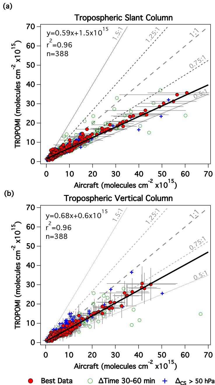
265 Figure 6: Scatter plots of airborne data gridded and scaled up to the TROPOMI pixel footprint vs. TROPOMI NO 2 tropospheric (a) slant column and (b) vertical column that are at least 75% mapped with a CRF < 50 % within ± 30 min of the TROPOMI overpass in red circles (open green circles show points when the time window is expanded to ± 60 min and blue crosses symbolize points where ΔCS > 50 hPa). The horizontal bars indicate the sub-pixel heterogeneity measured by the aircraft quantified as the standard deviation of aircraft slant columns over that pixel and vertical bars in (b) show the reported precision of the TROPOMI TrVC (the precision of the tropospheric slant columns in panel a are not large enough to be visible in this figure but the average is 5x10 14 molecules cm -2 with a standard deviation of 7x10 13 molecules cm -2 ).
