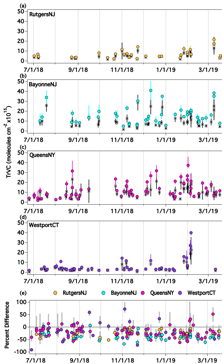
1300 Figure 11: Time series of Pandora and TROPOMI Standard TrVCs from 25 June 2018 through 19 March 2019. Circles represent the Pandora data \pm 10^{\text{th}}\text{-}90^{\text{th}} percentile in the \pm 30\text{-minute} window and the stars indicated the TROPOMI TrVC \pm the reported precision at (a) RutgersNJ, (b) BayonneNJ, (c) QueensNY, and (d) WestportCT. The percent difference of the TROPOMI Standard TrVC from Pandora colored by site is shown in (e) and the grey bars indicate the 10^{\text{th}}\text{-}90^{\text{th}} percentile of the column difference of TROPOMI TrVC from the sub-temporal Pandora data.
