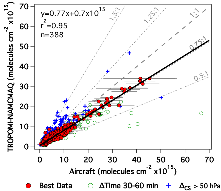
Figure 7: Scatter plots of airborne data gridded and scaled up to the TROPOMI pixel footprint vs. TROPOMI-NAMCMAQ \text{NO}_2 TrVCs that are at least 75% mapped with a CRF < 50 % within \pm 30 min of the TROPOMI overpass in red circles (open green circles show points when the time window is expanded to \pm 60 min and blue crosses symbolize points where \Delta\text{CS} > 50 hPa). The horizontal bars indicate the sub-pixel heterogeneity measured by the aircraft quantified as the standard deviation of aircraft vertical columns over that TROPOMI pixel.
