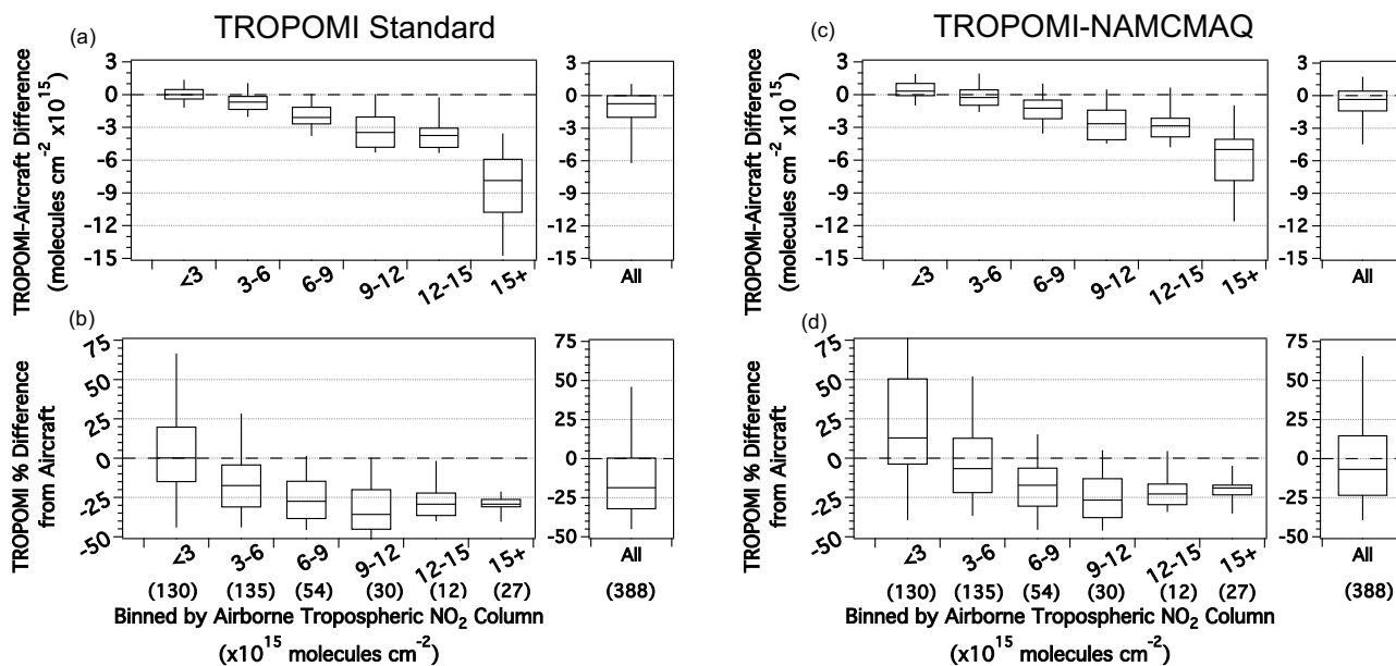
280 Figure 8: Box plots (95-75-50-25-5) showing the TROPOMI TrVC (a) column difference and (b) percent difference from airborne TrVCs binned at the labeled thresholds ( \times 10^{15} ) as well as for the total dataset (right), along with the equivalent box plots for TROPOMI-NAMCMAQ in (c) and (d). The number of points in each bin are indicated by the numbers in parentheses above the x-axis label.
