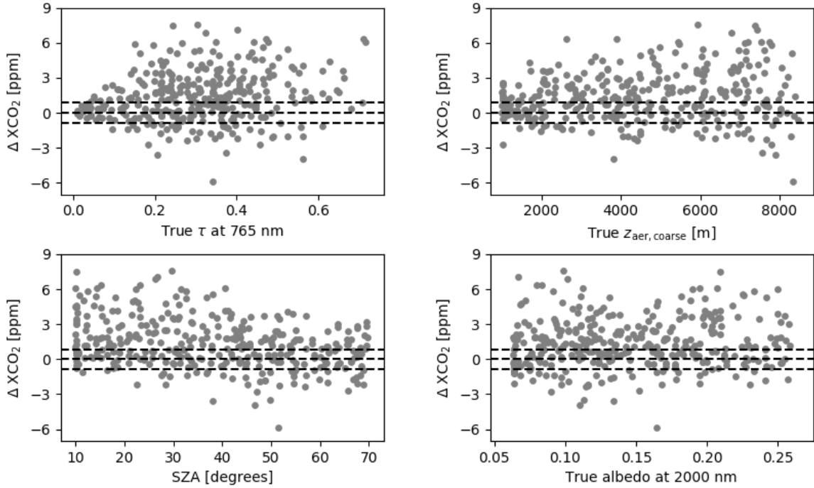
Figure 1. Residual \text{XCO}_2 from the converged retrievals using spectrometer measurements only, shown as a function of total aerosol optical depth \tau , coarse-mode aerosol height, SZA, and albedo. The input spectra are generated according to the ensemble of synthetic scenes (Section 4). The three dashed horizontal lines indicate \Delta\text{XCO}_2 at -0.86, 0, and 0.86 ppm.
