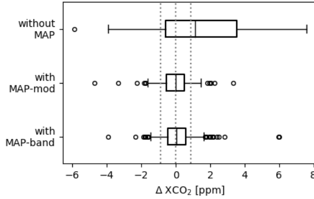
Figure 9. Boxplot of \Delta\text{XCO}_2 from retrievals on the synthetic scenes using 3-band spectrometer measurements only ('without MAP') versus those from retrievals using the combined MAP-mod and spectrometer data ('with MAP-mod'), and those from the combined MAP-band and spectrometer data ('with MAP-band') . The rectangles are outlined by the 15.9th and the 84.1th percentiles (P(15.9) and P(84.1)) with the 50th percentile (median) indicated by a vertical line inside the rectangles. The length of the whiskers are set to the difference between P(84.1) and P(15.9). The circles indicate retrievals with \Delta\text{XCO}_2 beyond the extent of the whiskers. The three dotted vertical lines mark -0.86, 0, and 0.86 ppm.
