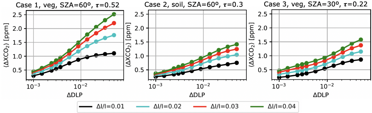
Figure 2. \langle \Delta XCO_2 \rangle as a function of \Delta I/I and \Delta DLP , shown for scenarios where the errors are among the largest for each individual case 1, 2, and 3. Here, \tau indicates the sum of the fine- and the coarse-mode aerosol optical depth at 765 nm.
