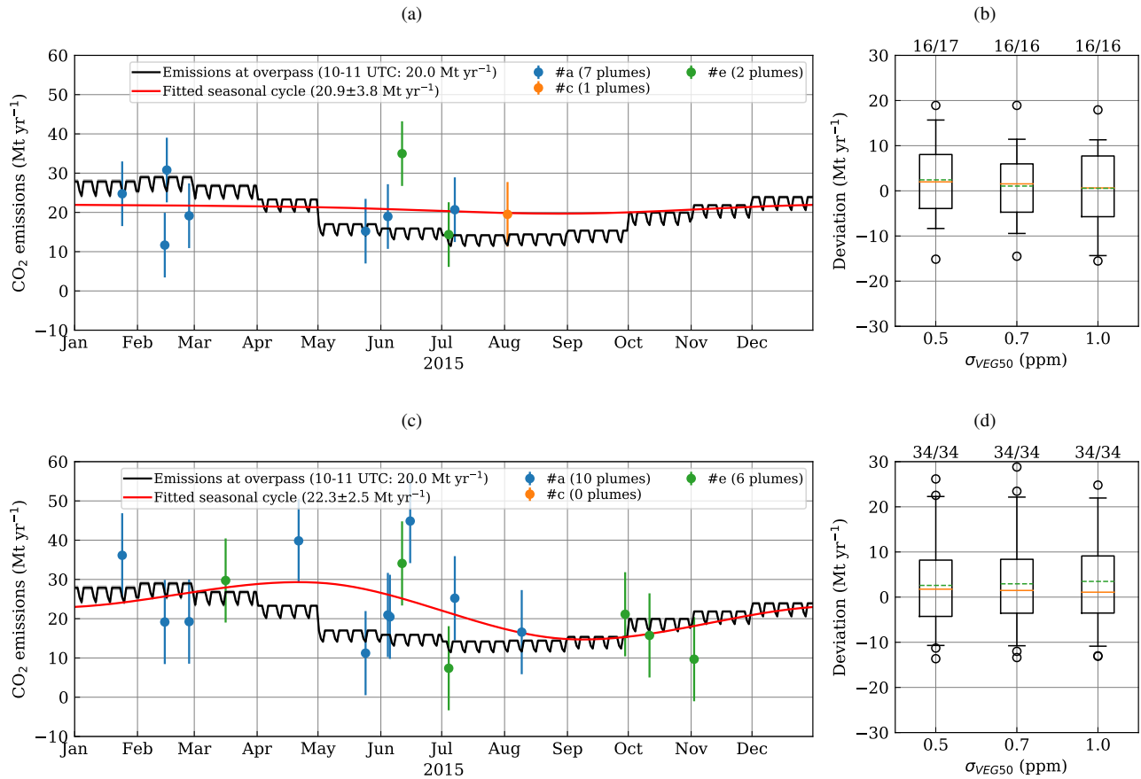
Figure 7. Time series of estimated CO 2 emissions of Berlin using a constellation of three satellites (#a, #c and #e) with medium noise instruments ( \sigma_{VEG50} = 0.7 ppm). The plumes were detected from (a) the CO 2 and (c) the NO 2 observations. The error bars show constant errors of 10.0 \text{ Mt yr}^{-1} corresponding to the standard deviation of the differences between estimated and real emissions. (b, d) The boxplots show the difference between estimated and CO 2 emissions at overpass of Berlin for six satellites. The boxes denote the range between 25th and 75th percentiles, orange lines are median values, and whiskers are 5th and 95th percentiles. The numbers above the boxes are the number of cases for which emissions could be estimated for all three scenarios (first number) and the number of successful emission estimates for each scenario (second number).
