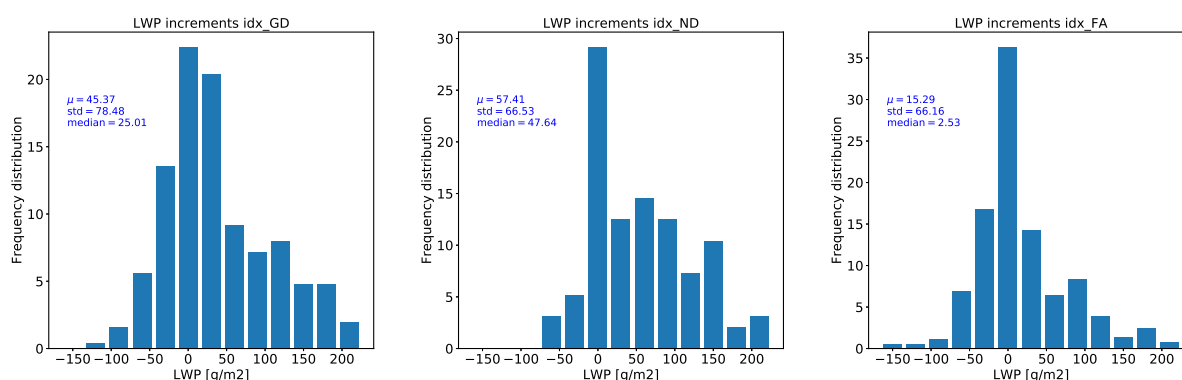
Figure 10. Frequency distribution of 1D-Var LWP increments ( \text{g}\cdot\text{m}^{-2} ). Statistics performed over 255 profiles of good fog detection (left panel), 95 profiles of undetected fog (middle panel) and 368 profiles of false alarms (right panel).
