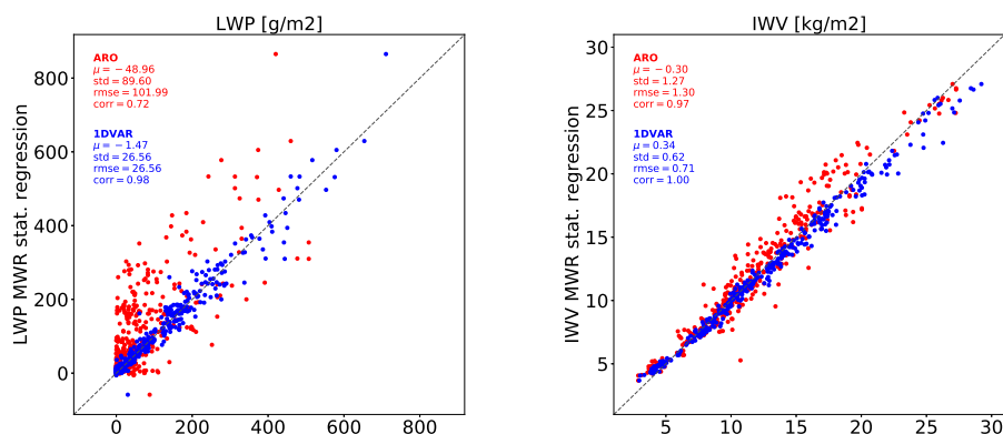
Figure 12. Scatterplot between a multi-channel regression based on MWR observations (y-axis) and the background forecast by AROME (red dots) or the 1D-Var analysis (blue dots) for LWP (left panel) and IWV (right panel). Statistics performed over 351 observed fog profiles.
