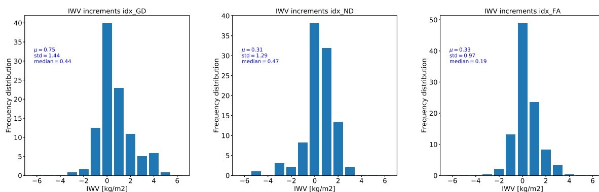
Figure 11. Frequency distribution of 1D-Var IWV increments ( \text{kg}\cdot\text{m}^{-2} ). Statistics performed over 255 profiles of good fog detection (left panel), 95 profiles of undetected fog (middle panel) and 368 profiles of false alarms (right panel).
