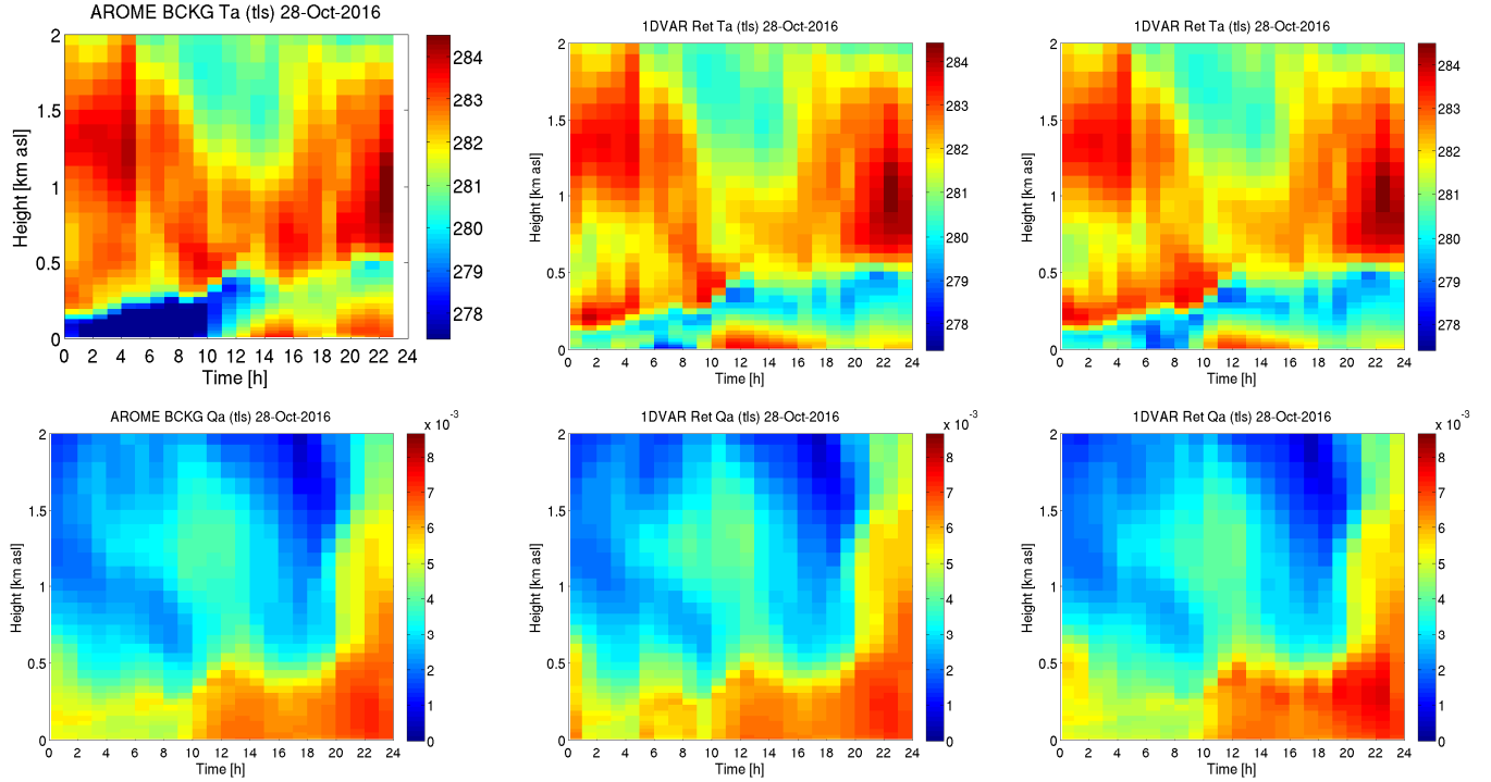
Figure 5. Time series of temperature profiles (top panels) and specific humidity (bottom panels) forecast by AROME (left panels) and retrieved with the 1D-Var scheme either using the optimal configuration (Config3, middle panels) or the worst one (CTRL, right panels). 28 October 2016.
