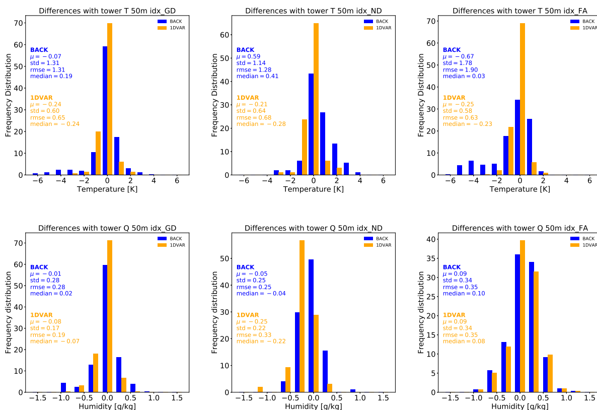
Figure 8. Frequency distribution of 1D-Var analyses (orange) and background (blue) differences with tower measurements for temperature (top panel) and specific humidity (bottom panel) at 50 m altitude. Statistics performed over 255 profiles of good fog detection (left panel), 95 profiles of undetected fog (middle panel) and 368 profiles of false alarms (right panel).
