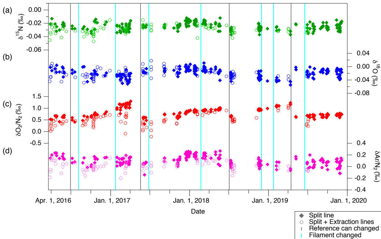
Figure 6: Standard gas (STDA) composition measured against reference gas for (a) \delta^{15}\text{N} , (b) \delta^{18}\text{O} , (c) \delta\text{O}_2/\text{N}_2 , and (d) \delta\text{Ar}/\text{N}_2 . Filled markers represent samples transferred only through the split line, and open markers represent samples transferred through both extraction and split lines. Vertical grey lines indicate the timing of replacements of reference can, and vertical light blue lines indicate the timing of filament replacements.
