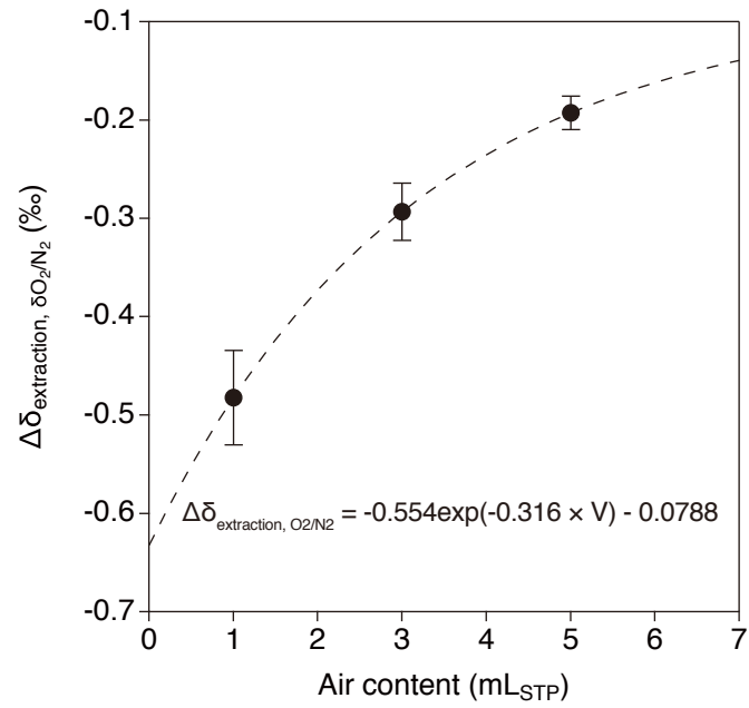
Figure 7: Change of \delta_{\text{O}_2/\text{N}_2} by wet extraction and overnight storage. Dashed line represents exponential fit to the data ( \Delta \bar{\delta}_{\text{extraction, O}_2/\text{N}_2} = -0.554 \exp(-0.316 \times V) - 0.0788 ).
