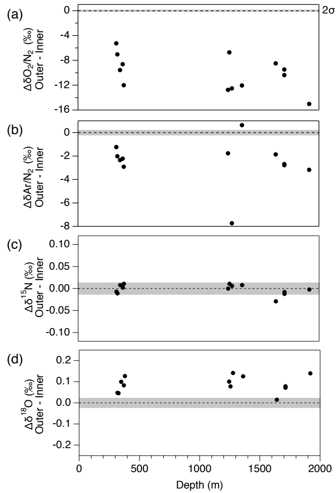
Figure 13: Pair difference ( \Delta ) between outer ice and inner ice for (a) \delta\text{O}_2/\text{N}_2 , (b) \delta\text{Ar}/\text{N}_2 , (c) \delta^{15}\text{N} , and (d) \delta^{18}\text{O} . Grey shadings indicate the estimated 2\sigma uncertainty for clathrate ice (from pooled standard deviations of duplicates with > 8 mm of outer removal).
