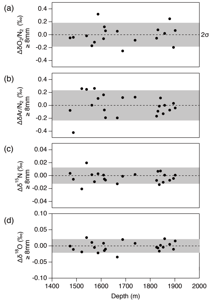
1090 Figure 15: Pair difference between the two inner ice pieces (data from “b” piece minus that from “a” piece) whose outer parts are removed by 8 mm or more for (a) \delta\text{O}_2/\text{N}_2 , (b) \delta\text{Ar}/\text{N}_2 , (c) \delta^{15}\text{N} , and (d) \delta^{18}\text{O} . Grey shadings indicate the estimated 2\sigma uncertainty for clathrate ice (from pooled standard deviations of duplicates).
