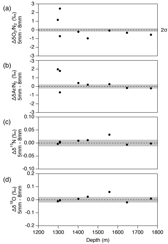
1085 Figure 14: Pair difference between the two inner ice pieces with the thickness of outer removal of 5 mm and 8 mm for (a) \delta^{O_2/N_2} , (b) \delta^{Ar/N_2} , (c) \delta^{15N} , and (d) \delta^{18O} . Grey shadings indicate the estimated 2\sigma uncertainty for clathrate ice (from pooled standard deviations of duplicates with > 8 mm of outer removal).
