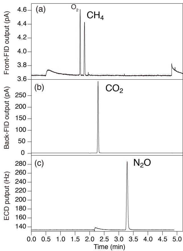
1040 Figure 4: Typical chromatogram of (a) Front FID for CH_4 (the largest peak is O_2 , and the second-largest peak is CH_4 ), (b) Back FID for CO_2 , and (c) ECD for N_2O .
