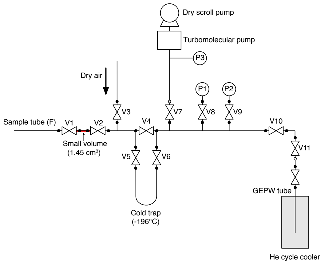
1035 Figure 2: Schematic diagram of the split line.
