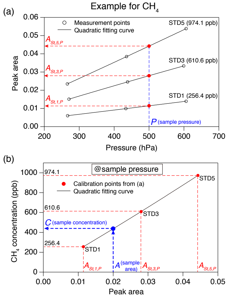
1045 Figure 5: Example of a calibration procedure for greenhouse gas concentration. (a) Peak areas for three standard gases measured at three pressures (black circles), with quadratic fits (black lines). Peak areas of the standard gases ( A_{St,1,P} , A_{St,3,P} , and A_{St,5,P} , red circles) estimated at the sample pressure (blue dashed line) are also shown. (b) Calibration curve at the sample pressure (black line) from the peak areas from (a). The numbers in the panel are CH 4 concentrations of the standard gases, A is the peak area of the sample, and C is the CH 4 concentration of the sample.
