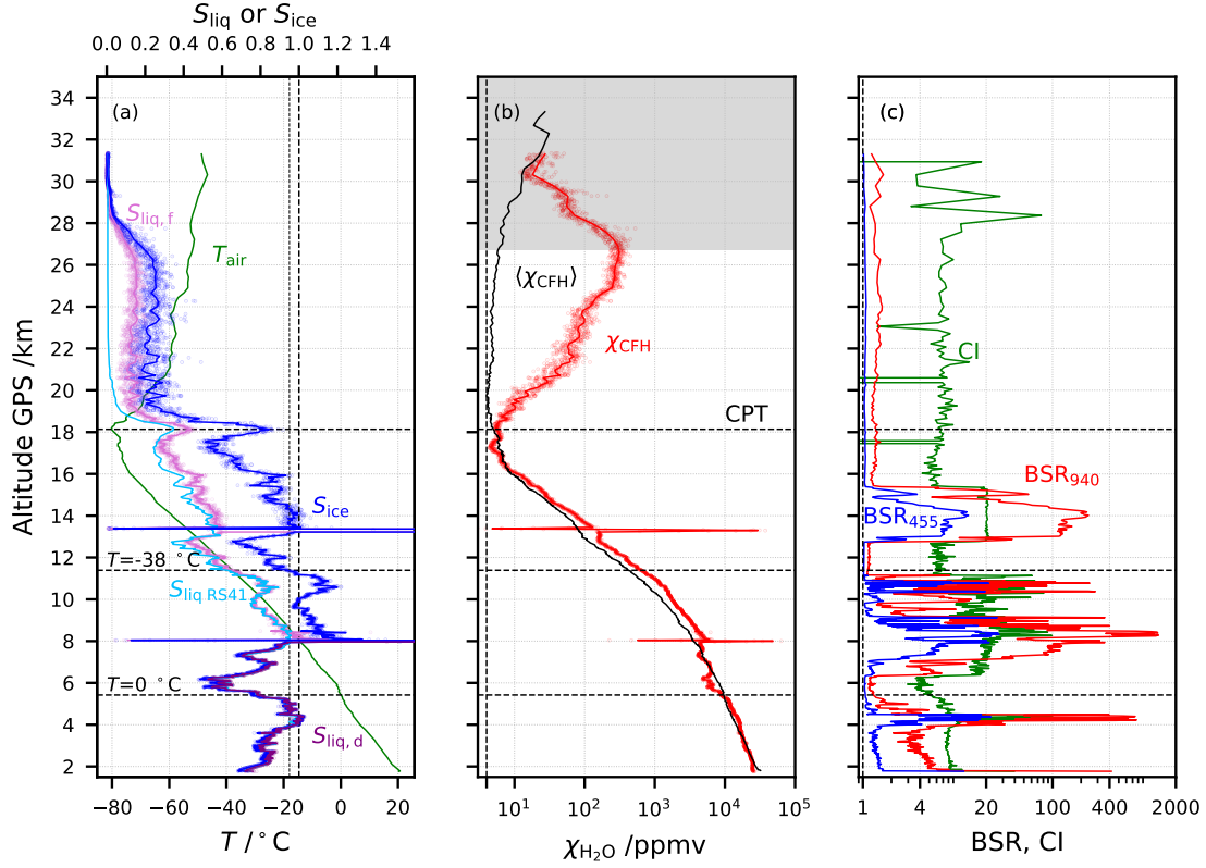
Figure 1: Flight NT029 in Nainital, India, on 30 August 2016. Lines: 1 hPa interval averaged values. Dots: 1 s data. (a) Green: air temperature measurement from the Vaisala RS41; light blue: relative humidity ( S_{\text{liq, RS41}} ) by the RS41; blue: ice saturation ( S_{\text{ice}} ) from the CFH; purple: saturation over water ( S_{\text{liq, d}} ) from the CFH considering the deposit on the mirror to be dew; pink: saturation over water ( S_{\text{liq, f}} ) from the CFH considering the deposit on the mirror to be frost. Note that the condensate on the CFH mirror was forced to turn from dew to frost after the freezing cycle, at T_{\text{frost}} = -15 °C. (b) Red: \text{H}_2\text{O} mixing ratio from the CFH in ppmv; black: season average \text{H}_2\text{O} mixing ratio excluding contaminated CFH profiles for the Nainital 2016 summer campaign (Brunamonti et al., 2018). Highlighted values with grey shading above the 20-hPa level are possibly contaminated by out gassing from the balloon envelope. ‘CPT’ marks the cold point tropopause. (c) Red: 940-nm backscatter ratio from the COBALD; blue: same for 455 nm; green: color index (CI) from the COBALD.
