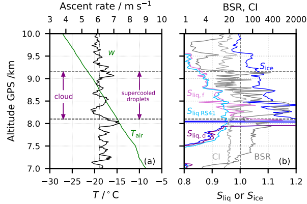
Figure 2: Mixed-phase cloud detail of flight NT029. Lines: 1 hPa interval averaged values. (a) Green: air temperature; black: ascent velocity measured by the RS41 in \text{m s}^{-1} . (b) Light blue: saturation over water ( S_{\text{liq, RS41}} ) measured by the RS41; purple: saturation over water ( S_{\text{liq,d}} ) from the CFH considering the deposit on the mirror to be dew; pink: saturation over water ( S_{\text{liq,f}} ) from the CFH considering the deposit on the mirror to be frost; blue: ice saturation ( S_{\text{ice}} ) from the CFH; dark grey: 940-nm backscatter ratio from the COBALD; light grey: color index (CI) from the COBALD. Horizontal dashed lines mark supercooled droplet region.
