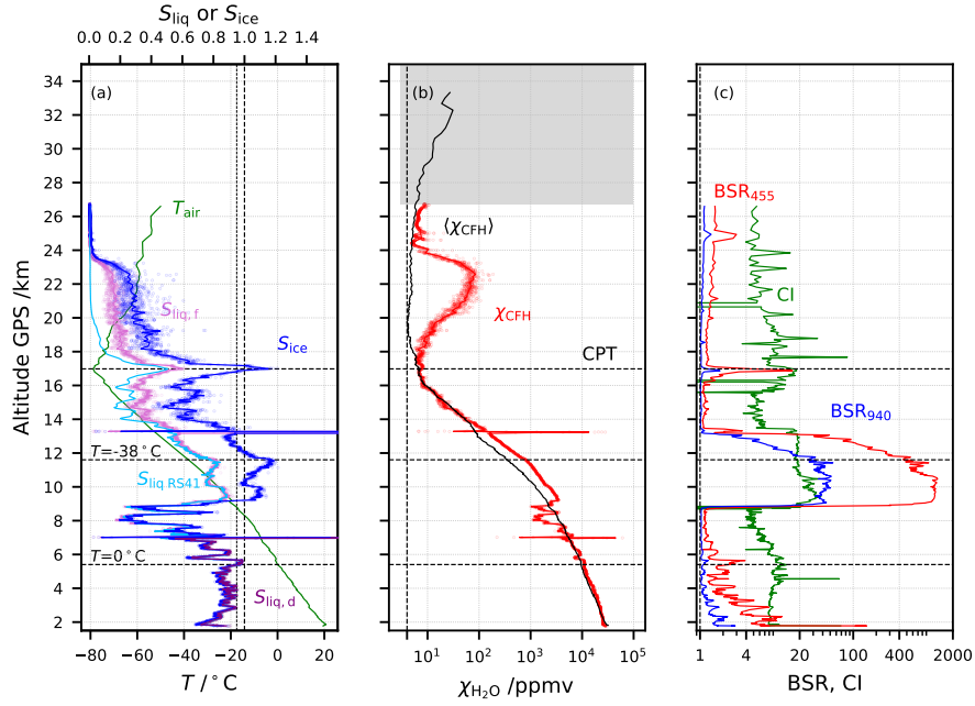
Figure 2. Flight NT011 in Nainital, India, on 15 August 2016. Lines: 1 hPa interval averaged values. Dots: 1 s data. (a) Green: air temperature from the Vaisala RS41; light blue : saturation over water ( S_{\text{liq, RS41}} ) measured by the RS41; blue: ice saturation ( S_{\text{ice}} ) from the CFH, purple : saturation over water ( S_{\text{liq, d}} ) from the CFH considering the deposit on the mirror to be dew; pink : saturation over water ( S_{\text{liq, f}} ) from the CFH considering the deposit on the mirror to be frost. Note that the condensate on the CFH mirror was forced to turn from dew to frost after the freezing cycle, at T_{\text{frost}} = -15^\circ\text{C} . (b) Red: \text{H}_2\text{O} mixing ratio from the CFH in ppmv; black: season average \text{H}_2\text{O} mixing ratio excluding contaminated CFH profiles for the Nainital 2016 summer campaign (Brunamonti et al., 2018). Highlighted values with grey shading above the 20-hPa level are possibly contaminated by out gassing from the balloon envelope. ‘CPT’ marks the cold point tropopause. (c) Red: 940-nm backscatter ratio from the COBALD; blue: same for 455 nm; green: color index (CI) from the COBALD.
