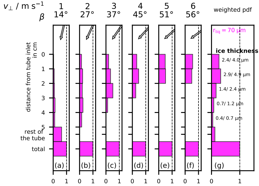
Figure 15: Collision/freezing efficiency of hydrometeors in the intake tube for mixed-phase cloud 2 of flight NT007 with average vertical inlet velocity w_{\parallel} = 4.0 \text{ m s}^{-1} . r_{liq} = 70 \mu\text{m} (pink). (a-f) Freezing efficiency for various velocities ( v_{\perp} ) perpendicular to the tube walls: (a) 1 \text{ m s}^{-1} , 14^{\circ} ; (b) 2 \text{ m s}^{-1} , 27^{\circ} ; (c) 3 \text{ m s}^{-1} , 37^{\circ} ; (d) 4 \text{ m s}^{-1} , 45^{\circ} ; (e) 5 \text{ m s}^{-1} , 51^{\circ} ; (f) 6 \text{ m s}^{-1} , 56^{\circ} . The 'rest of the tube' takes account of all collisions occurring deeper than 5 cm inside the tube, including the mirror holder. (g) Weighted sum of the efficiencies in panels (a-f) by the horizontal velocity pdf of Figure 13d, in front of each bar we write the thickness of the subsequent ice layer considering radial homogeneous cover of the intake tube and the lower (left) and upper (right) LWC estimate for the cloud.
