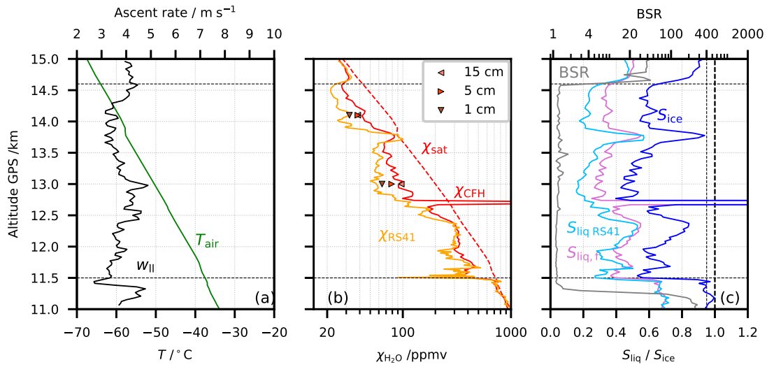
Figure 17: Flight NT007 and FLUENT simulation results for sublimation in the upper troposphere. (a) Green: air temperature; black: ascent velocity. (b) Red: \text{H}_2\text{O} mixing ratio by the CFH; orange: \text{H}_2\text{O} mixing ratio RS41; dashed red: saturation \text{H}_2\text{O} mixing ratio for the air temperature; symbols: FLUENT simulation results for the tube average mixing ratios \langle \chi_{\text{H}_2\text{O}} \rangle_{\text{vol}} in tubes with different ice coating depths d (full circumference): \blacktriangleleft d = 15 cm; \blacktriangleright d = 5 cm; \blacktriangledown d = 1 cm; (c) Light blue: saturation over water ( S_{\text{liq RS41}} ) by the RS41; pink: saturation over water ( S_{\text{liq f}} ) from the CFH considering the deposit on the mirror to be frost; blue: ice saturation ( S_{\text{ice}} ) from the CFH; grey: 940-nm backscatter ratio from the COBALD. Horizontal dashed lines limit the integration interval used for estimating the sublimated ice in the upper troposphere.
