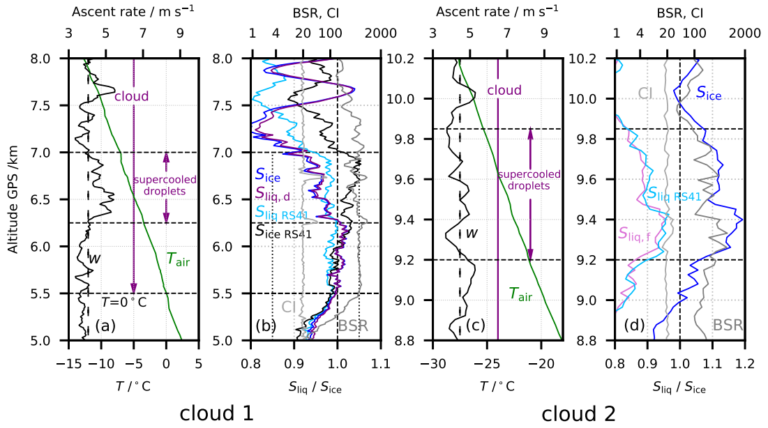
Figure 10: Mixed-phase cloud details of flight NT007. Lines: 1 hPa interval averaged values. (a-b) Cloud 1; (c-d) cloud 2. (a and c) Green: air temperature; black: ascent velocity by the RS41 in \text{m s}^{-1} . (b and d) Light blue: saturation over water ( S_{\text{liq, RS41}} ) by the RS41; purple: saturation over water ( S_{\text{liq, d}} ) from the CFH considering the deposit on the mirror to be dew; pink: saturation over water ( S_{\text{liq, f}} ) from the CFH considering the deposit on the mirror to be frost; blue: ice saturation ( S_{\text{ice}} ) from the CFH; black: ice saturation ( S_{\text{ice, RS41}} ) from the RS41; dark grey: 940-nm backscatter ratio from the COBALD; light grey: color index (CI) from the COBALD. Horizontal dashed lines mark supercooled droplet region and T_{\text{air}} = 0^\circ\text{C} .
