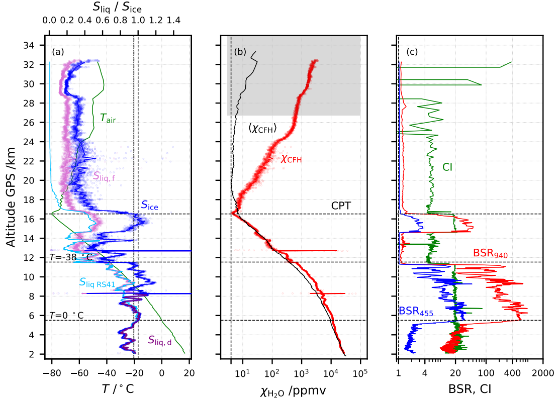
Figure 9: Flight NT007 in Nainital, India, on 11 August 2016. Lines: 1 hPa interval averaged values. Dots: 1 s data. (a) Green: air temperature measurement from the Vaisala RS41; light blue: saturation over water ( S_{\text{liq, RS41}} ) measured by the RS41; blue: ice saturation ( S_{\text{ice}} ) from the CFH; purple: saturation over water ( S_{\text{liq, d}} ) from the CFH considering the deposit on the mirror to be dew; pink: saturation over water ( S_{\text{liq, f}} ) from the CFH considering the deposit on the mirror to be frost. Note that the condensate on the CFH mirror was forced to turn from dew to frost after the freezing cycle, at T_{\text{frost}} = -15^\circ\text{C} . (b) Red: \text{H}_2\text{O} mixing ratio from the CFH in ppmv; black: season average \text{H}_2\text{O} mixing ratio excluding contaminated CFH profiles for the Nainital 2016 summer campaign (Brunamonti et al., 2018). Highlighted values with grey shading above the 20-hPa level are possibly contaminated by out gassing from the balloon envelope. ‘CPT’ marks the cold point tropopause. (c) Red: 940-nm backscatter ratio from the COBALD; blue: same for 455 nm; green: color index (CI) from the COBALD.
