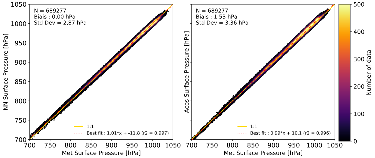
585 Figure 1: Density histogram of the surface pressure retrieved from the OCO-2 satellite measurements against that derived from GEOS-FP-IT. The left figure is for the NN approach while the right figure is for the ACOS v9r retrieval (using the official bias-correction). The figure insets provide the number of data points, the bias, the standard deviation, the equation of the best linear fit and the correlation. The yellow line is the 1:1 line whereas the red dotted line is the best linear fit.
