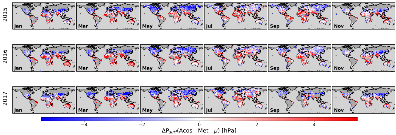
655 Figure A3: Same as Figure 5 but for the surface pressure retrieved by the ACOS algorithm. The mean bias over the full period ( \mu ) is removed so that the differences are centered on zero.
