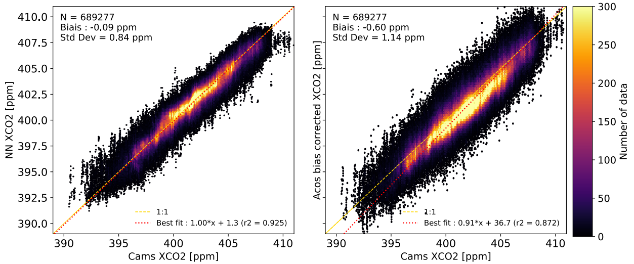
590 Figure 2: Same as Figure 1 but for XCO2. In this case, the reference data is the CAMS v18r2 simulation.
