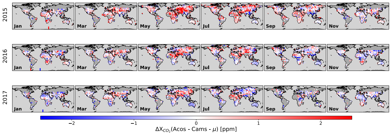
660 Figure A4: Same as Figure 7 but for the XCO2 retrieved by the ACOS algorithm. The mean bias over the full period ( \mu ) is removed so that the differences are centered on zero.
