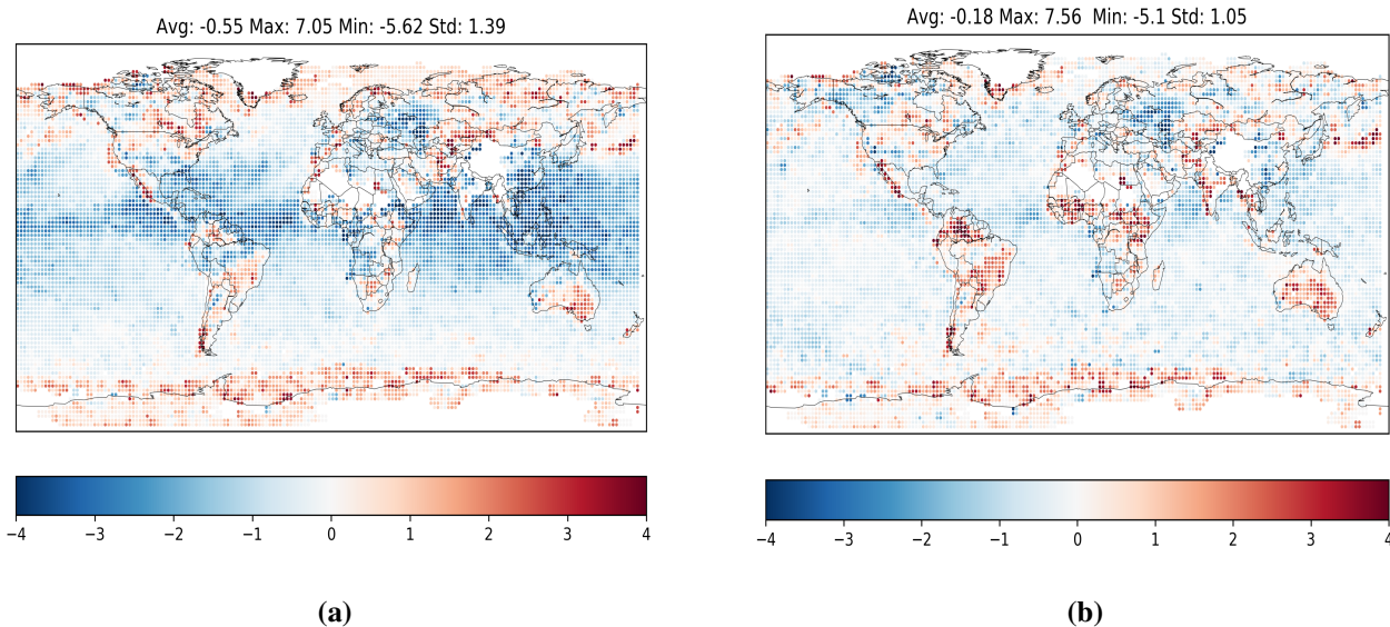
Figure 4. Difference ( in °C ) between the IFS SST forecast and the analysis of the SST given by RdiagExp (with a diagonal matrix) (a), and that given by RfullExp (with a correlated matrix) (b) averaged by box of 2°.
