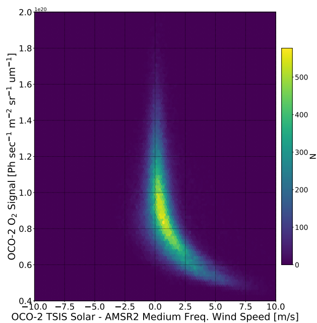
Figure 3. Heatmap of OCO-2 O 2 A-band signal compared to wind speed difference (OCO-2 TSIS solar - AMSR2 medium freq.)
