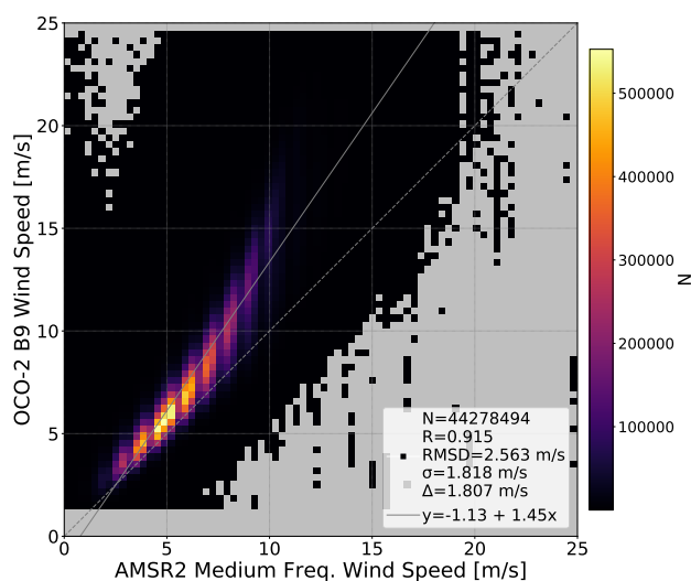
Figure 1. Heatmap of OCO-2 B9 wind speed compared to AMSR2 medium frequency wind speed. The B9 lite file quality flag has been applied, along with a height scaling.
