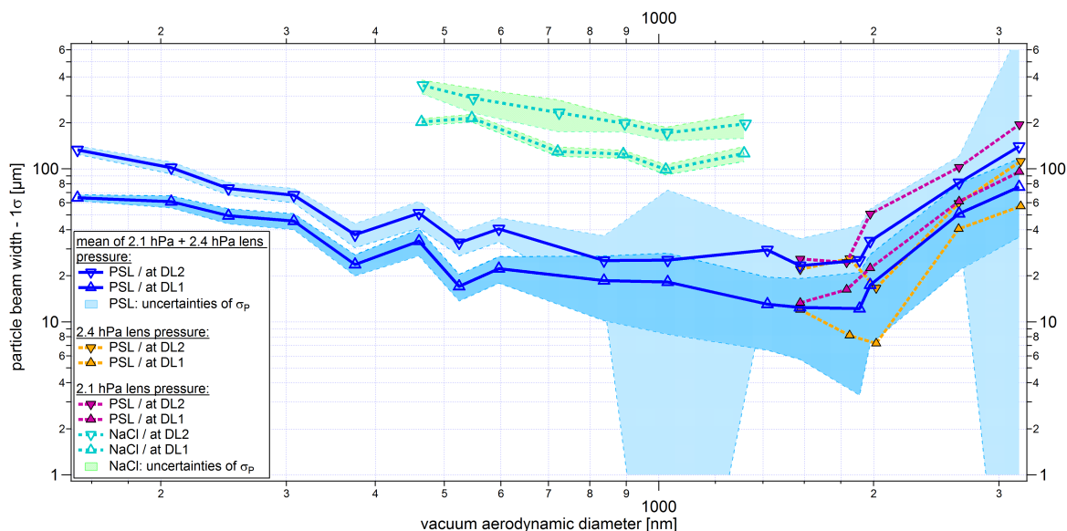
Figure 14. Size-resolved particle beam widths (one \sigma_P ), as defined in Eq. 4, at the two detection stages (DL1 and DL2) for PSL and NaCl particles. Below 1600 nm, the beam widths are averaged for 2.1 hPa and 2.4 hPa lens pressure (PSL only). The y-uncertainty range is given by the uncertainty of the fit of each scan (see Sect. 4.2.2). The x-uncertainty bars correspond to the standard deviation of the particle size distribution per particle size, particle type and lens pressure measured with the ALABAMA, converted into d_{va} according to Eq. S1 (Supplement).
