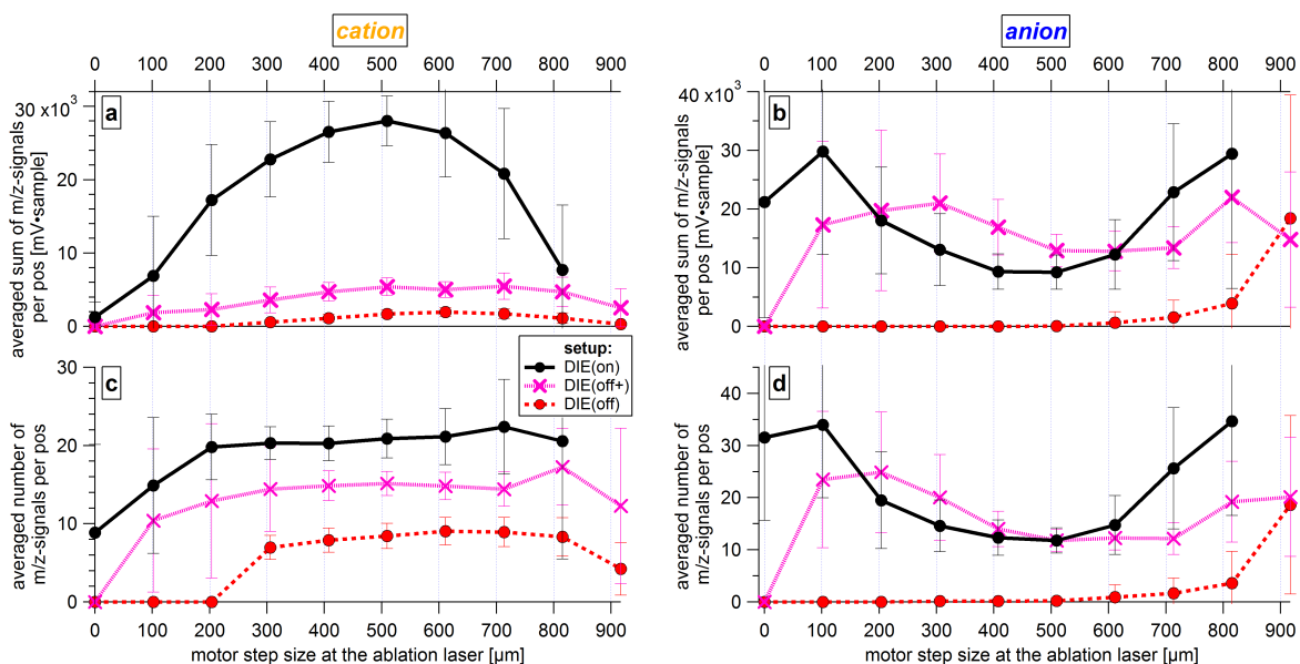
Figure 21. Dependence of mass spectral information on particle beam position along the cross section of the ablation laser’s beam path and the applied ion extraction field setup using 1029 nm ( d_{va} ) PSL particles. Panel a) and b) represent the averaged signal intensities of the mass spectra per scan position. Panel c) and d) represent the averaged number of m/z-signals of the mass spectra per scan position. Measurements were performed with laser energies between 4.8 mJ and 5.4 mJ and with the DMA that selected particle charge number of z = 1 . PSL particles of 1029 nm ( d_{va} ) result in a particle beam width as diameter of about 150 \mu\text{m} for 4\sigma (= 95 % of particles) at the ablation point and in an effective ablation laser beam width of about 500 \mu\text{m} . The uncertainty bars correspond to the standard deviation of the number and sum of the m/z-signals of the mass spectra per position.
