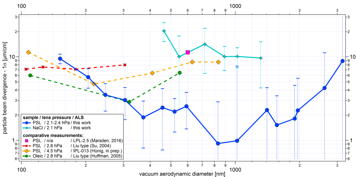
Figure 16. Comparison of size-resolved particle beam divergences for different ALS. The particle beam divergence for the ALABAMA was calculated from the particle beam width (one \sigma_D ) at both detection units and their distance from each other. The same approach was used in Hünig (in prep.) and Marsden et al. (2016). For Huffman et al. (2005) and Su et al. (2004) the distance from the exit of the ALS to the vaporizer was used to determine the particle beam divergence, assuming that the particle beam has no broadening at the center point of the exit of the ALS. However, there is a finite radius of the particle beam at the exit of the ALS, as mentioned in Cziczko et al. (2006) and confirmed by our study. Sphericity is assumed for PSL and oleic acid particles, and a cubic shape for NaCl particles. The results of Su et al. (2004) are shown considering a particle density for PSL of 1.05 \text{ g cm}^{-3} . The y-uncertainty range is given by the uncertainty of the fit of each scan (see Sect. 4.2.2) and Gaussian error propagation. The x-uncertainty bars correspond to the standard deviation of the particle size distribution per particle size, particle type and lens pressure measured with the ALABAMA, converted into d_{va} according to Eq. S1 (Supplement).
