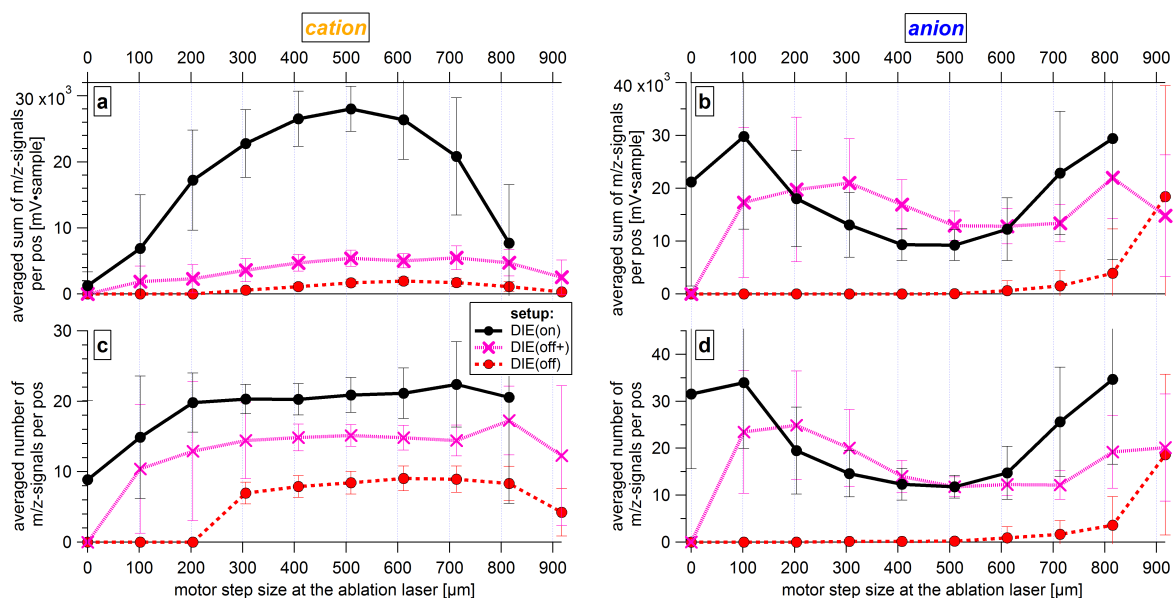
Figure 21. Mass spectral information in dependence of the particle beam position along the cross section of the ablation laser’s beam path and the applied ion extraction field setup using 1029 nm ( d_{va} ) PSL particles. Panel a) and b) represent the averaged signal intensities of the mass spectra per scan position. Panel c) and d) represent the averaged number of m/z-signals of the mass spectra per scan position. Measurements were performed with laser energies between 4.8 mJ and 5.4 mJ and with the DMA that selected particle charge number of z = 1 . PSL particles of 1029 nm ( d_{va} ) result in a particle beam width of about 150 \mu\text{m} for 4\sigma (= 95 % of particles) at the ablation point and in an effective ablation laser beam width of about 500 \mu\text{m} . The uncertainty bars correspond to the standard deviation of the number and sum of the m/z-signals of the mass spectra per position.
