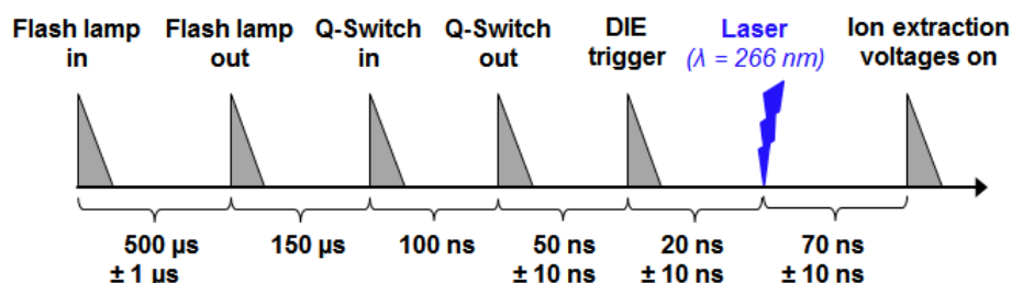
Figure 7. Time diagram of the trigger signals of the ablation laser, the laser pulse and the time-controlled switching process of the high voltages at the first electrodes (modified after Brands, 2009). Flash lamp in: trigger signal for the flash lamp in the laser; Flash lamp out: actual triggering of the flash lamp; Q-Switch in: trigger signal for the Q-Switch of the laser; Q-Switch out: actual triggering of the Q-Switch; DIE trigger: trigger signal for the HTS. The triangles shown in the figure were only used for better visualization and do not represent the decay times of the signals. The uncertainty values correspond to the reading accuracy at the oscilloscope.
