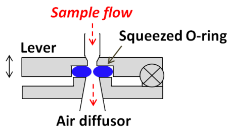
Figure 4. Schematic drawing of the constant pressure inlet (CPI) used in the ALABAMA. The double arrow on the lever indicates the possible directions of movement for squeezing the O-ring. The desired position of the lever is reached by means of a motor, which operates in dependency of the set lens pressure and the ambient sample air pressure.
