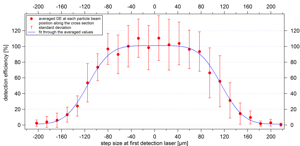
Figure 12. Lens scan along the cross section of the first detection laser using the example of 400 nm PSL particles. The averaged values of the DE, as well as the associated standard deviations (given as the uncertainties), result from a measurement time of about 5–10 seconds per particle beam position and from seven adjacent paths. The zero position on the x-axis corresponds to the laser beam center point in z-direction.
