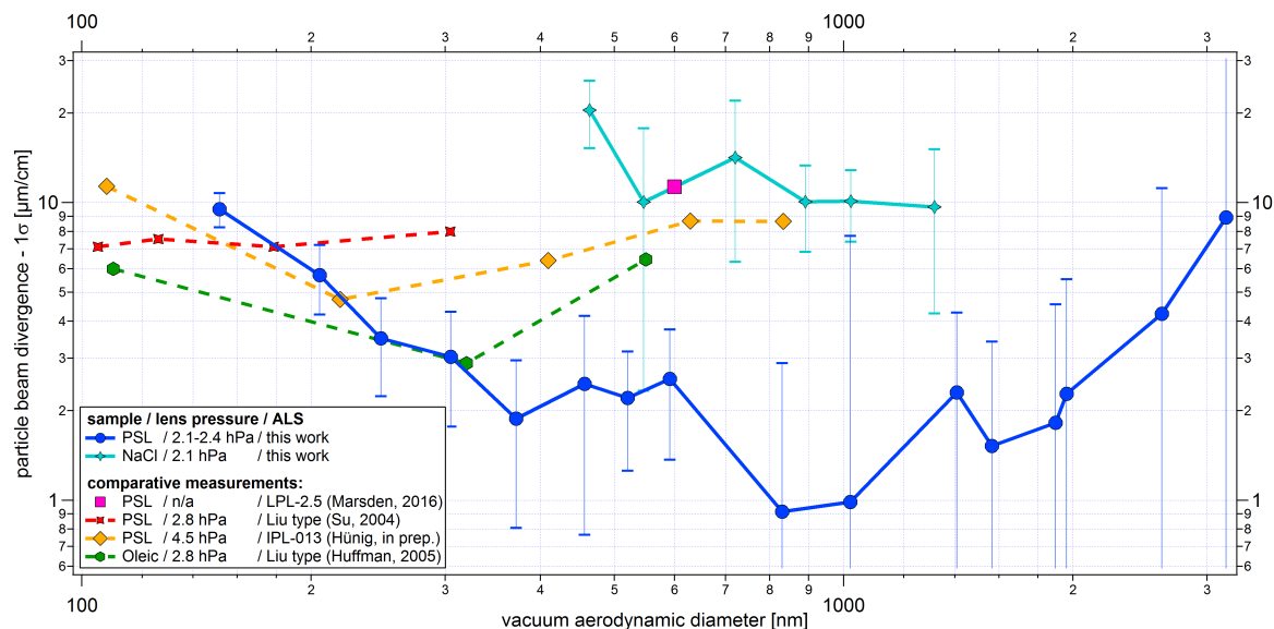
Figure 16. Comparison of size-resolved particle beam divergences for different ALS. The particle beam divergence for the ALABAMA was calculated from the particle beam width ( 1\sigma ) at both detection units and their distance from each other. The same approach was used in Hünig (in prep.) and Marsden et al. (2016). For Huffman et al. (2005) and Su et al. (2004) the distance from the exit of the ALS to the vaporizer was used to determine the particle beam divergence, assuming that the particle beam has no broadening at the center point of the exit of the ALS. However, there is a finite radius of the particle beam at the exit of the ALS, as mentioned in Cziczo et al. (2006) and confirmed by our study. Sphericity is assumed for PSL and oleic acid particles, and a cubic shape for NaCl particles. The results of Su et al. (2004) are shown considering a particle density for PSL of 1.05 \text{ g cm}^{-3} . The y-uncertainty range is given by the uncertainty of the fit of each scan (see Sect. 4.2.2) and Gaussian error propagation. The x-uncertainty bars correspond to the standard deviation of the particle size distribution per particle size, particle type and lens pressure measured with ALABAMA, converted into d_{va} according to Eq. S1 (Supplement).
