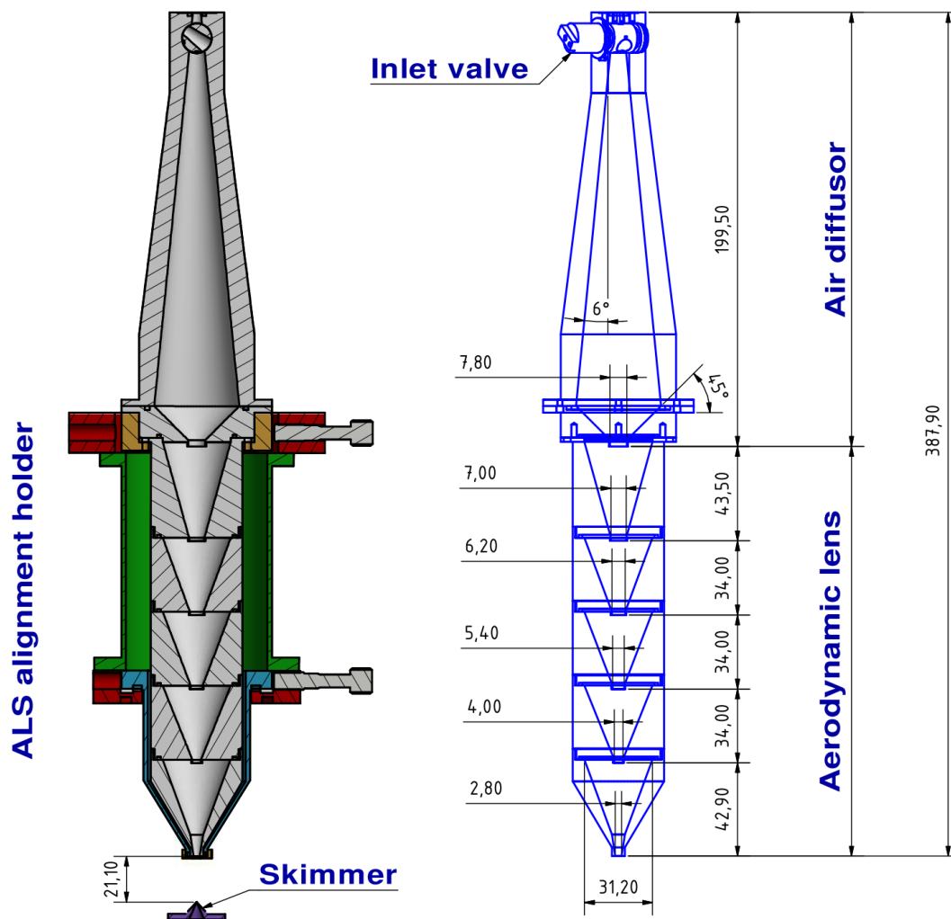
Figure 3. Schematic of the new aerodynamic lens, the air diffuser (including a conical shaped valve) and the ALS alignment holder, as well as the corresponding dimensions in millimeters. On the left side, the cross-section of the ALS alignment holder in the xz -plane is presented, which is why only one upper and one lower adjusting screw is shown, whereas the adjusting screws perpendicular to them (in y -direction) are not shown. The two lower screws precision align the pivot point of the ALS (O-ring center close to the lens exit) centrally above the skimmer, the upper screws tilt the ALS around the pivot point, aligning the aerodynamic particle path to the geometrical detection system axis (see also Supplement Sect. 7). The two upper screws have now been replaced by motors (as described in Sect. 3.1.3). A spring mechanism is used for the required restoring force on the opposite side of the adjusting screws/motors.
