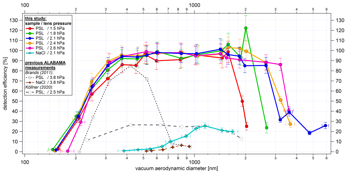
Figure 13. Size-resolved detection efficiency of PSL and NaCl particles. The detection efficiency is related to particles that led to coincidences. The results achieved with the new ALS are shown with solid lines. The colors represent the different lens pressures from 1.5 hPa to 2.6 hPa and the markers distinguish between PSL and NaCl particles. ALABAMA measurements taken with the previously used Liu-type aerodynamic lens (Kamphus et al., 2008) and without the air diffusor are shown as dashed lines. The y-uncertainty bars refer to the uncertainties of the components used (see Supplement Sect. 15.1 and 15.2) and the x-uncertainty bars correspond to the standard deviation of the particle size distribution per particle size, particle type and lens pressure measured with ALABAMA, converted into d_{va} according to Eq. S1 (Supplement).
