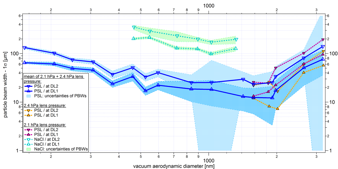
Figure 14. Size-resolved particle beam widths (PBWs) at the two detection stages (DL1 and DL2) for PSL and NaCl particles. Below 1600 nm, the beam widths are averaged for 2.1 hPa and 2.4 hPa lens pressure (PSL only). The PBWs are given as 1\sigma as defined in Eq. 4. The y-uncertainty range is given by the uncertainty of the fit of each scan (see Sect. 4.2.2). The x-uncertainty bars correspond to the standard deviation of the particle size distribution per particle size, particle type and lens pressure measured with ALABAMA, converted into d_{va} according to Eq. S1 (Supplement).
