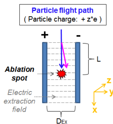
Figure 5. Schematical illustration of charge-dependent particle deflections using a constant electric ion extraction field within the mass spectrometer. The blue arrow shows the particle flight path that is not influenced by the electric field, while the pink arrow indicates the charge-dependent deflection.
