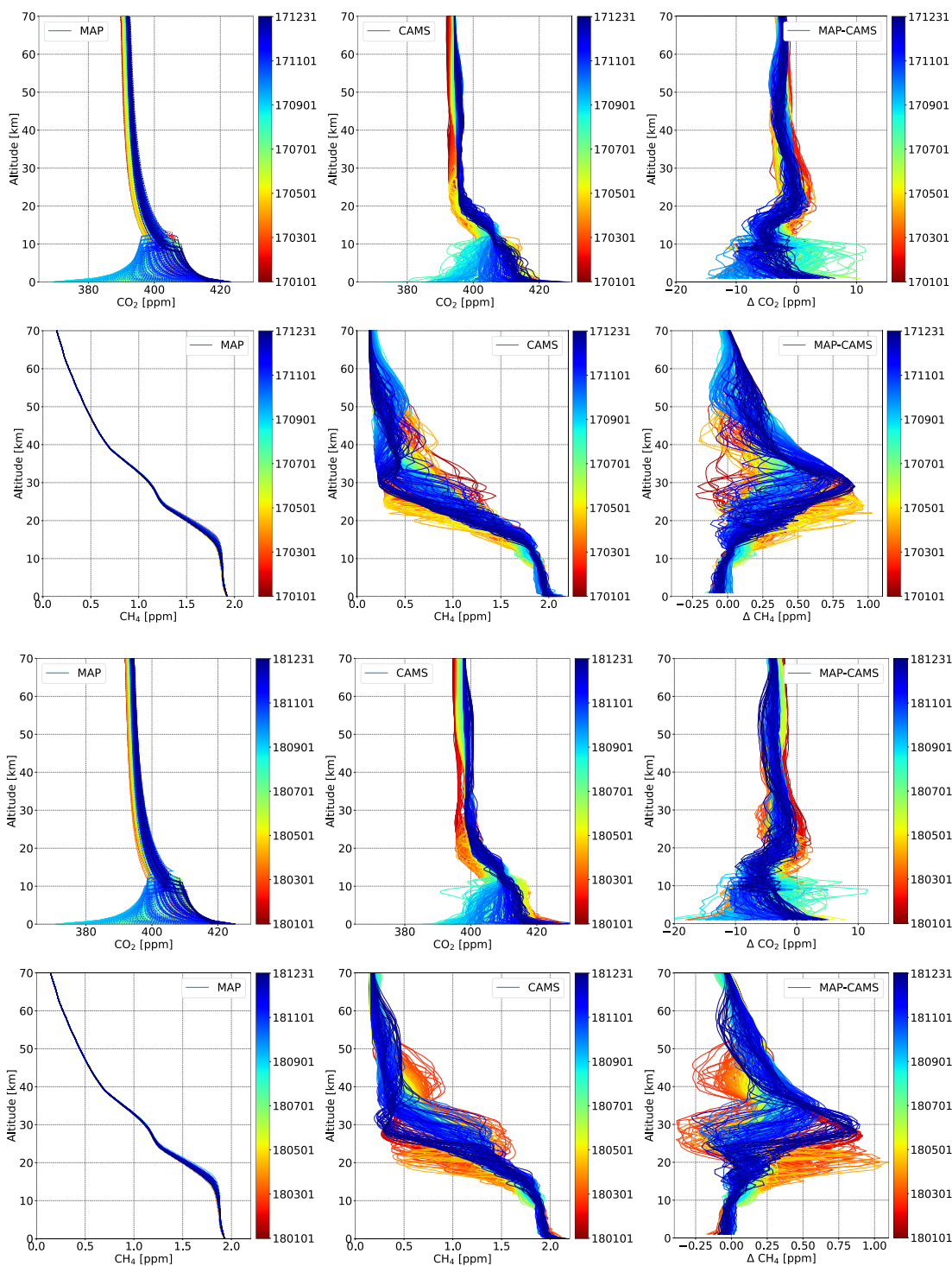
Figure 2. Profiles of MAP (left columns), CAMS (middle columns) and the difference of MAP-CAMS (right columns) for CO 2 and CH 4 in 2017 and 2018.
