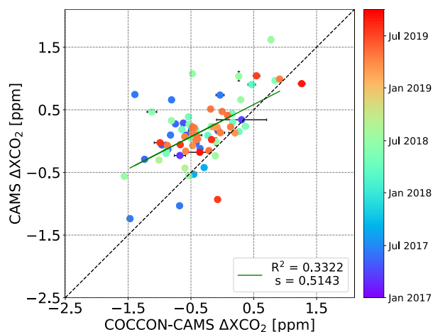
Figure 11. Difference of XCO_2 measured between Kiruna and Sodankylä. Plot showing the comparison between CAMS and COCCON. The annotations follow those in Figure 5.
