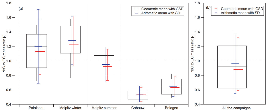
Figure S2: Statistics (10 th , 25 th , 50 th , 75 th and 90 th percentiles, arithmetic and geometric means, SD and GSD) of the rBC to EC mass ratio ( m_{rBC}/m_{EC} ) per campaign (panel a) and with all the campaigns of this work (panel b).
