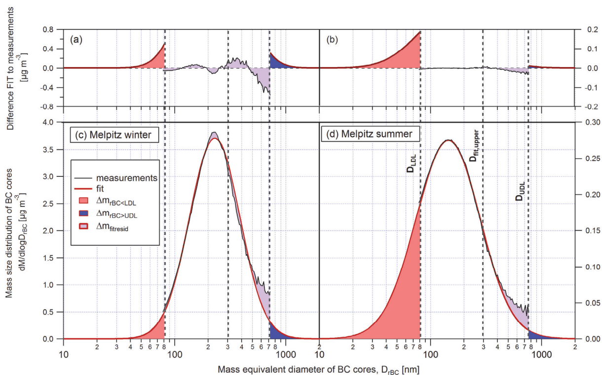
1280 Figure 1: Approach to correct for the rBC mass outside the rBC core size range covered by the SP2 for the Melpitz 1285 winter (panels a and c) and the Melpitz summer (panels b and d) campaigns. The bottom two panels show the measured rBC mass size distribution as a function of rBC core mass equivalent diameter, including the SP2 detection limits D_{LDL} and D_{UDL} . The lognormal functions are fitted between D_{LDL} and D_{fit,upper} . The integrated area of the red, purple, and blue shadings correspond to \Delta m_{rBC < LDL} , \Delta m_{fitresid} and \Delta m_{rBC > UDL} , respectively (see Sect. 2.3.5). The top two panels additionally show the same shadings after subtraction of the measured size distribution (and measurement forced to be zero outside the SP2 detection range). The average mass size distributions of the other campaigns are represented in Fig. S1.
