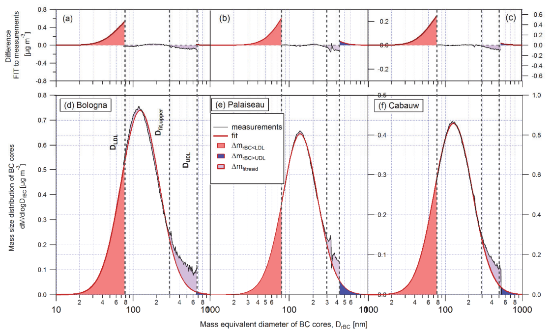
Figure S1: Approach to correct for the rBC mass outside the rBC core size range covered by the SP2 for the Bologna (panels a and d), the Palaiseau-Paris (panels b and e) and the Cabauw (panels c and f) campaigns. The bottom three panels show the measured rBC mass size distribution as a function of rBC core mass equivalent diameter, including the SP2 detection limits D_{LDL} and D_{UDL} . The lognormal functions are fitted between D_{LDL} and D_{fit,upper} . The integrated area of the red, purple, and blue shadings correspond to \Delta m_{rBC < LDL} , \Delta m_{fitresid} and \Delta m_{rBC > UDL} , respectively (see Sect. 2.3.5). The top three panels additionally show the same shadings after subtraction of the measured size distribution (and measurement forced to be zero outside the SP2 detection range).
