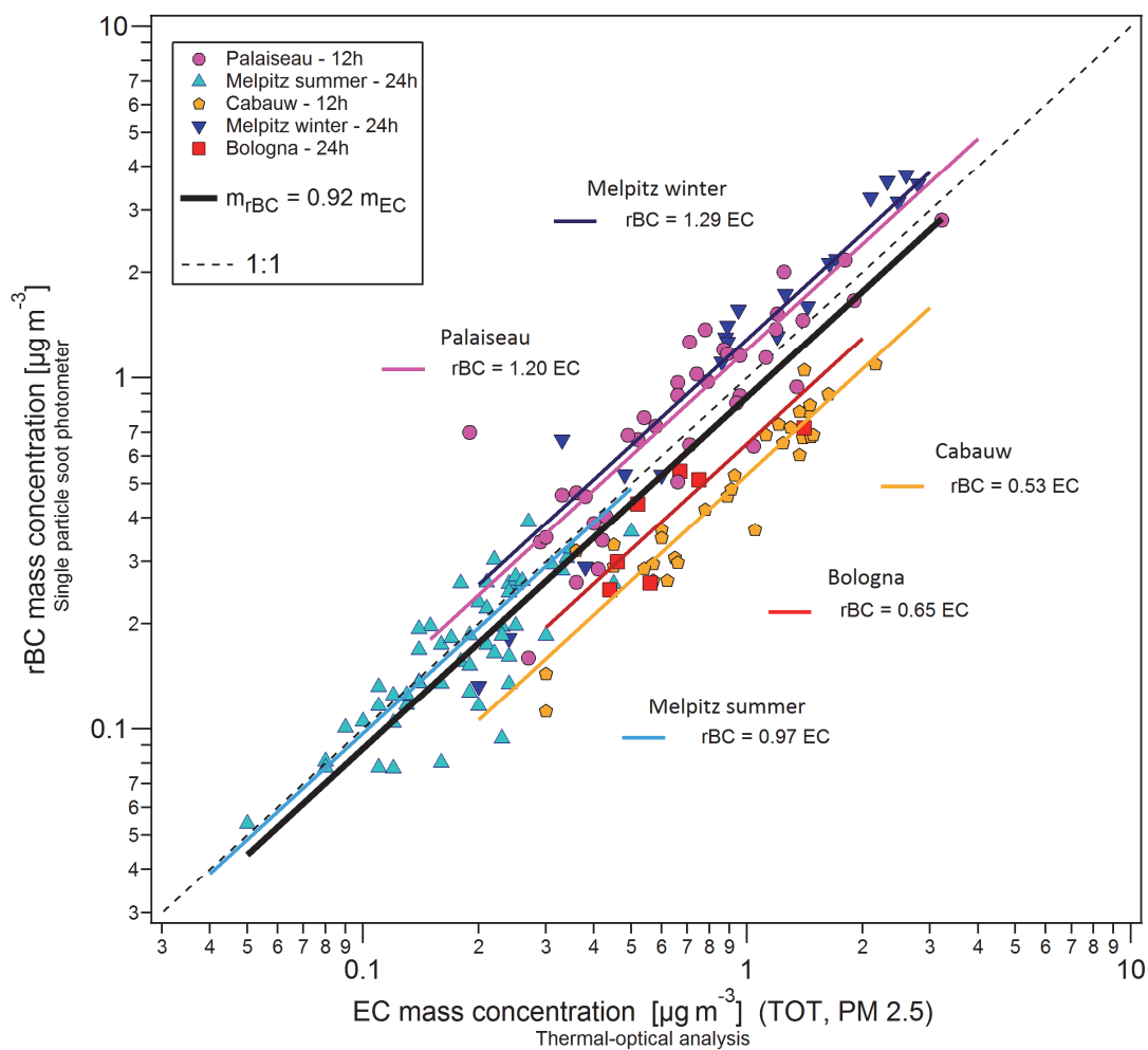
1305 Figure 3: rBC mass concentration versus EC mass concentration for the five campaigns studied in this paper. The median rBC to EC mass ratios are shown as lines for each campaign. Uncertainties of EC measurements as a function of EC and TC filter surface loadings as well as EC/TC mass ratio are presented in Fig. S3 and discussed in Sect. 3.3.2.
