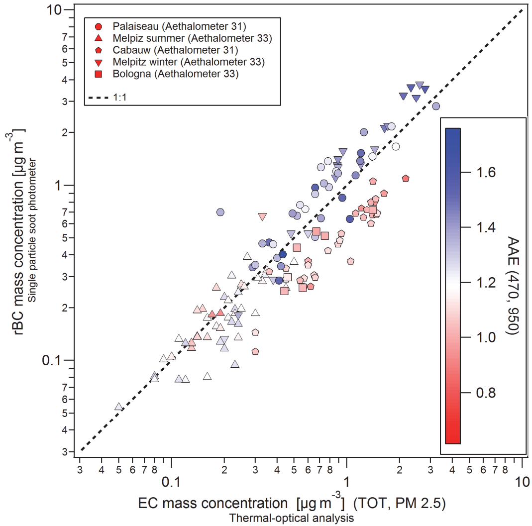
1320 Figure 5: rBC mass concentration versus EC mass concentration for all campaigns of this study color-coded by the Ångström absorption exponent of each data point.
