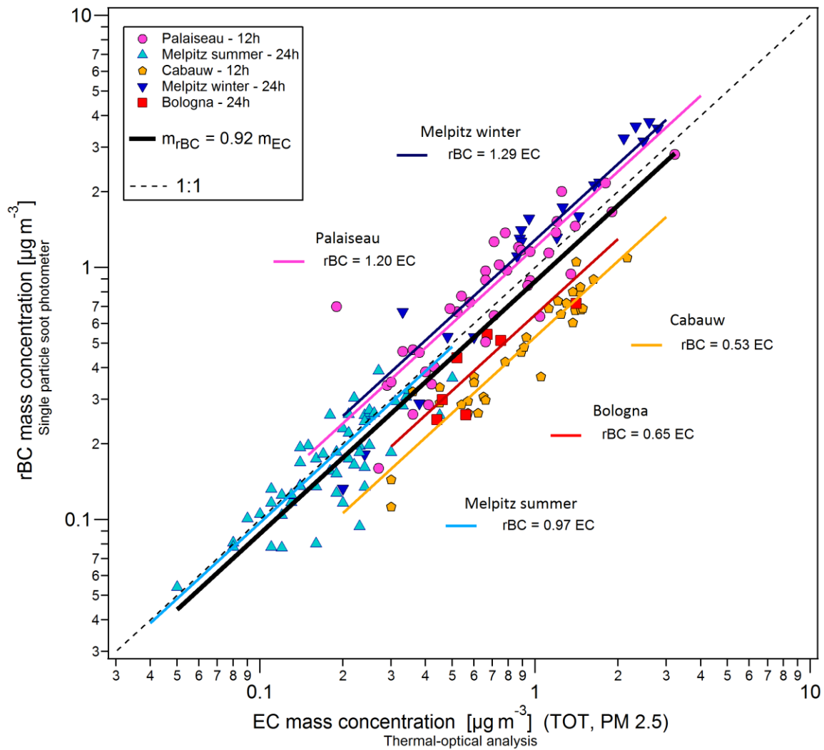
1255 Figure 3: rBC mass concentration versus EC mass concentration for the five campaigns studied in this paper. The median rBC to EC mass ratios are shown as lines for each campaign. Uncertainties of EC measurements as a function of EC and TC filter surface loadings as well as EC/TC mass ratio are presented in Fig. S3 and discussed in Sect. 3.3.2.
