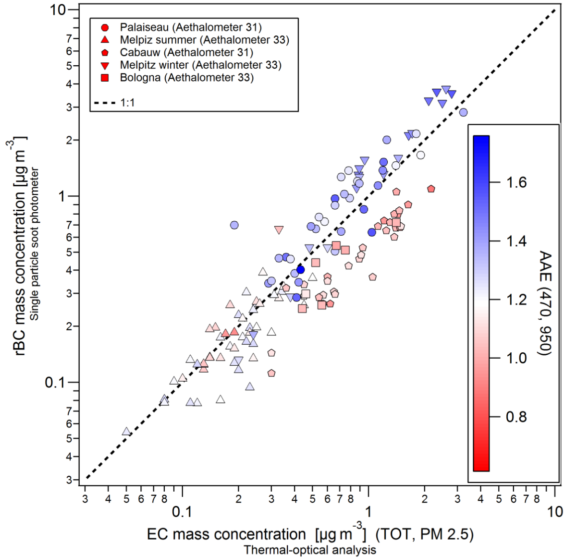
1270 Figure 5: rBC mass concentration versus EC mass concentration for all campaigns of this study color-coded by the Ångström absorption exponent of each data point.
