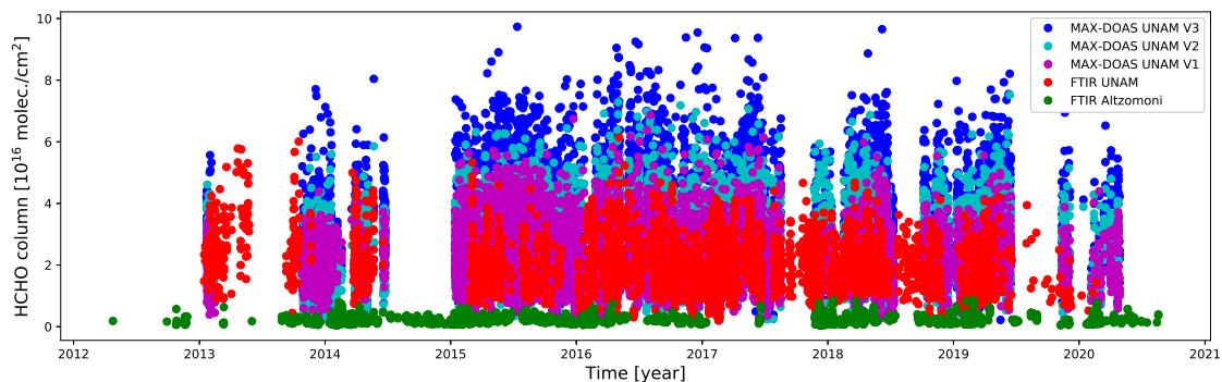
Figure 1. Hourly means of HCHO vertical column densities (VCDs) from the MAX-DOAS instrument at UNAM ( V1 (magenta), V2 (cyan), V3 (blue)), solar absorption FTIR instrument at UNAM (red) and at Altzomoni (green). The measurements in Mexico City at the UNAM-campus (red, magenta, cyan & blue) are one order of magnitude higher than the background measurements at the mountain site Altzomoni (green). The same applies to their variance. The difference between the MAX-DOAS and FTIR measurements at UNAM is mainly explained by their averaging kernel and is discussed in detail in the text. The altitude ranges covered by each instrument are FTIR UNAM VCDs 2-16 km, FTIR Altzomoni VCDs 4-16 km and MAX-DOAS UNAM VCDs 2-5 km.
