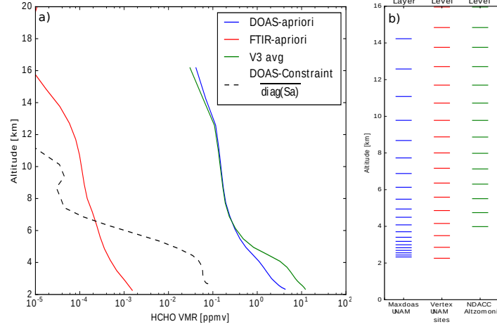
Figure 6. a) A priori information for the MAX-DOAS and FTIR retrievals. The blue line is the a priori used in the MAX-DOAS retrieval, the black dashed line shows the square root of the Sa -matrix in the MAX-DOAS retrieval regularized according to optimal estimation (OE). As commonly used for FTIR retrievals that form part of the NDACC network, an a priori taken from the WACCAM model was used. The green line is the average of the MAX-DOAS retrieved HCHO profiles (V3, both sides) and gives an idea about the vertical distribution of HCHO above UNAM. This averaged profile is used as common a priori for the improved intercomparison between MAX-DOAS and FTIR; b) Vertical grids of the MAX-DOAS and FTIR (both measurement sites) inversions.
