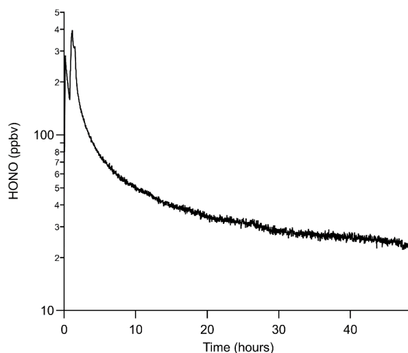
Figure 6. Mixing ratio of HONO produced from a \text{NaNO}_2 coated annular denuder using PD-6c. Time zero is when HCl was first introduced to the annular denuder at 50 % RH. Note that HONO mixing ratios are on a log scale.
