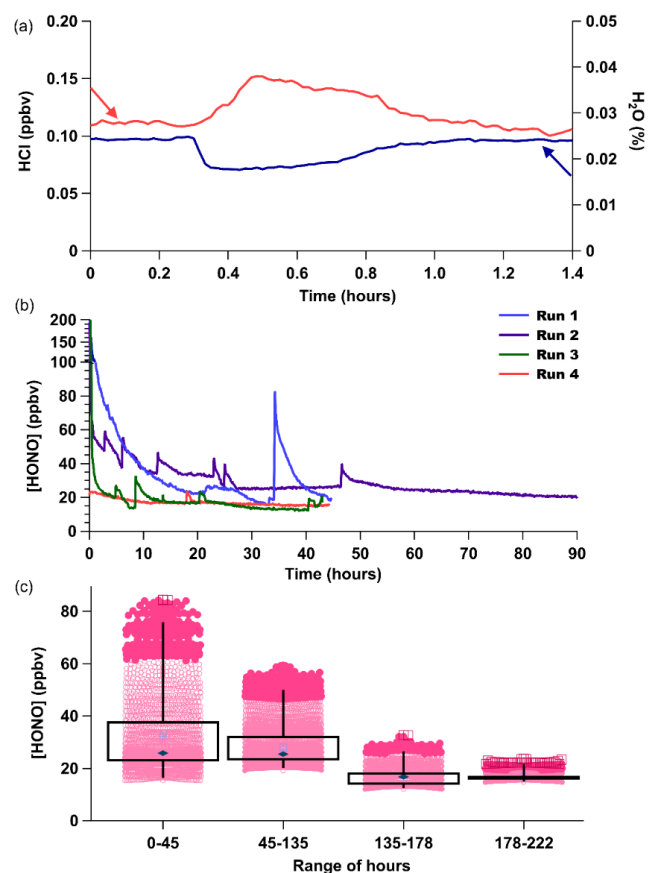
485 Figure 4. (a) CRDS high-resolution observation an HCl emission pulse (red) and H 2 O decrease (blue) from PD-6a resulting in 50 % increase of the HCl mixing ratio emitted. (b) Time series of four consecutive measurement periods of HONO production, using only PD-6c and a new NaNO 2 coated reaction device in each run. (c) Box (1 st and 3 rd quartile) and whiskers (3σ from the mean) of HONO mixing ratios observed for the four runs are binned by duration of use for each new reaction device in hours. Mean values are indicated with a filled dark blue diamond marker, median values by the light blue crossed box marker, dark pink circles are 2σ outliers and dark red squares 3σ outliers 490
