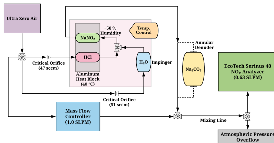
Figure 1. Flow and component schematic of the HONO calibration system (pink shaded region) interfaced with a NO x analyzer (green), dilution mass flow controller (blue), and an exchangeable Na 2 CO 3 annular denuder (yellow). Lines with black arrows denote the direction of gas flow through system components. Tee and cross fittings are denoted by arrays of grey triangles.
