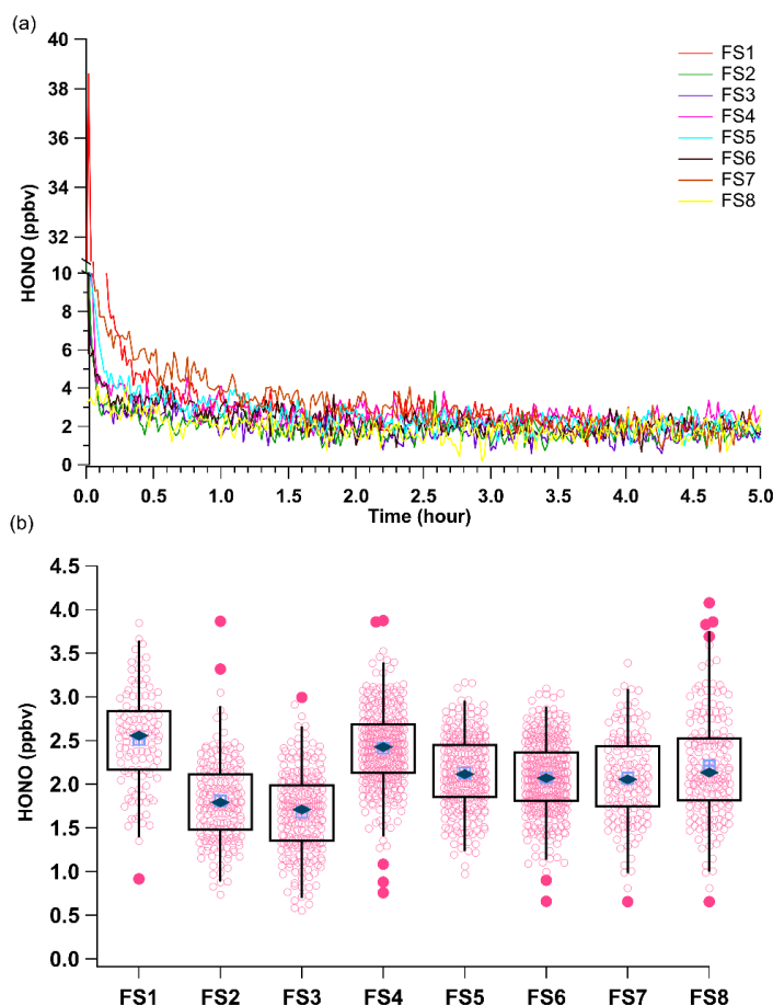
Figure 5. (a) Mixing ratios of HONO for the eight field transport simulations (FS, Table S1). All observations were background corrected by linear interpolation across the experiments using zero air before and after HONO observations and an \text{Na}_2\text{CO}_3 coated annular during (Fig. S4). (b) Box and whiskers plot of the HONO output using measurements collected after two hours of calibration source stabilization. The light blue crossed box represents the median, the dark blue diamond the mean, light pink circles the data points, dark pink circles the 3\sigma outliers, and the black box the 1 st and 3 rd quartiles of observed HONO mixing ratios. The whiskers denote the 3\sigma standard deviation.
