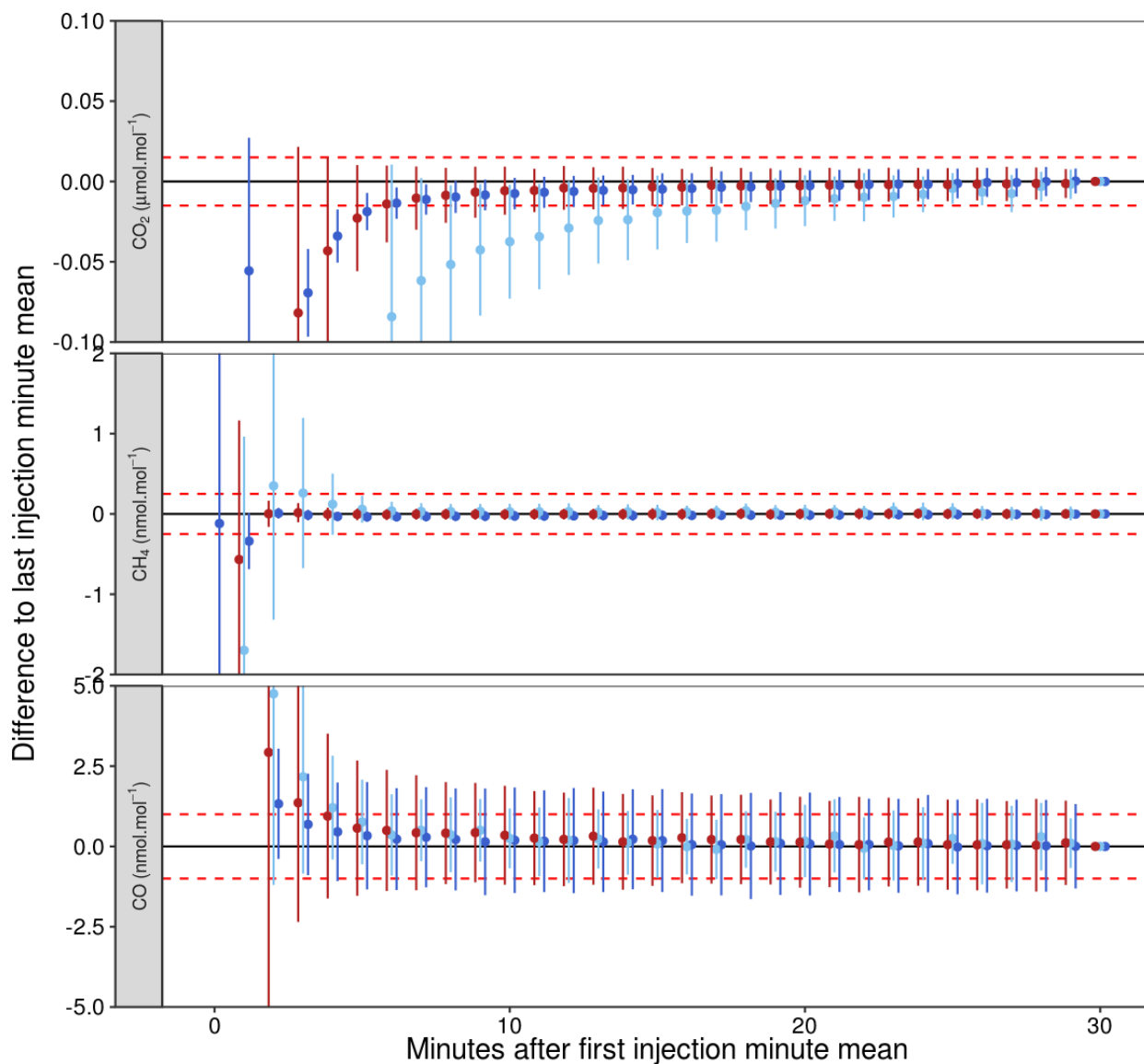
Figure 5. Difference between the last injection minute averaged data point and the rest of the injection for cylinder samples for Monte Cimone station (CMN) for instrument 590. All the injections over the last six months are averaged. Short-term target is in dark blue, long-term target in light blue and calibration in red. Red dashed lines show the thresholds. Vertical lines on each point show the minute standard deviation.
