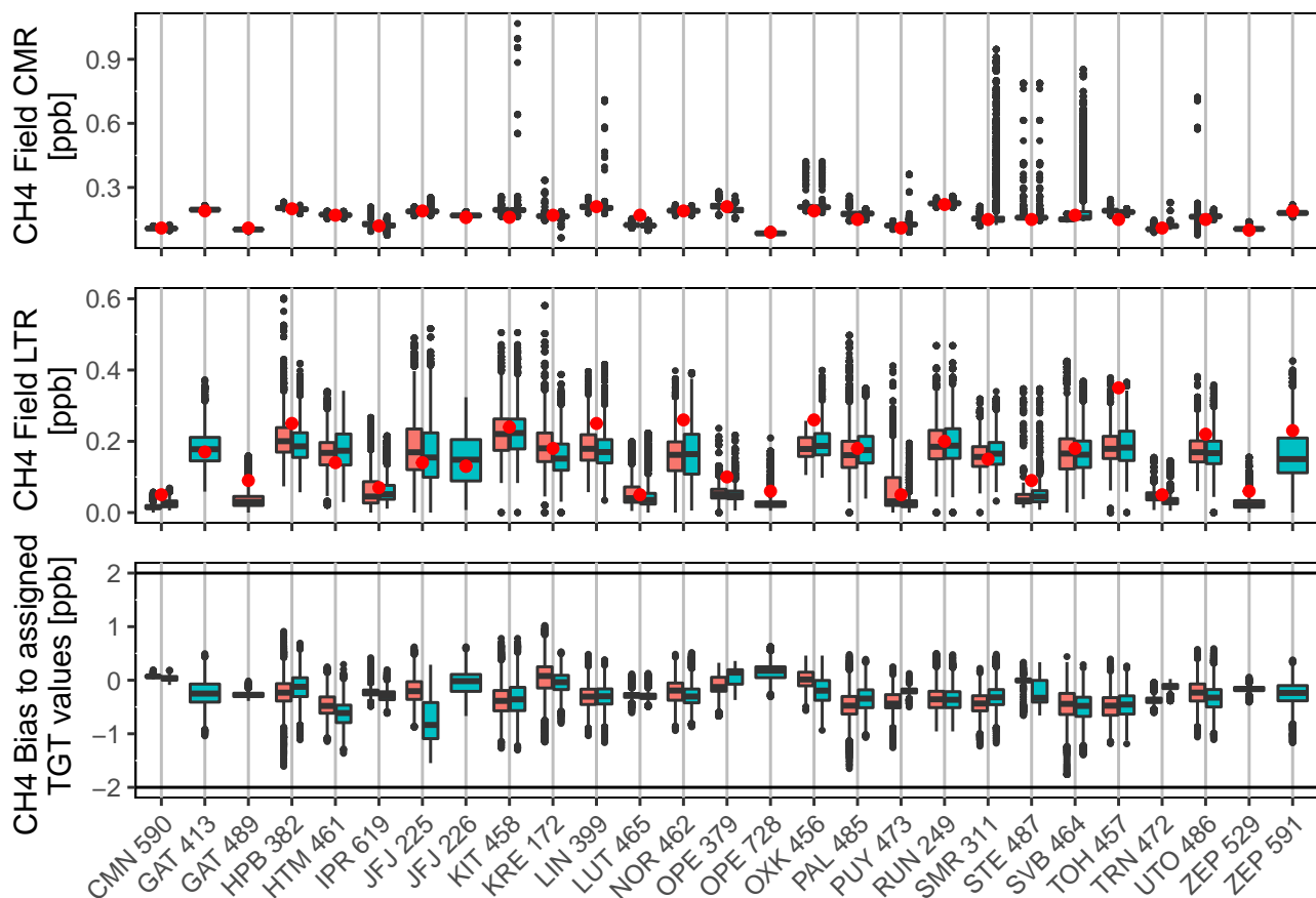
Figure 17. Uncertainties and bias to the short-term target for CH 4 defined as in Figure 13. The red dot shows the minute CMR and LTR from the MLab initial tests. The left box (pink) is calculated using data from the year prior to labeling. The right box (blue) is calculated using data from March 2019 to March 2020. For Gat, 489 was prior to 413. For JFJ, 226 has replaced 225. At OPE, 729 is running in parallel with 379. At ZEP, 529 was prior to 591. The x-axis shows the site trigram and ICOS ID of the analyzer. The black lines in the bias plot show the WMO compatibility goals.
