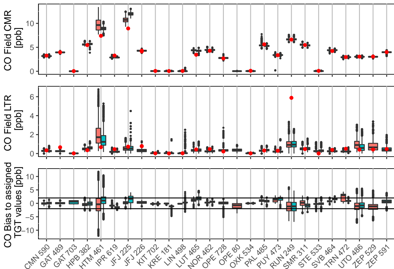
Figure 18. Uncertainties and bias to the short-term target for CO defined as in Figure 13. The red dot shows the minute CMR and LTR from the MLab initial tests. The left box (pink) is calculated using data from the year prior to labeling. The right box (blue) is calculated using data from March 2019 to March 2020. For Gat, 489 was prior to 413. For JFJ, 226 has replaced 225. At OPE, 729 is running in parallel with 379. At ZEP, 529 was prior to 591. The x-axis shows the site trigram and ICOS ID of the analyzer. The black lines in the bias plot show the WMO compatibility goals.
