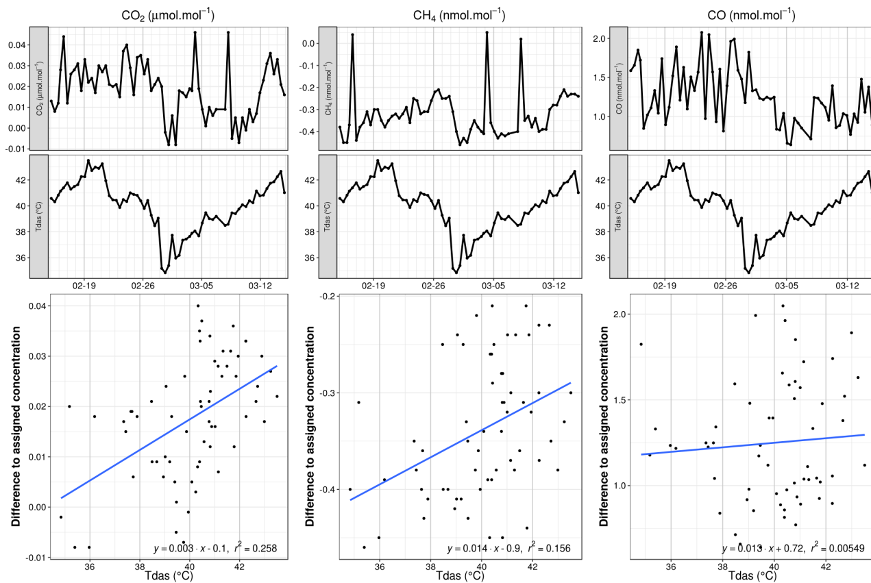
Figure 8. Temperature influence on the measurements at Puy de Dôme station (PUY) for the instrument 473 and the target cylinder D337581. On top, greenhouse gas and instrument temperature (T das ) measurements against time. On the bottom, greenhouse gas measurements against instrument temperature. In most of the cases, no dependencies are seen.
