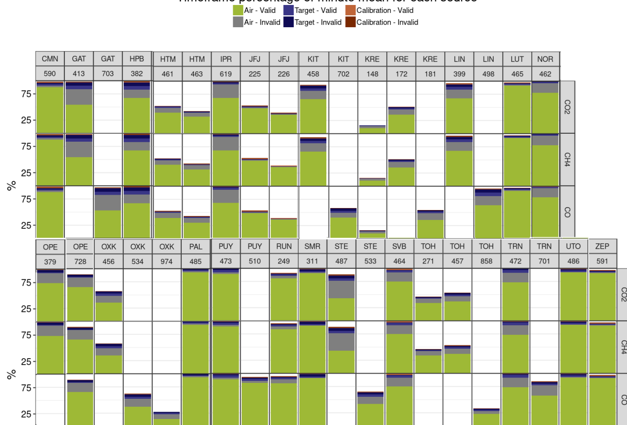
Figure 14. Data distribution between ambient air, target and calibration gases for the 23 stations for CO 2 , CH 4 and CO over the past year. Calibration is in red, target in blue and air in green/gray. Gray and darker color are invalid data. 100% is reached when data are available for the full year. For some stations, two instruments are used to measure CO 2 , CH 4 and CO (see their ICOS ID on the second line). For other, due to instrumental failure, a new instrument has replaced the previous one. See Table 3 for the acronyms and more details about each station.
