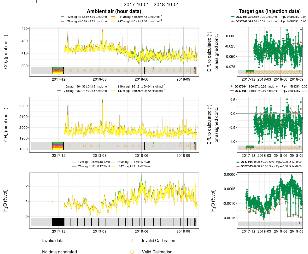
Figure 11. One year of hourly averaged greenhouse gas measurements at Torfhaus station (TOH) for instrument 457. The different levels and targets are plotted with different colors. Ambient air is plotted on the left, target measurements on the right. Calibration are shown with orange open circles. Invalid data are shown at the bottom of each plot. Cylinder number (D*****), mean values ( \pm X ), point-to-point variability (Ptp) and difference to the assigned value (Diff) are displayed above the target gas plots. Measured GHG are shown on the different panels from top to bottom.
