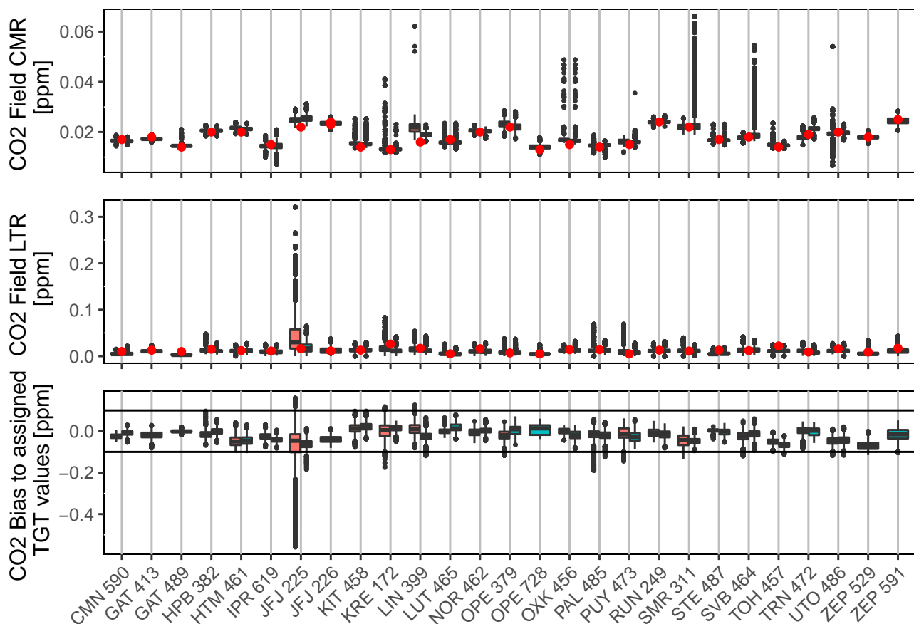
Figure 16. Uncertainties and bias to the short-term target for CO 2 defined as in Figure 13. The red dot shows the minute CMR and LTR from the MLab initial tests. The left box (pink) is calculated using data from the year prior to labeling. The right box (blue) is calculated using data from March 2019 to March 2020. For Gat, 489 was prior to 413. For JFJ, 226 has replaced 225. At OPE, 729 is running in parallel with 379. At ZEP, 529 was prior to 591. The x-axis shows the site trigram and ICOS ID of the analyzer. The black lines in the bias plot show the WMO compatibility goals.
