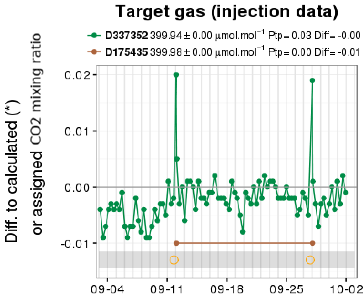
Figure 1. One month of target gas injections for CO 2 (ppm or \mu\text{mol.mol}^{-1} ), shown as the difference of calculated vs. assigned mixing ratios. Short term target is plotted in green, whilst long term data are in brown. The calibration dates are shown by the light orange open circles. Cylinder number (D*****), mean values ( \pm X ), point-to-point variability ( P_{tp} ) and difference to the assigned value ( \text{Diff} ) are displayed above the figure.
