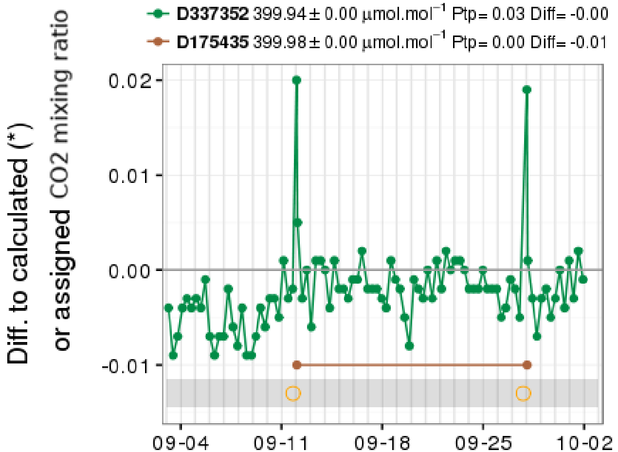
Figure 1. One month of target gas injections for CO 2 (ppm or \mu\text{mol.mol}^{-1} ), shown as the difference of calculated vs. assigned mixing ratios. Short term target is plotted in green, whilst long term data are in brown. The calibration dates are shown by the light orange open circles. Cylinder number (D*****), mean values ( \pm X ), point-to-point variability (Ptp) and difference to the assigned value (Diff) are displayed above the figure.
