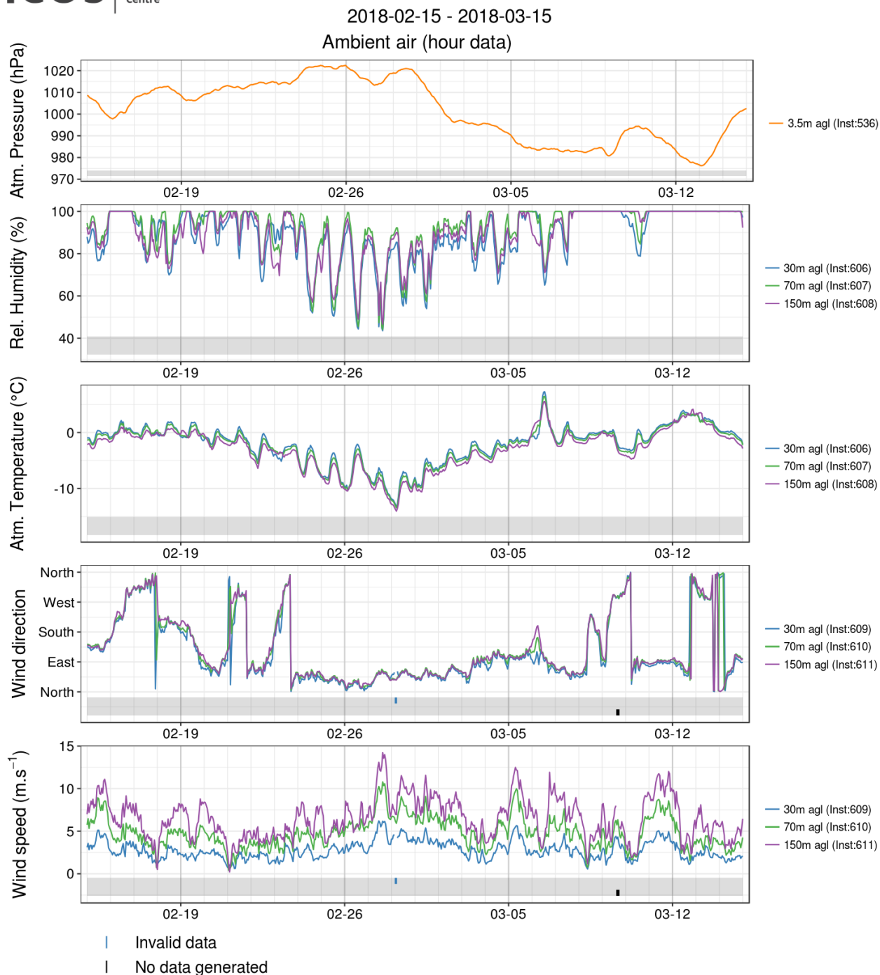
Figure 9. One month of meteorological parameters at Hyltemossa station (HTM). From top to bottom: atmospheric pressure, relative humidity, atmospheric temperature, wind direction and wind speed. The data at the different levels are plotted with different colors.
