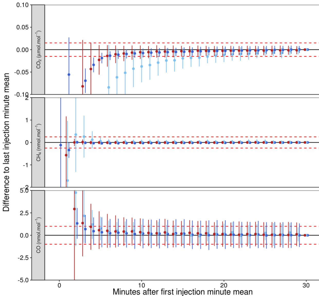
Figure 5. Difference between the last injection minute averaged data point and the rest of the injection for cylinder samples for Monte Cimone station (CMN) for instrument 590. All the injections over the last six months are averaged. Short-term target is in dark blue, long-term target in light blue and calibration in red. Red dashed lines show the thresholds. Vertical lines on each point show the minute standard deviation.
