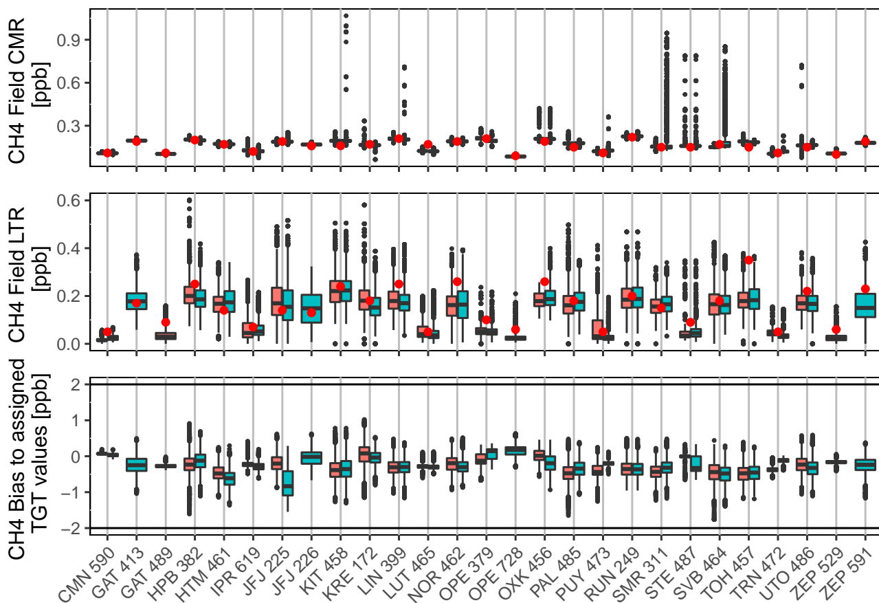
Figure 17. Uncertainties and bias to the short-term target for CH 4 defined as in Figure 12. The red dot shows the minute CMR and LTR from the MLab initial tests. The left box (pink) is calculated using data from the year prior to labeling. The right box (blue) is calculated using data from March 2019 to March 2020. For Gat, 489 was prior to 413. For JFJ, 226 has replaced 225. At OPE, 729 is running in parallel with 379. At ZEP, 529 was prior to 591. The x-axis shows the site trigram and ICOS ID of the analyzer. The black lines in the bias plot show the WMO compatibility goals.
