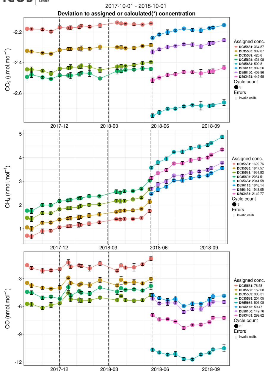
Figure 6. Evolution of the analyzer raw output when measuring different calibration gases with respect to the assigned values over a year at Trainou station (TRN) for instrument 472. Each calibration cylinder is shown with a different color. Assigned values are indicated on the right for each cylinder (D*****).
