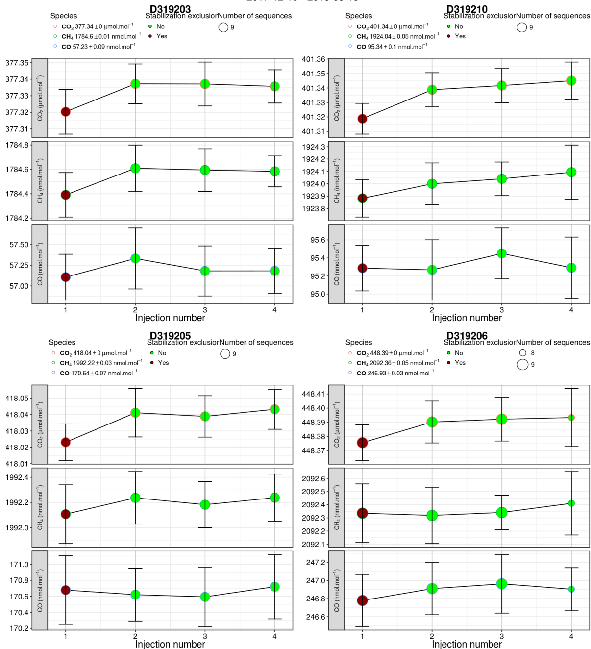
Figure 7. Average of each cycle injection for the last calibrations over three months at Svartberget station (SVB) for instrument 464. Green dots are data used for the calibration correction, red is rejected for stabilization. The number of calibrations is shown of the top right. Assigned values are on the top left. Cylinder number (D***** ) is shown at the top of each panel.
