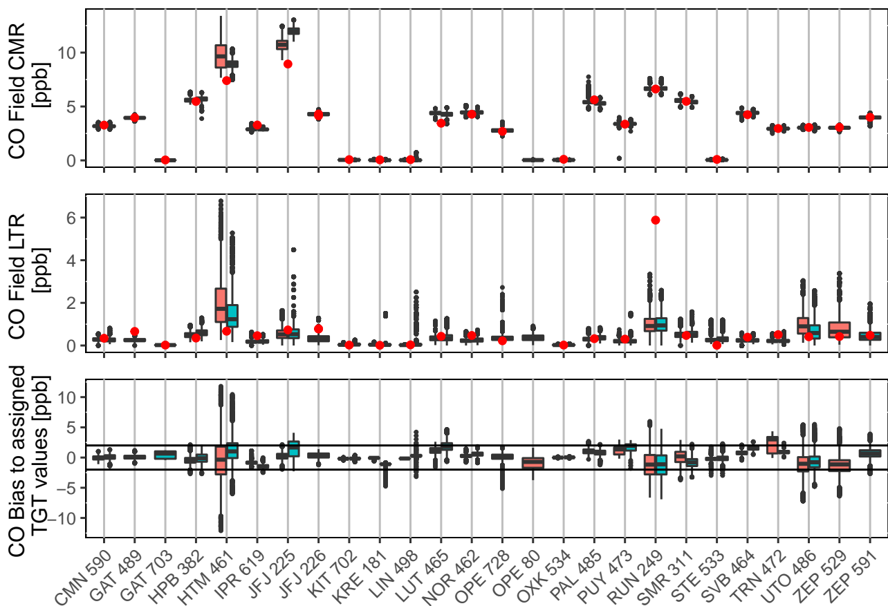
Figure 18. Uncertainties and bias to the short-term target for CO defined as in Figure 12. The red dot shows the minute CMR and LTR from the MLab initial tests. The left box (pink) is calculated using data from the year prior to labeling. The right box (blue) is calculated using data from March 2019 to March 2020. For Gat, 489 was prior to 413. For JFJ, 226 has replaced 225. At OPE, 729 is running in parallel with 379. At ZEP, 529 was prior to 591. The x-axis shows the site trigram and ICOS ID of the analyzer. The black lines in the bias plot show the WMO compatibility goals.
