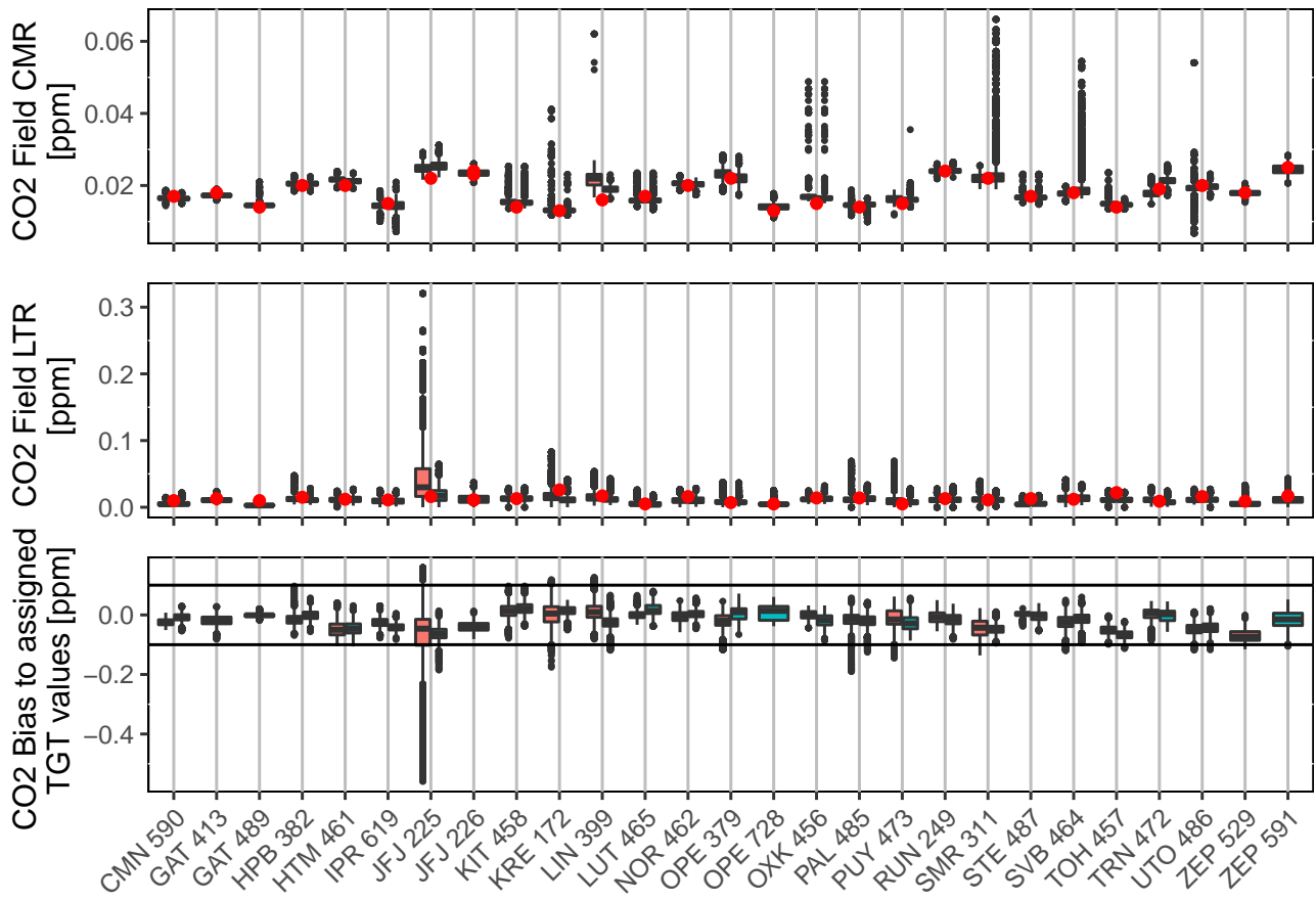
Figure 16. Uncertainties and bias to the short-term target for CO 2 defined as in Figure 12. The red dot shows the minute CMR and LTR from the MLab initial tests. The left box (pink) is calculated using data from the year prior to labeling. The right box (blue) is calculated using data from March 2019 to March 2020. For Gat, 489 was prior to 413. For JFJ, 226 has replaced 225. At OPE, 729 is running in parallel with 379. At ZEP, 529 was prior to 591. The x-axis shows the site trigram and ICOS ID of the analyzer. The black lines in the bias plot show the WMO compatibility goals.
