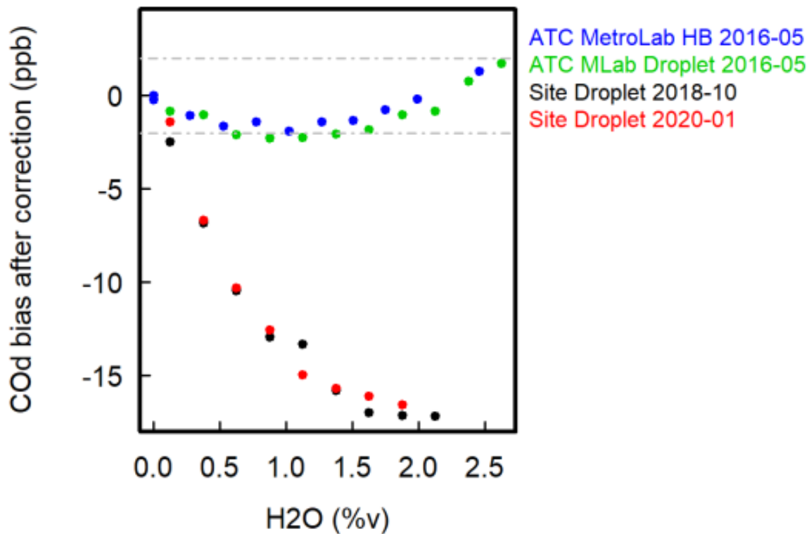
Figure 20. Example of water vapor correction assessment over time for CO. HB stands for humidity bench while Droplet is for the droplet test described in the text. The humidity bench allows a much more controlled and precise sensitivity test. The two sites droplets show a large drift of the water vapor correction compared to the initial tests.
