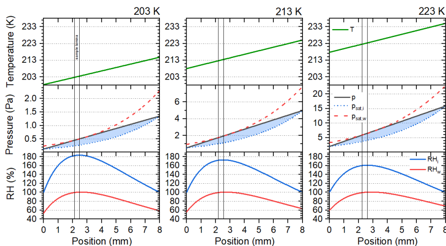
Figure 1. Linear temperature (top row) and vapour pressure (second row) gradients between the wall plates of SPIN at 203 K, 213 K, 223 K lamina temperature and RH_w = 100\% . Vapour pressure ( p ) is compared to saturation pressure over water ( p_{sat,w} ) and ice ( p_{sat,i} ), calculated according to Murphy and Kopp (2005). Ice super-saturated conditions are indicated as shaded areas. The resulting profiles of relative humidity with respect to ice ( RH_i ) and with respect to water ( RH_w ) are given in the third row. Sample position is indicated by vertical lines.
