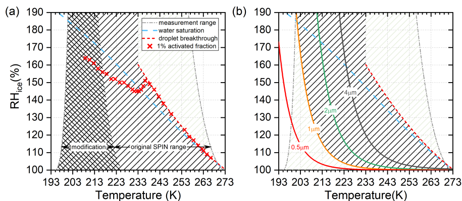
Figure 3. Calculated range of T-,RH i -conditions. (a) Extended limit of experimental capacity with the modified SPIN cooling system (cross-hatched area) compared to the original setup (hatched area). Water saturation is indicated as blue dashed line. Red crosses show 1% activated fractions, measured with 200 nm ammonium sulfate particles (see Fig. 4). Above 235 K the data indicate onset of water breakthrough conditions, below 235 K homogeneous freezing of solution droplets. (b) Limiting conditions to distinguish 0.5 μm, 1 μm, 2 μm and 4 μm (diameter) test particles from growth limited ice crystals. Conditions excluded from ice detection by droplet breakthrough and ice crystal growth are lightly hatched. Total experimental range to measure ice nucleation with the modified SPIN setup is shown as dark hatched area.
