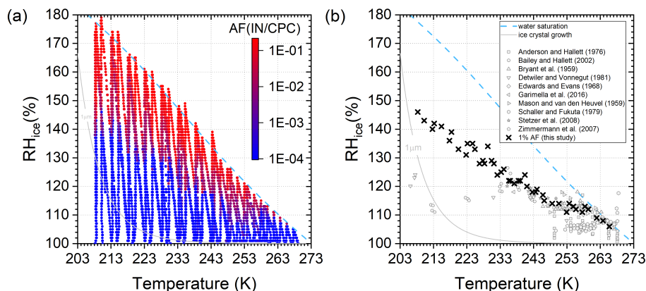
Figure 5. (a) Activated fraction of 200 nm AgI particles, (b) 1% AF in comparison to literature data (references indicated in the figure legend). Water saturation and 1 μm ice crystal growth conditions are indicated as lines.
