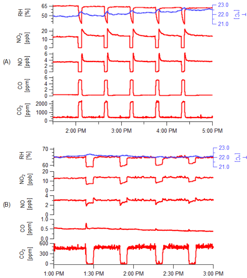
720 Figure 11: Performance of the on-board calibration system over sequential cycles (for demonstration) showing (a) the span gas delivery for CO and CO 2 (and zero air to provide zero concentrations for NO and NO 2 ) over 5 repeated cycles and (b) the zeroing function for CO 2 over 4 cycles where other signals are shown to illustrate minimal changes with zero trap (NO x changes are due to shown RH changes). PM zeroing function results are shown in Fig. S13.
