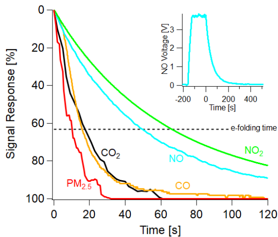
715 Figure 10: Instrument response times shown as the normalized signal response of various sensors in the stationary monitor to a step change in target pollutant concentration and their respective e-folding times. Insert shows a typical step change of calibration gas and the sensor response. Time zero indicates when the multipollutant monitor switched to sampling zero air after reaching a steady state response to the pollutant. Gas sensor response times vary due to the individual sensors' diffusive or electrochemical timescales.
