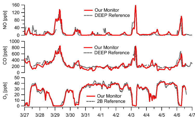
695 Figure 7: Ambient data at 1 h resolution in New Haven, CT near construction shows large NO enhancements. The presence of NO is confirmed by both the titration of O_3 (i.e. NO+O_3 reaction) to zero and large enhancements in CO (a combustion co-pollutant). The near-road DEEP Criscuolo Park site (1.6 km away from sampling location in downtown New Haven) is used for comparison. Note: our NO sensor does not have significant cross-response to O_3 or CO. (See Fig. S11 for additional NO comparisons.) Multipollutant monitor data is corrected for RH/T where appropriate.
