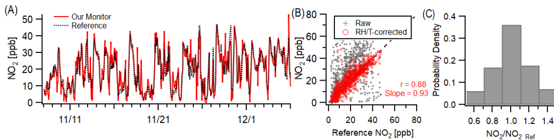
675 Figure 3: Outdoor ambient monitor comparison of NO 2 from Baltimore, MD (Oldtown site). (a) Time series of RH/T-corrected multipollutant monitor data with reference data. (b) With RH/T correction factors the data achieves good correlation. (c) Over 35% of the measurements are within 10% of the reference site.
