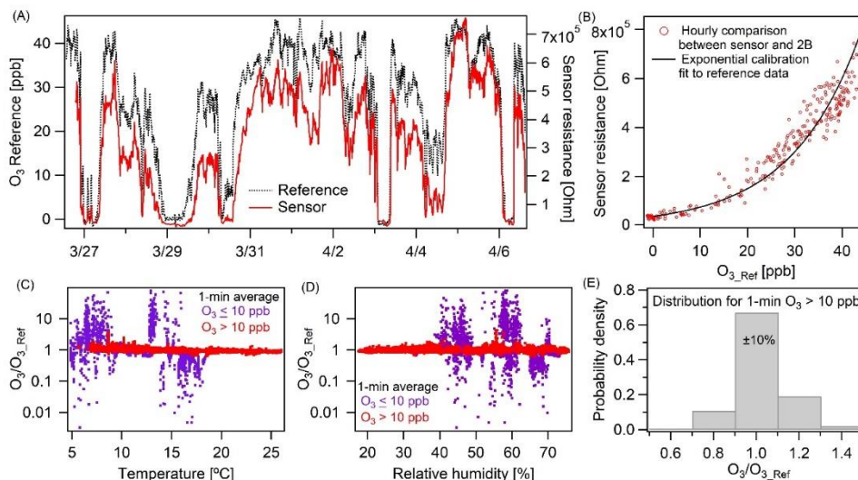
690 Figure 6: Ozone calibration performance and evaluation (a) over 2 weeks in New Haven, CT shown and (b) calibrated against a 2-B Tech reference monitor (note panel A shows sensor resistance, not concentration). (c-d) The ratio of our calibrated vs. reference measurement for concentrations greater and less than 10 ppb over the range of RH and temperatures observed, with no dependence on RH and a slight temperature dependence. (c-d) At concentrations greater than 10 ppb our measurements are much more accurate, (E) with 70% of the 1 min average data falling within \pm 10\% .
